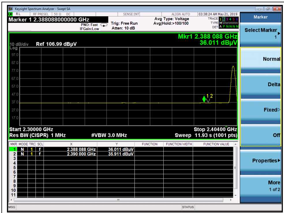
(Channel = 0, AVG)
