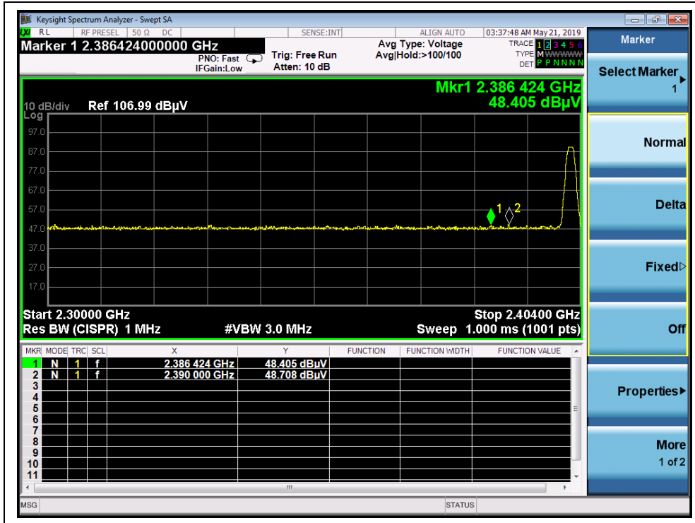
(Channel = 0, PEAK)
