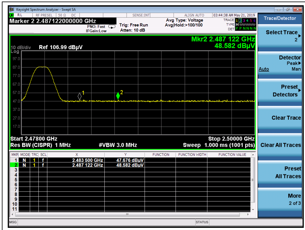
(Channel = 39, PEAK)
