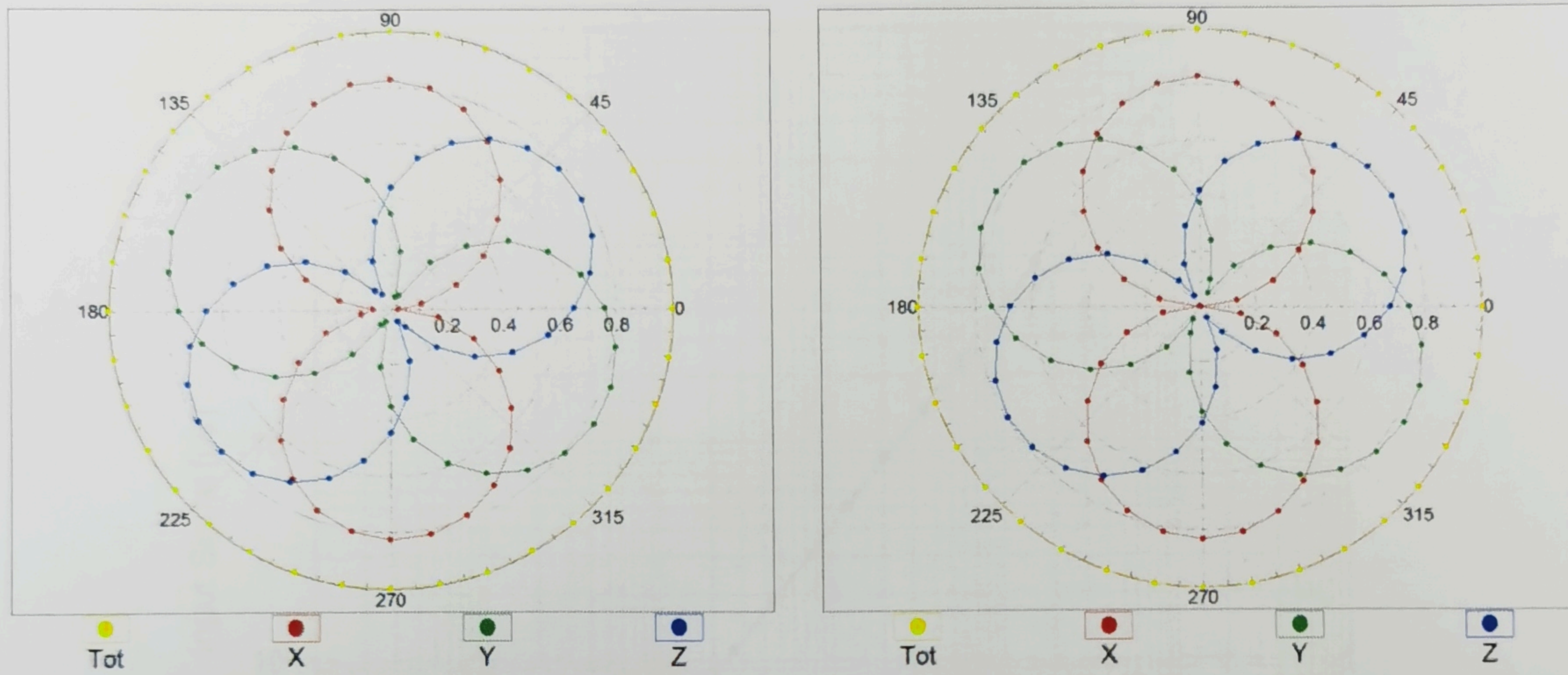
f=600 MHz,TEM
