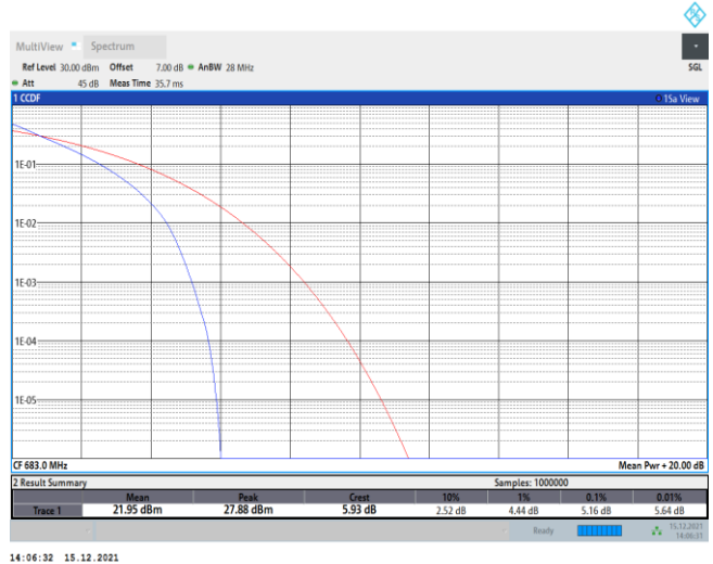
Band71-20MHz-QPSK-133322-100RB#0
