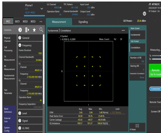
Band41-20MHz-16QAM-40620-100RB#0
