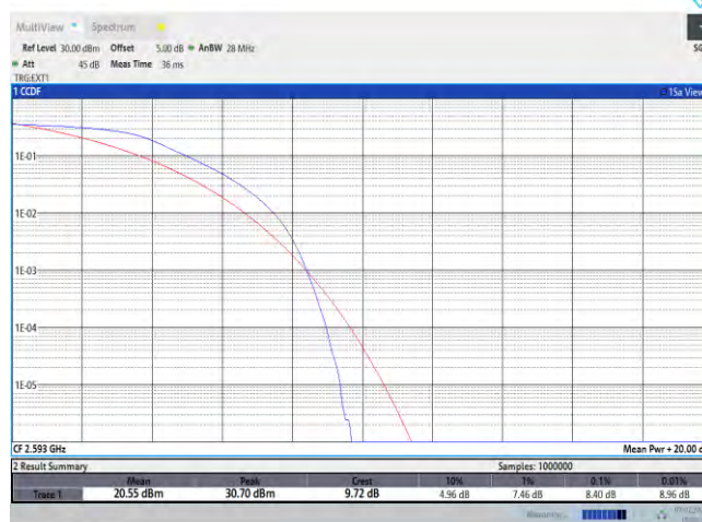
Band41-20MHz-QPSK-40620-100RB#0
