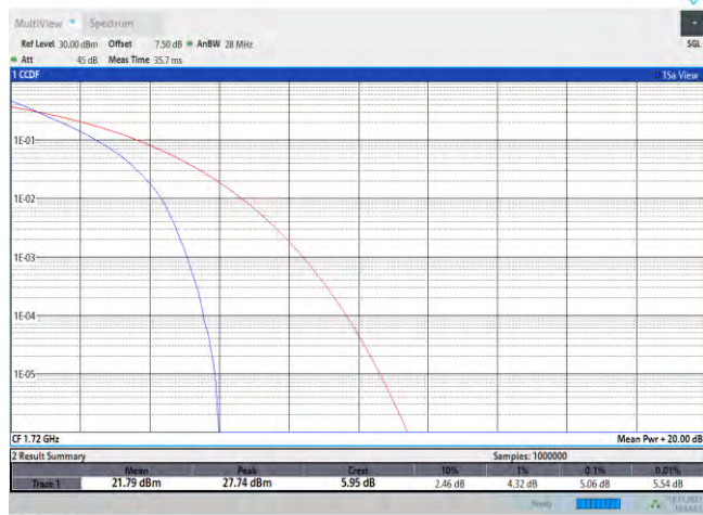
Band66-20MHz-QPSK-132322-100RB#0
