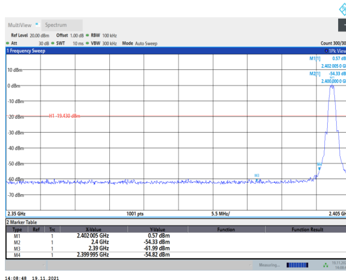
BLE_1M_Ant1_Low_2402
