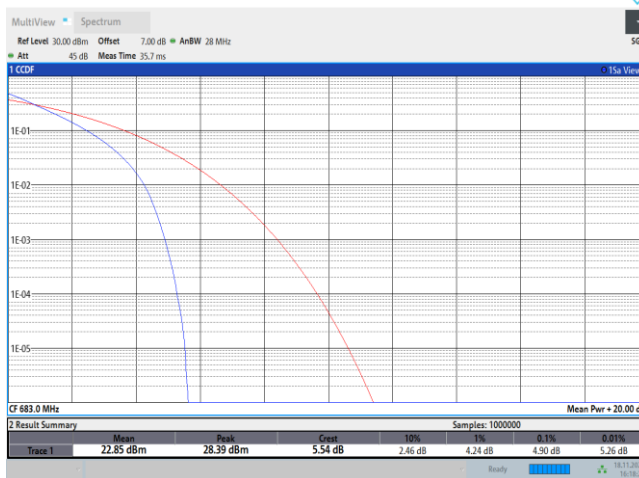
Band71-20MHz-QPSK-133322-100RB#0
