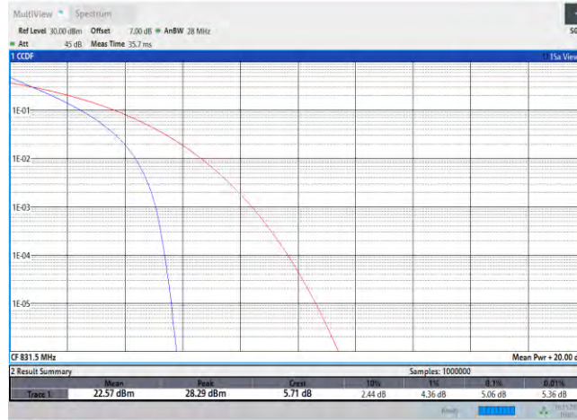
Band26-15MHz-QPSK-26915-75RB#0
