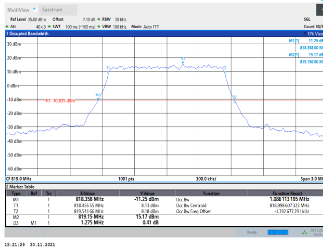
Band26-1.4MHz-QPSK-26740-6RB#0
