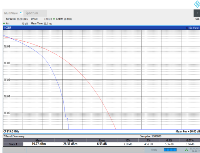
Band26-10MHz-QPSK-26740-50RB#0
