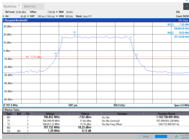
Band12-1.4MHz-QPSK-23095-6RB#0
