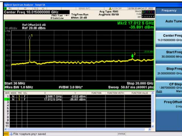
Band41C-30M-20G / 20MHz+20MHz /100RB+100RB/ QPSK / Mid CH
