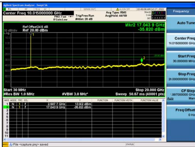
Band41C-30M-20G / 10MHz+20MHz /1RB+1RB/ QPSK / Mid CH
