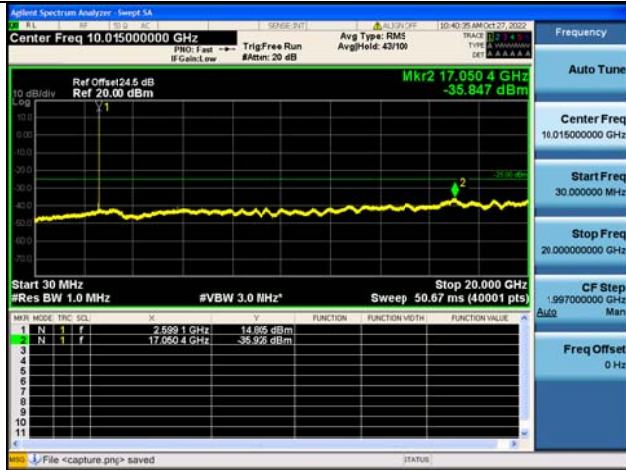
Band41C-30M-20G / 20MHz+5MHz / 1RB+1RB / QPSK / Mid CH
