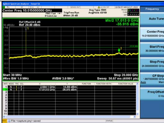
Band41C-30M-20G / 20MHz+15MHz /1RB+1RB/ QPSK / Mid CH
