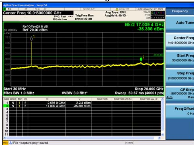
Band41C-30M-20G / 20MHz+5MHz / 100RB+25RB / QPSK / High CH
