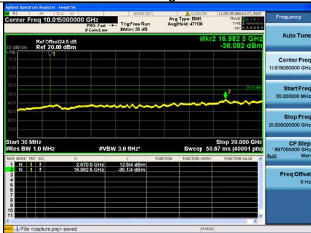
Band41C-30M-20G / 5MHz+20MHz / 1RB+1RB / QPSK / High CH
