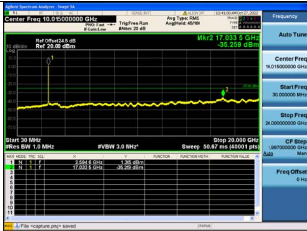
Band41C-30M-20G / 20MHz+5MHz / 100RB+25RB / QPSK / Mid CH
