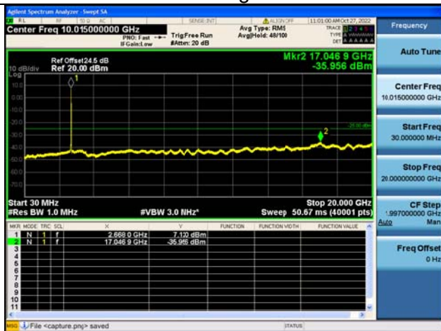
Band41C-30M-20G / 5MHz+20MHz / 25RB+100RB / QPSK / High CH
