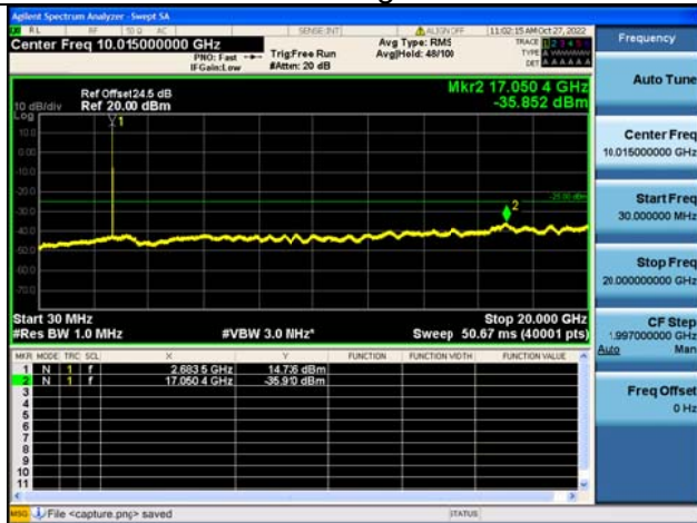
Band41C-30M-20G / 20MHz+5MHz / 1RB+1RB / QPSK / High CH
