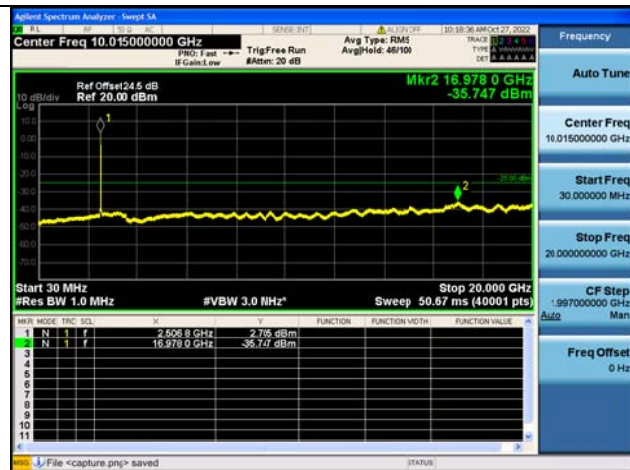
Band41C-30M-20G / 15MHz+20MHz / 75RB+100RB/ QPSK / LOW CH
