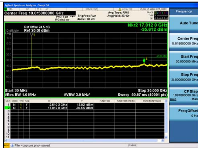
Band41C-30M-20G / 15MHz+20MHz / 1RB+1RB/ QPSK / LOW CH
