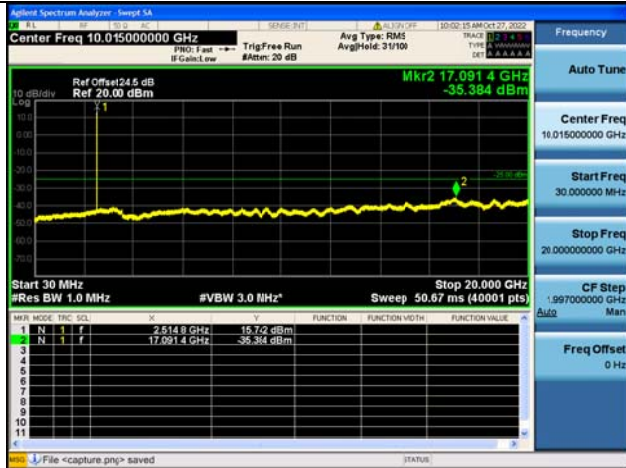
Band41C-30M-20G / 20MHz+5MHz / 1RB+1RB / QPSK / LOW CH
