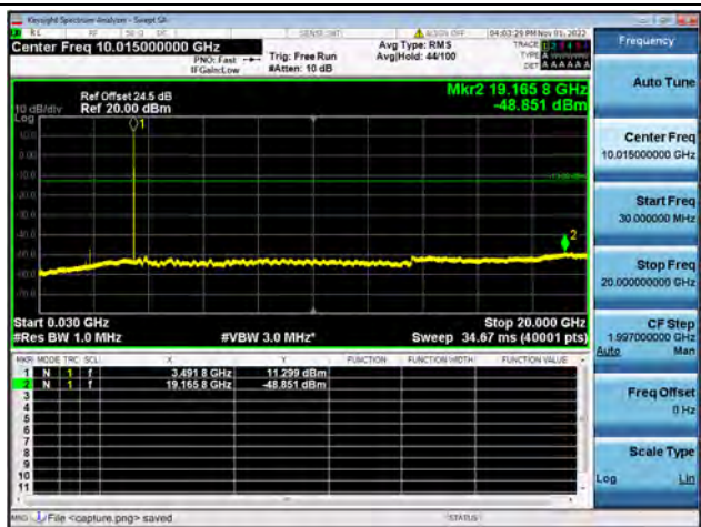
Band42-30M-20G / 20MHz / Mid CH / 64QAM
