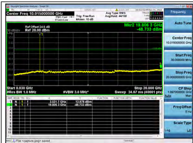
Band42-30M-20G / 20MHz / High CH / QPSK
