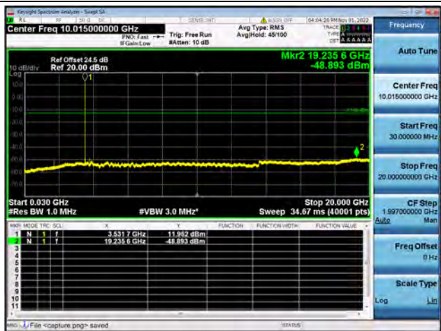
Band42-30M-20G / 20MHz / High CH / 16QAM
