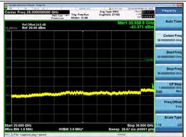
Band42-20G-36G / 20MHz / Low CH / 64QAM
