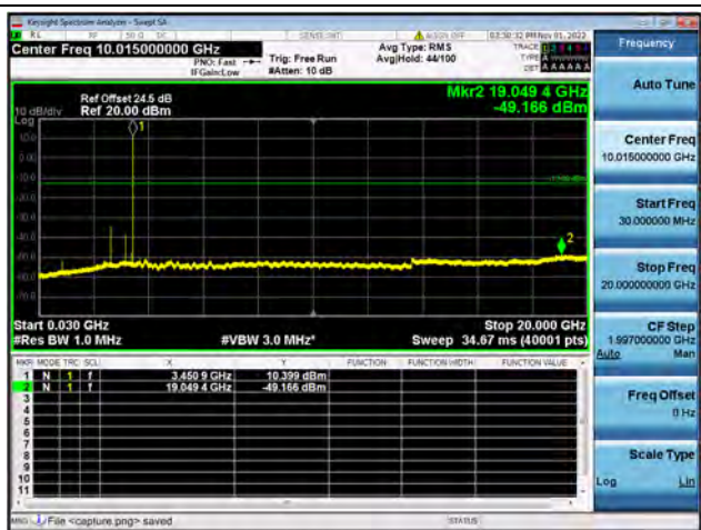
Band42-30M-20G / 5MHz / Low CH / 16QAM
