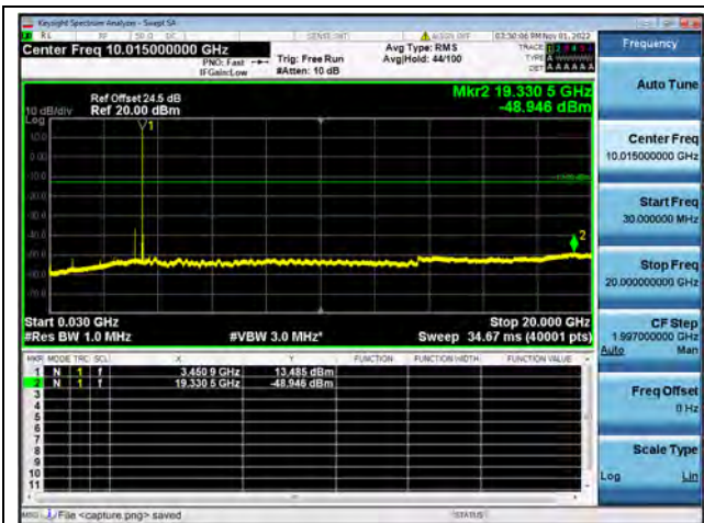
Band42-30M-20G / 5MHz / Low CH / QPSK
