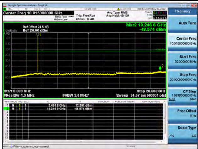
Band42-30M-20G / 20MHz / Mid CH / 16QAM
