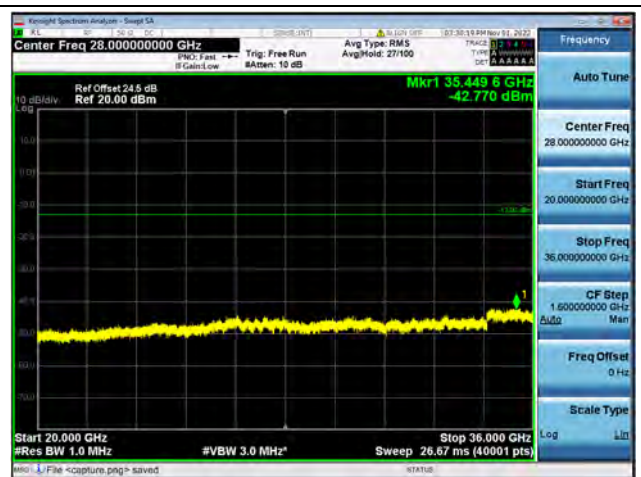
Band42-20G-36G / 5MHz / Low CH / QPSK
