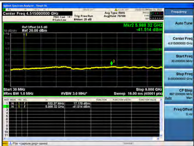
Band26Part22 / 10MHz / Mid CH / 64QAM
