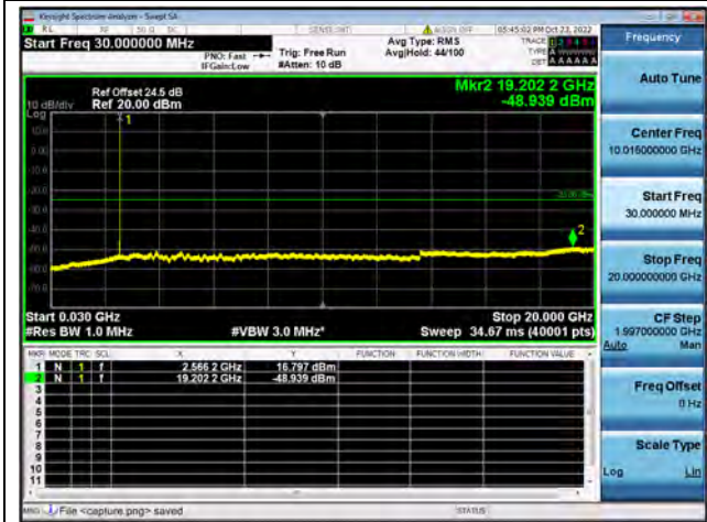
Band7-30M-20G / 5MHz / High CH / 16QAM
