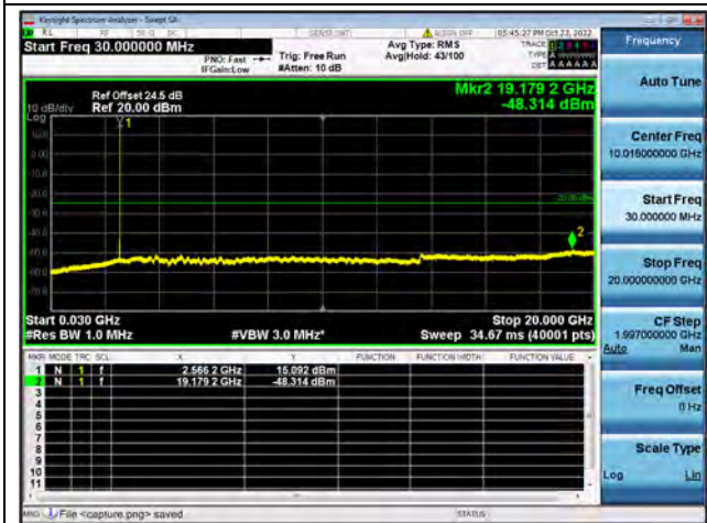
Band7-30M-20G / 5MHz / High CH / 64QAM
