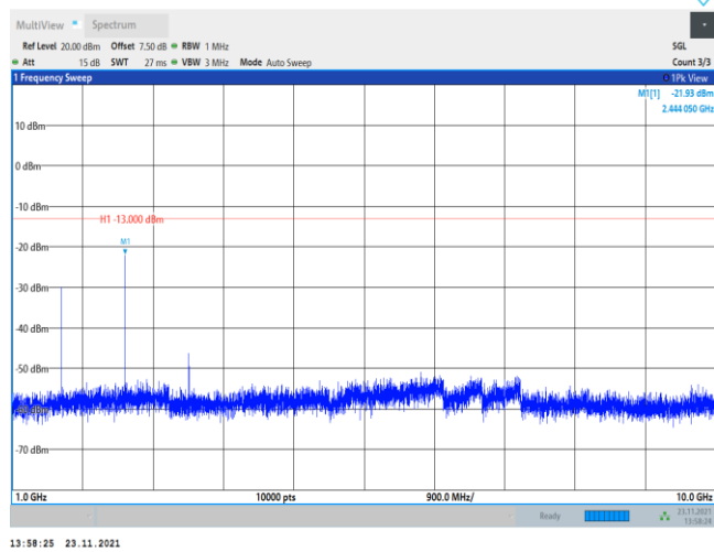
Band26-10MHz-QPSK-26740-1RB#0-Range2:1000~10000MHz
