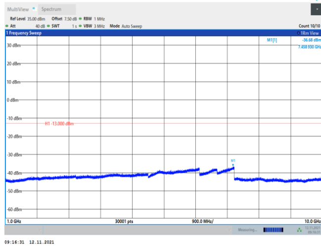
Band12-10MHz-QPSK-23060-1RB#0-Range2:1000~10000MHz
