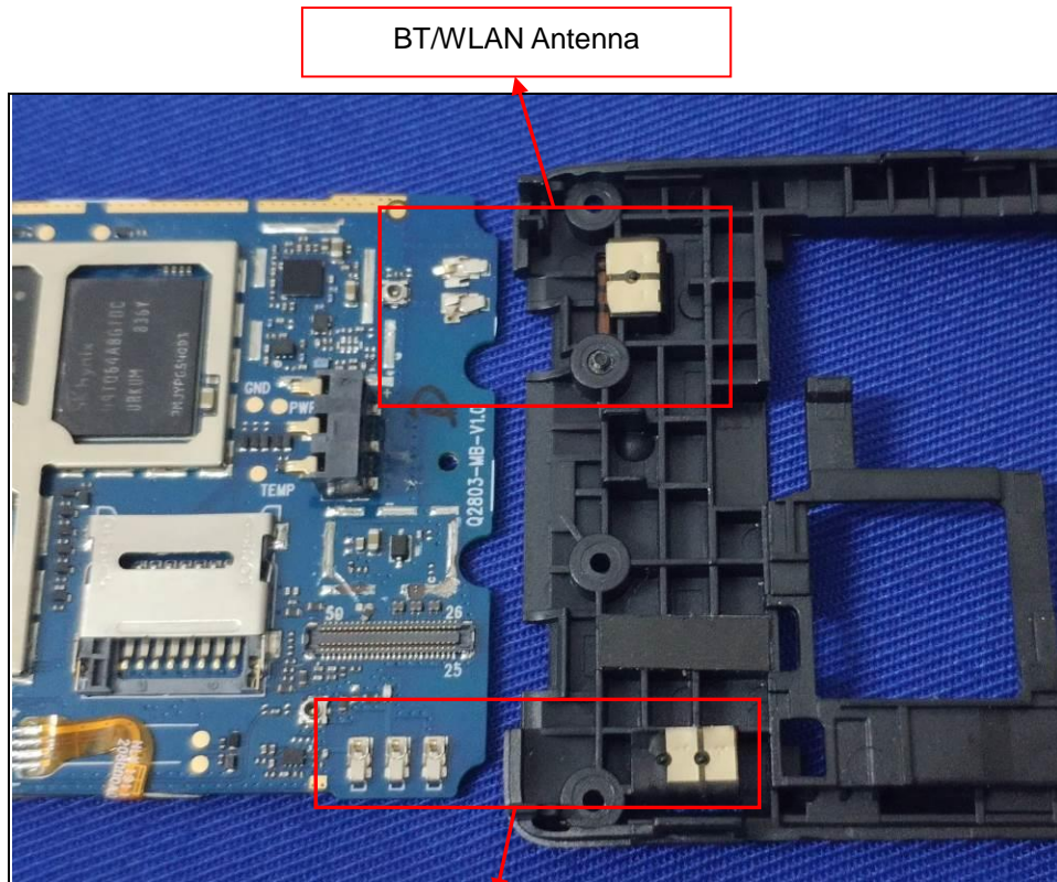
Diversity Antenna
