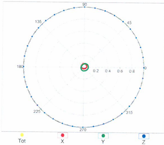
f=600 MHz,TEM,90°
