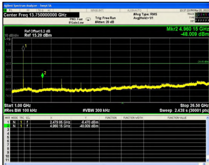
2DH5_Ant1_2480_1000~26500
