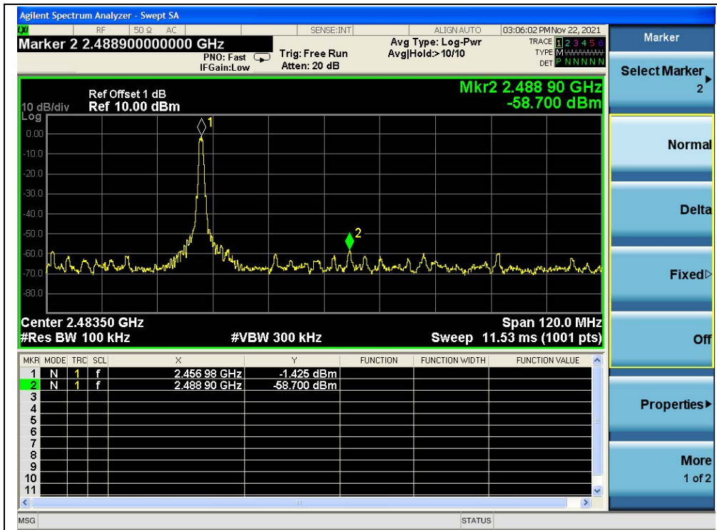
(Band Edge, 2483.5MHz)
