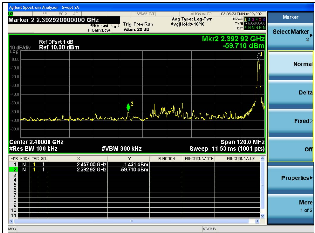
(Band Edge, 2400MHz)
