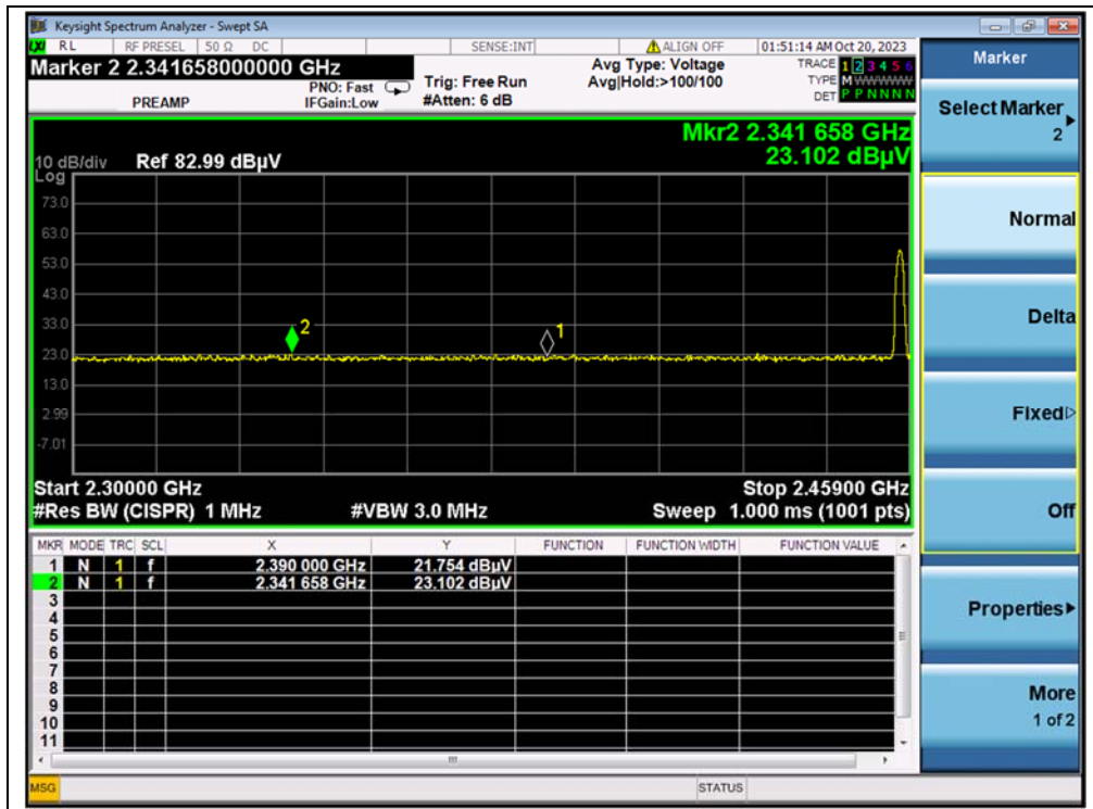
(PEAK, 2457MHz)
