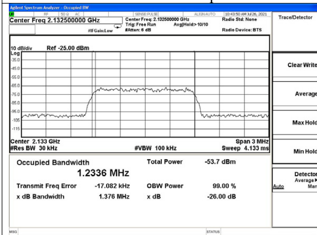
AWS band DL input
