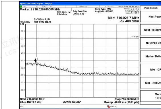
Lower 700MHz band GSM UL Right Side Pre AGC
