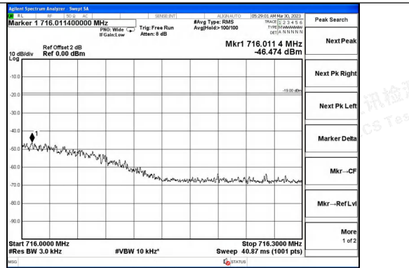
Lower 700MHz band GSM UL Right Side 10dB Above AGC
