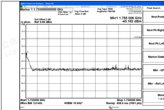
AWS Band GSM UL Right Side Pre AGC
