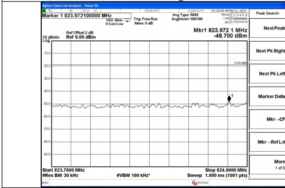
Cellular Band CDMA UL Left Side Pre AGC
