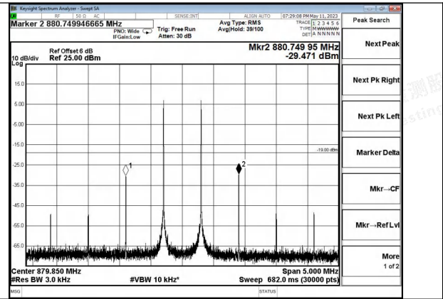
Cellular Band AGC+10dB, DL
