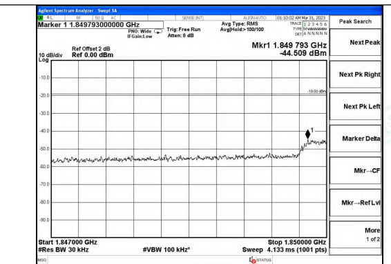
PCS Band CDMA UL Left Side Pre AGC
