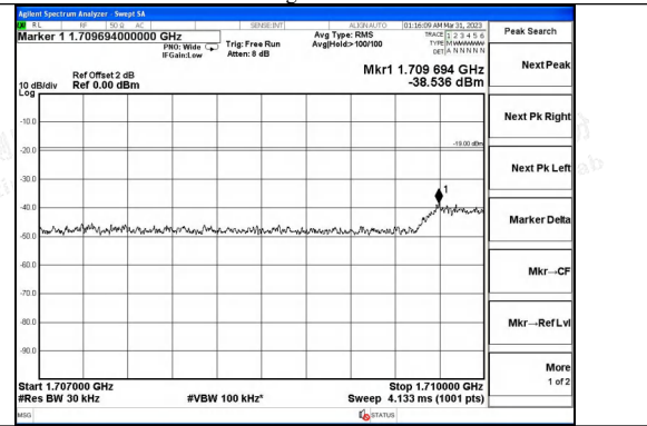
AWS Band CDMA UL Left Side 10dB Above AGC
