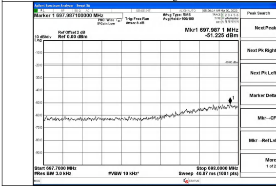
Lower 700MHz band GSM UL Left Side Pre AGC
