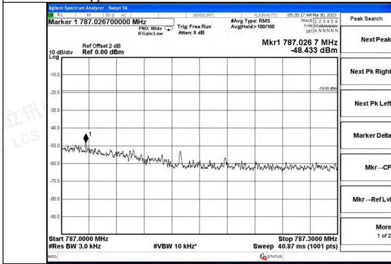
Upper 700MHz band GSM UL Right Side Pre AGC
