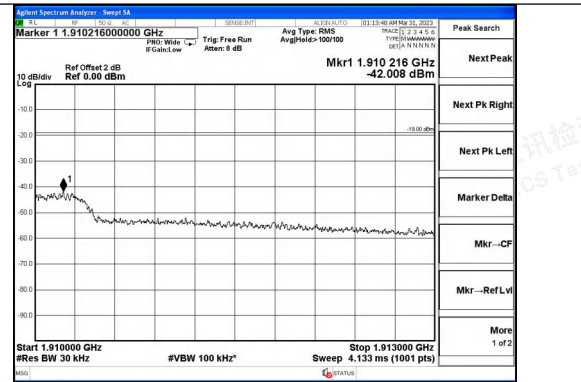
PCS Band CDMA UL Right Side 10dB Above AGC
