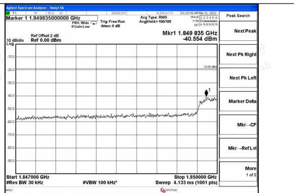
PCS Band CDMA UL Left Side 10dB Above AGC
