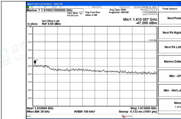
PCS Band CDMA UL Right Side Pre AGC
