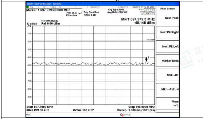
Lower 700MHz band CDMA UL Left Side Pre AGC
