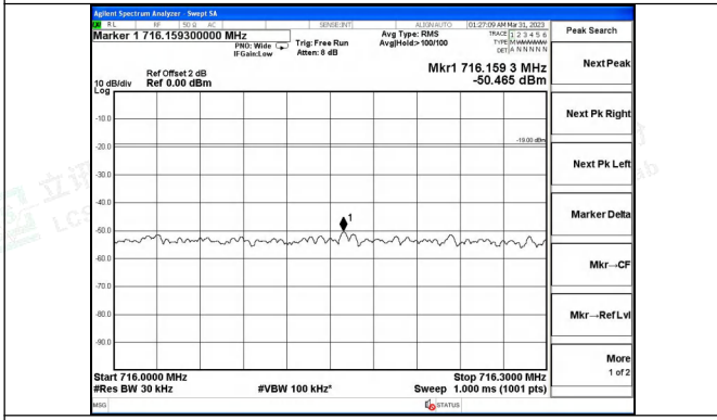
Lower 700MHz band CDMA UL Right Side Pre AGC
