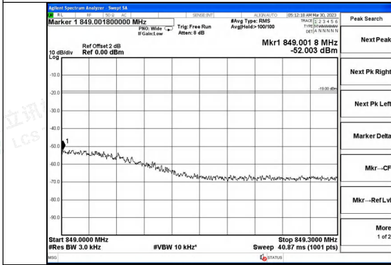
Cellular Band GSM UL Right Side Pre AGC
