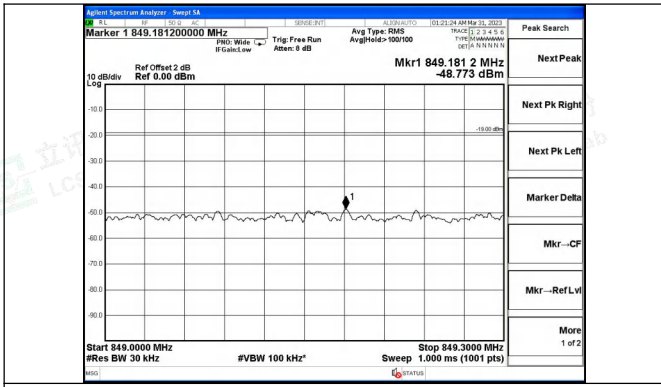
Cellular Band CDMA UL Right Side Pre AGC
