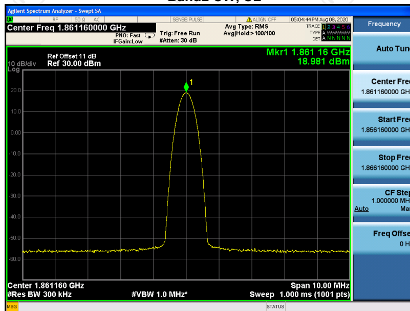
Band2 CW, UL
