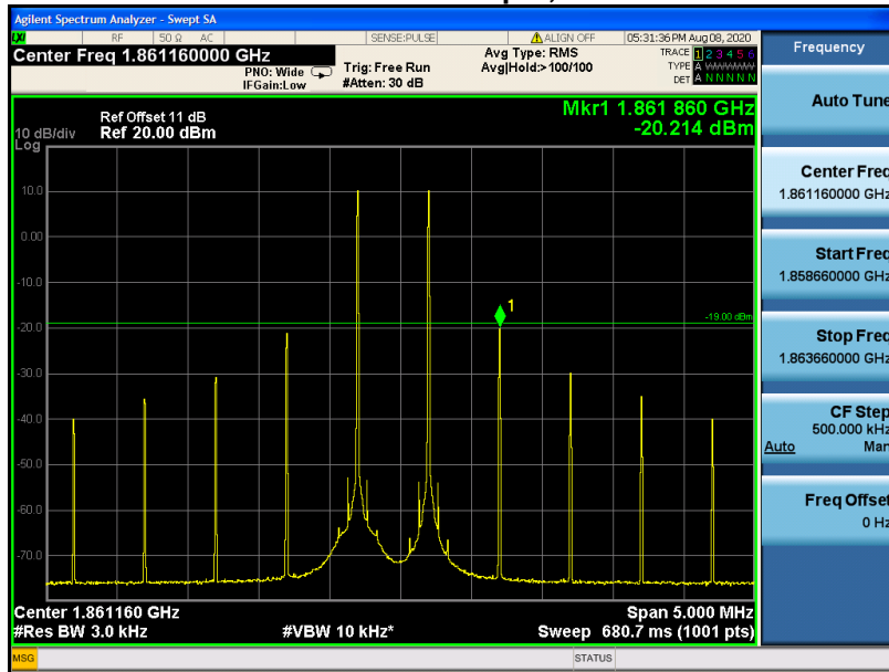
Band2 Max. Input, UL
