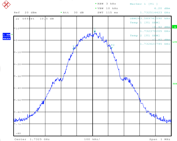
Band4 GSM UL output
