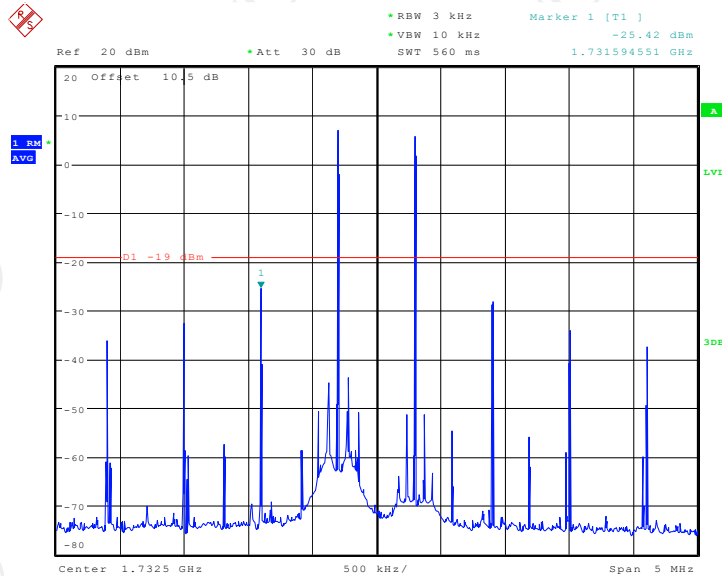
Band4 AGC+10dB, UL
