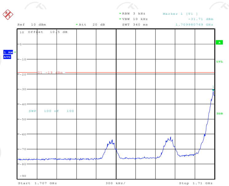
Band4 GSM UL Left Side Pre AGC
