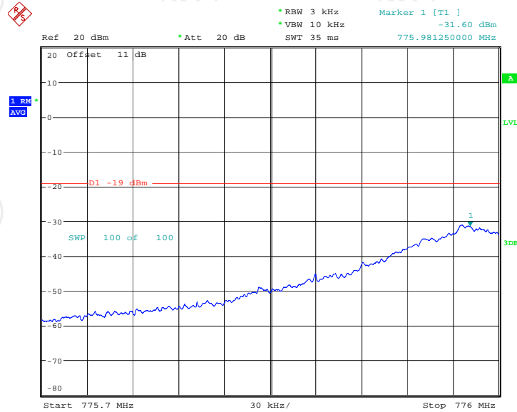
Band13 GSM UL Left Side Max. Input
