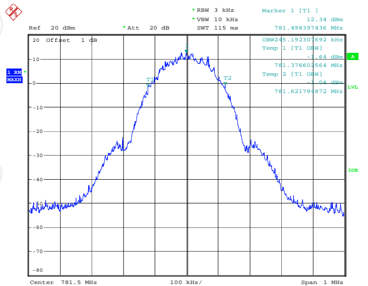
Band13 GSM UL output
