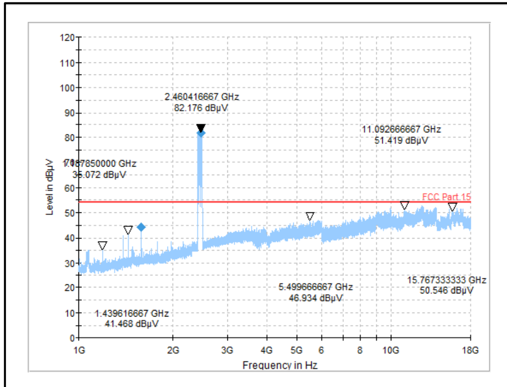
Plot: 1 GHz – 18 GHz: Bluetooth BR/EDR Mode / 3 DH5 / Max Power 9 / Hopping On
