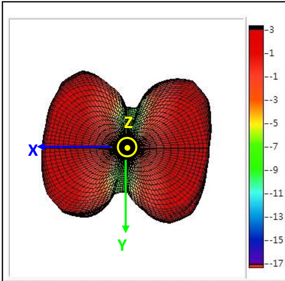
3D Gain Pattern @ 5850 MHz (unit: dBi)
