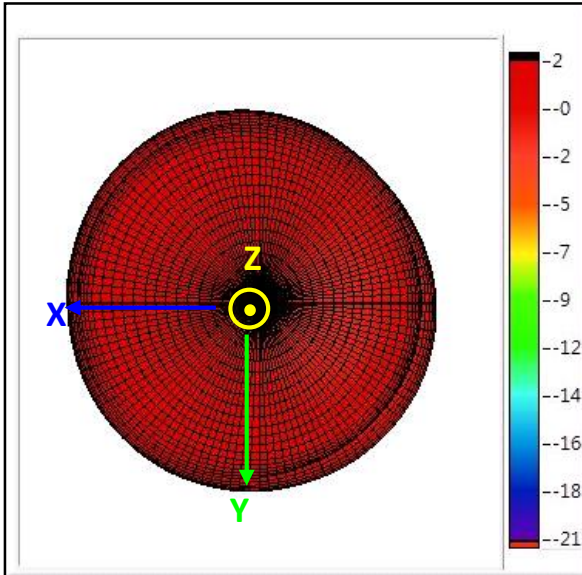
3D Gain Pattern @ 2442 MHz (unit: dBi)
