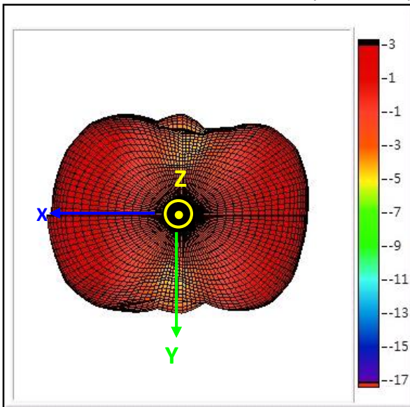
3D Gain Pattern @ 5150 MHz (unit: dBi)
