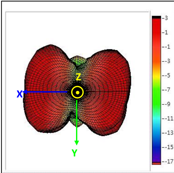
3D Gain Pattern @ 5500 MHz (unit: dBi)
