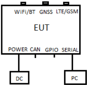
Figure 3.4-1: Setup diagram
