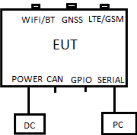
Figure 3.4-1: Setup diagram
