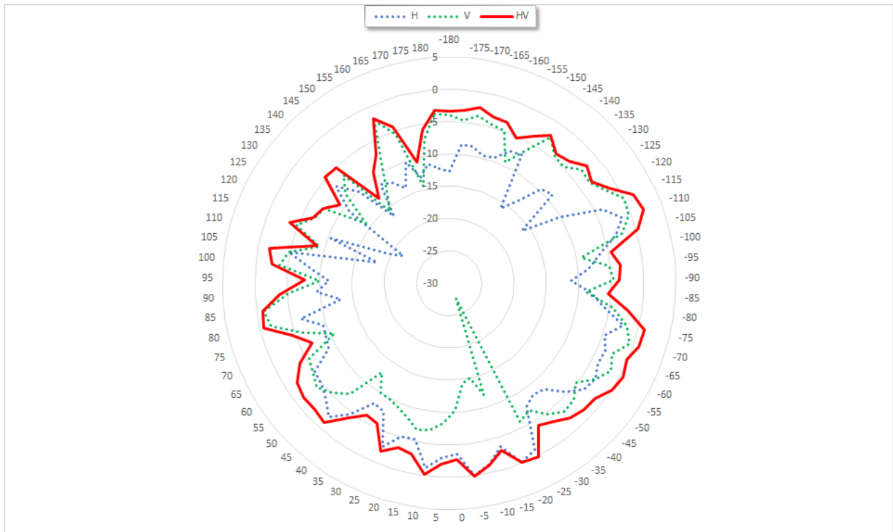
Pattern azimuthal plane 802.11 2440 MHz Blue channel
