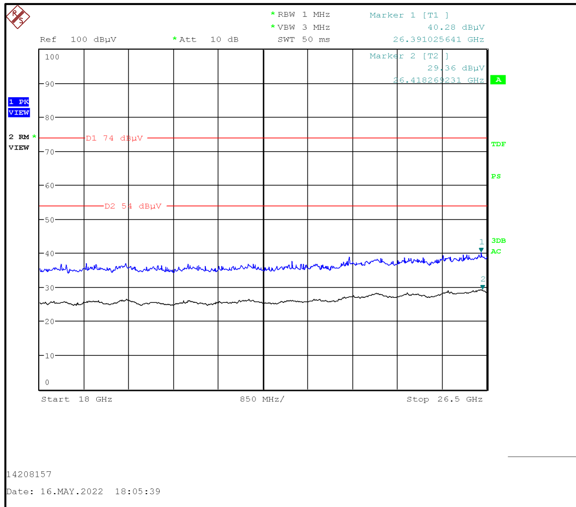
Plot: 18 GHz – 26.5 GHz: BT-EDR Mode / Packet Type: 3DH5 / Hopping OFF/ MAX PWR 7 / Bottom Channel
