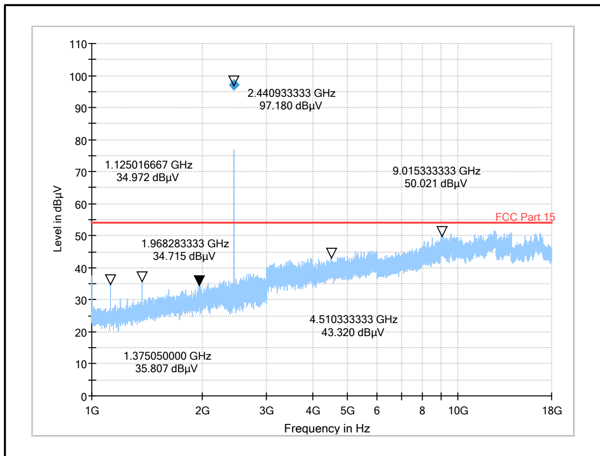
Plot: 1 GHz – 18 GHz: BT-EDR Mode / Packet Type: 3DH5 / Hopping OFF/ MAX PWR 7 / Middle Channel
