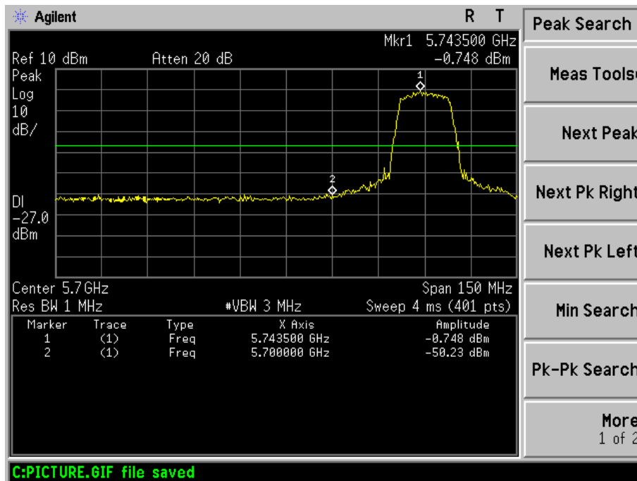
Antenna1 - CH01
