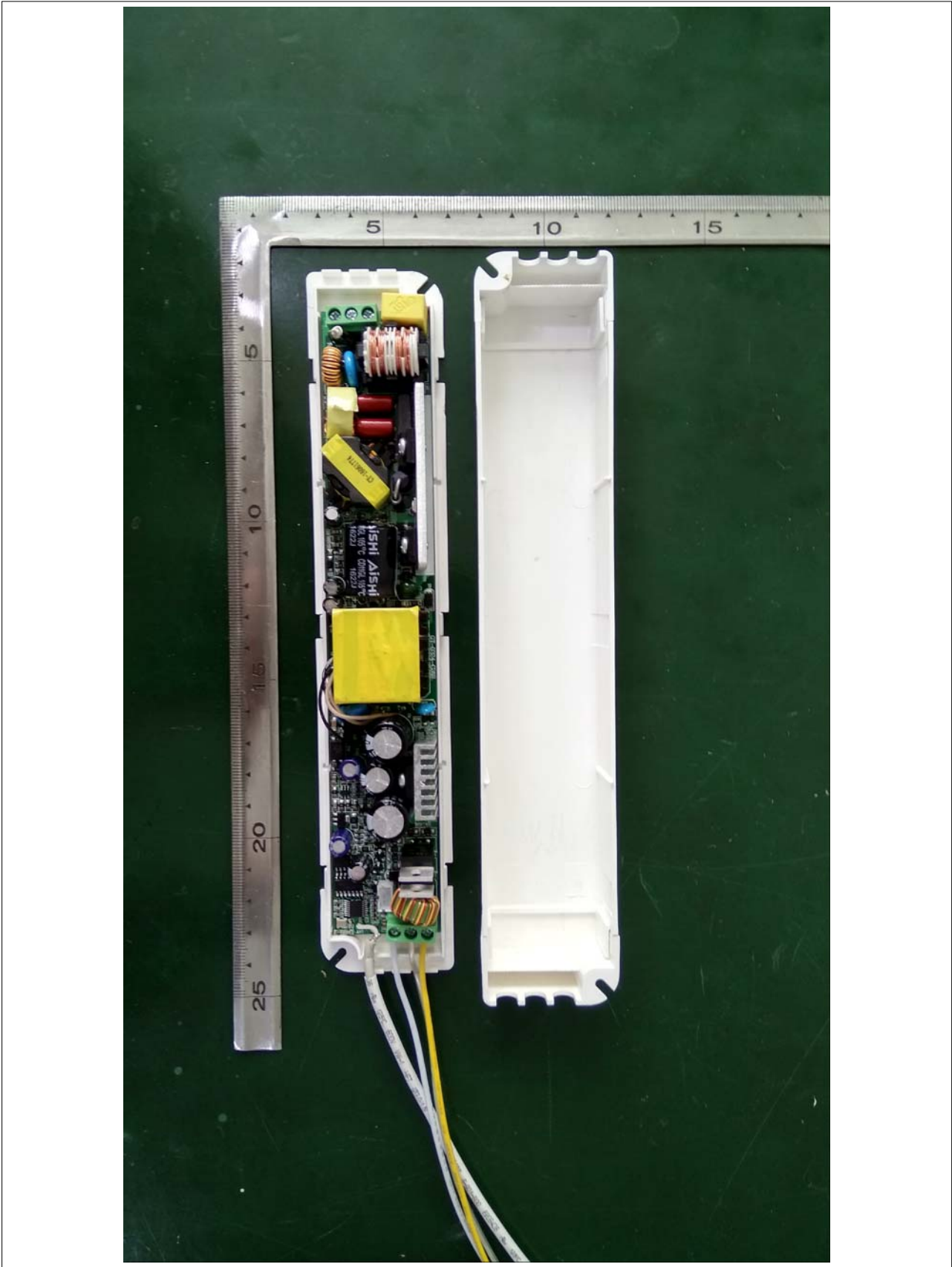
Internal Photos 1(Receiver)
