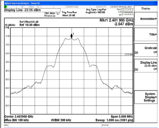
Channel 0 / 2402 MHz
