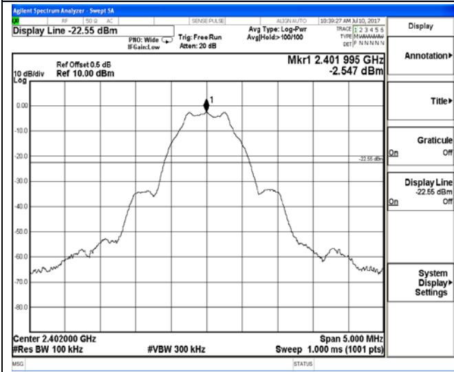
2399.5 MHz – 2404.5 MHz
