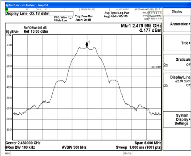
2477.5 MHz – 2482.5 MHz
