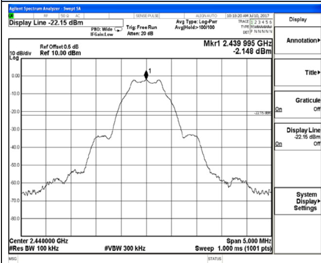
Channel 19 / 2440 MHz
