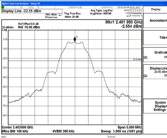
2399.5 – 2404.5 MHz
