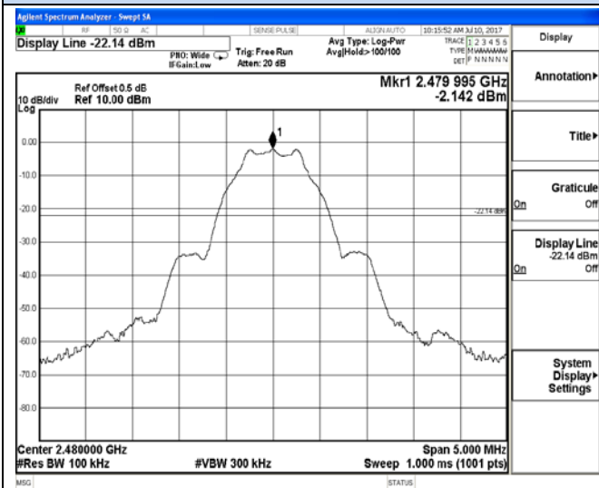
Channel 39 / 2480 MHz
