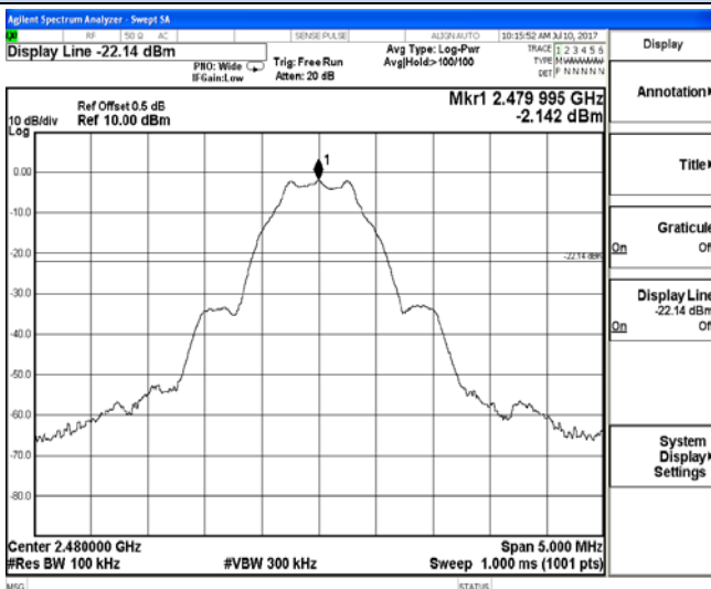
2477.5 – 2482.5 MHz
