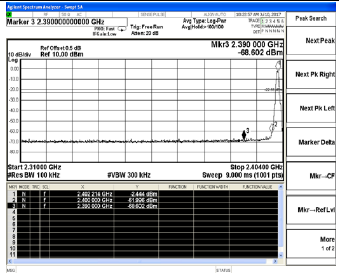
Channel 0 / 2402 MHz
