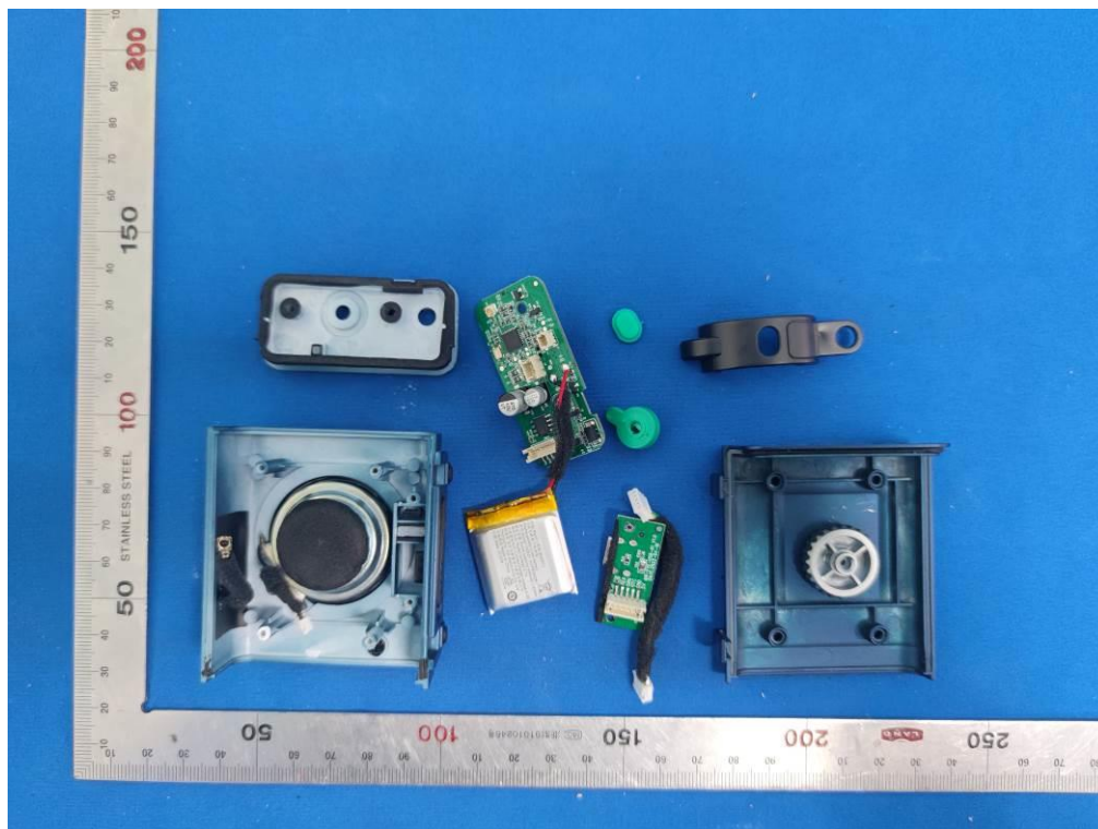
OPEN VIEW-2 OF EUT (FIGURE 1)
