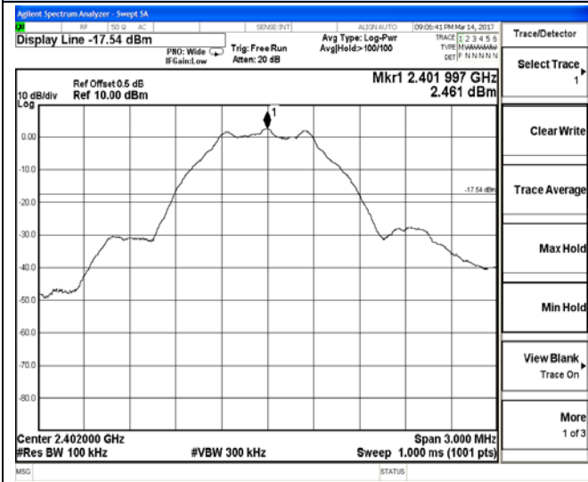
2400.5 – 2403.5 MHz
