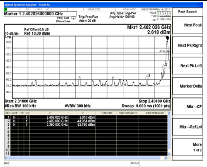
Channel 0 / 2402 MHz
