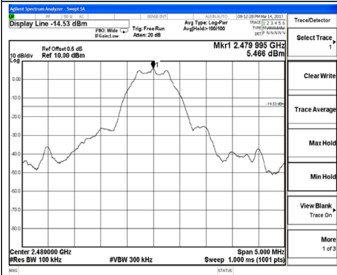
2478.5 – 2481.5 MHz
