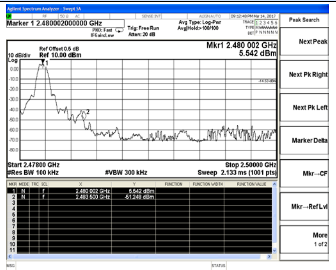
Channel 39 / 2480 MHz
