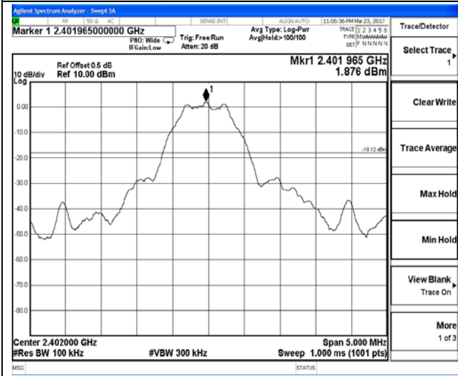
2399.5 – 2404.5 MHz
