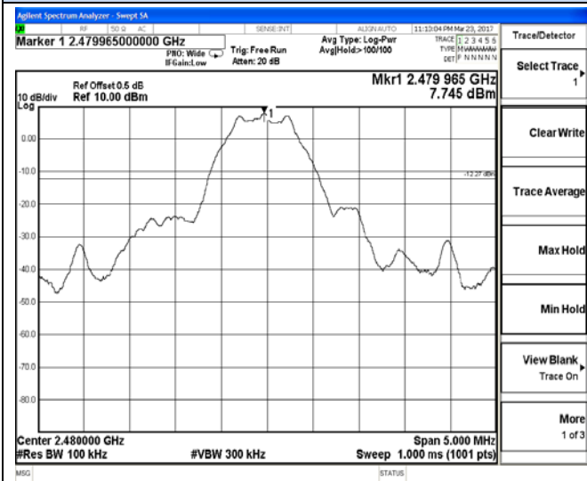
2477.5 – 2482.5 MHz
