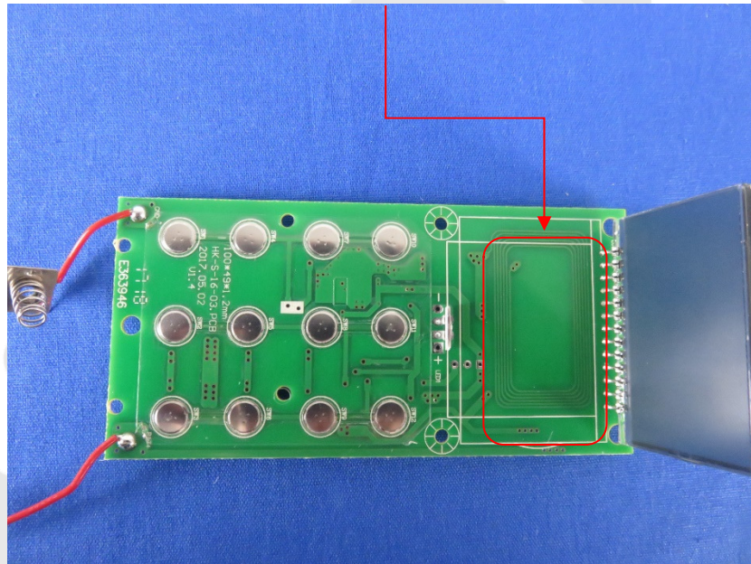
Loop Antenna
