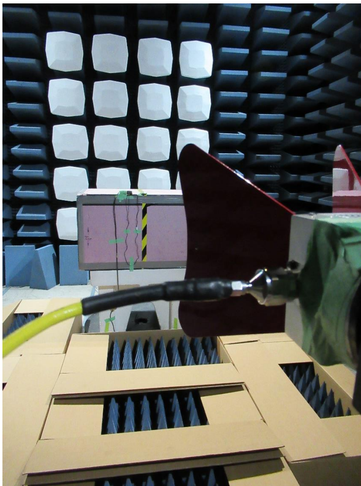
Figure 3: Radiated Emissions (1 – 18 GHz)
