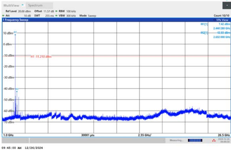
BLE_2M-Ant1-2440-1000~26500-PASS
