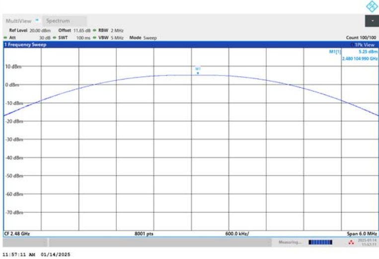
BLE_1M-Ant1-2480-PASS
