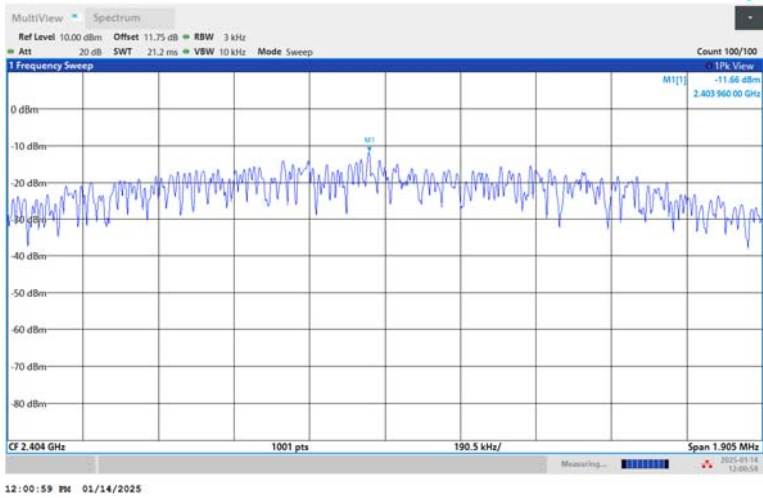
BLE_2M-Ant1-2404-PASS
