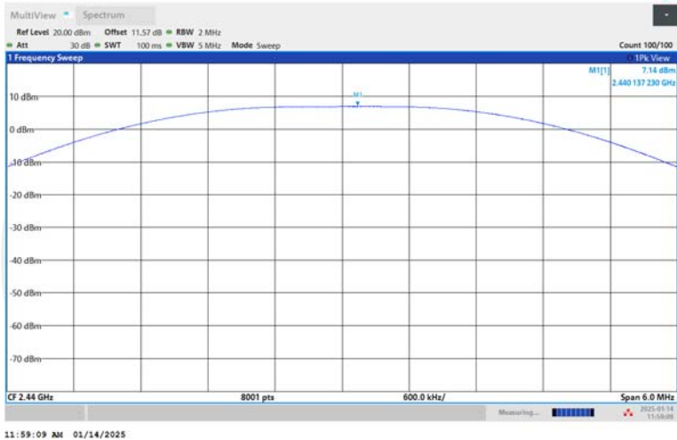
BLE_2M-Ant1-2440-PASS
