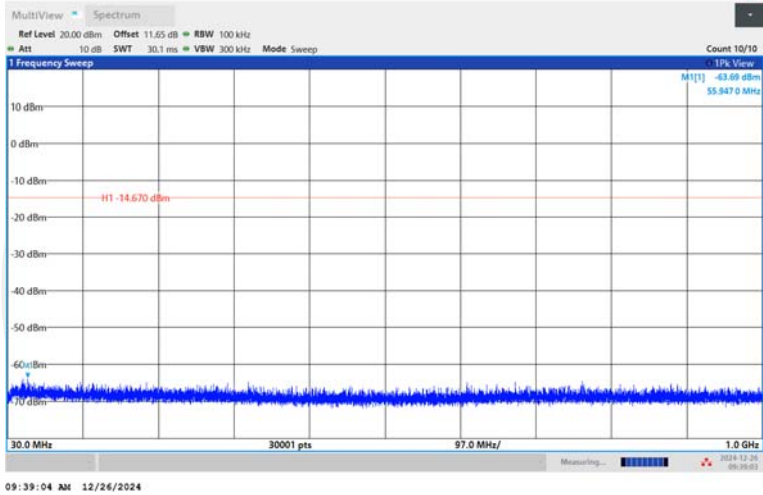
BLE_1M-Ant1-2480-30~1000-PASS
