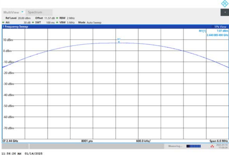
BLE_1M-Ant1-2440-PASS
