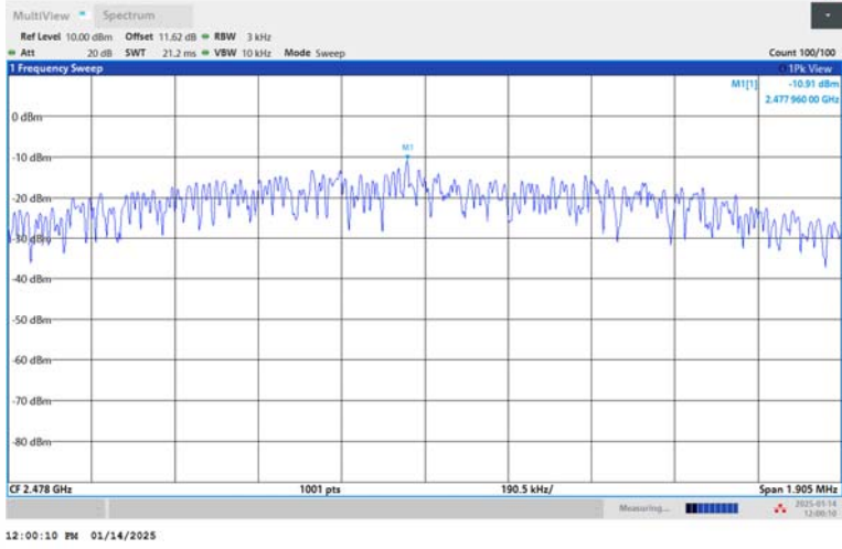
BLE_2M-Ant1-2478-PASS
