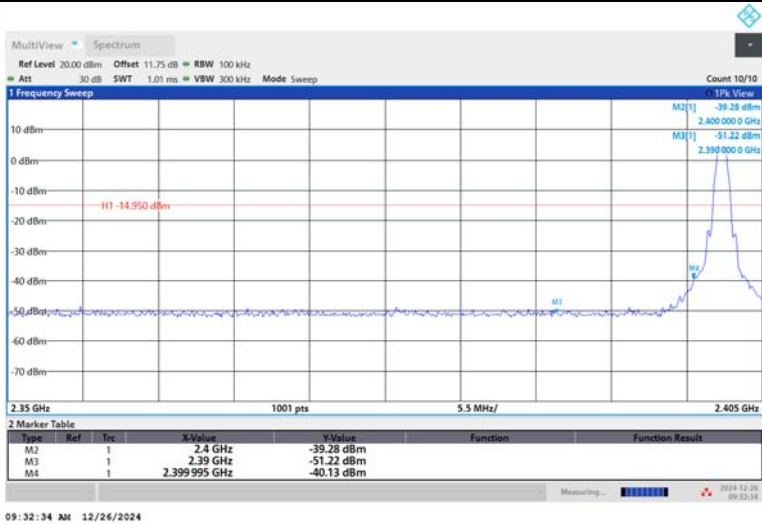
BLE_1M-Ant1-2402-PASS
