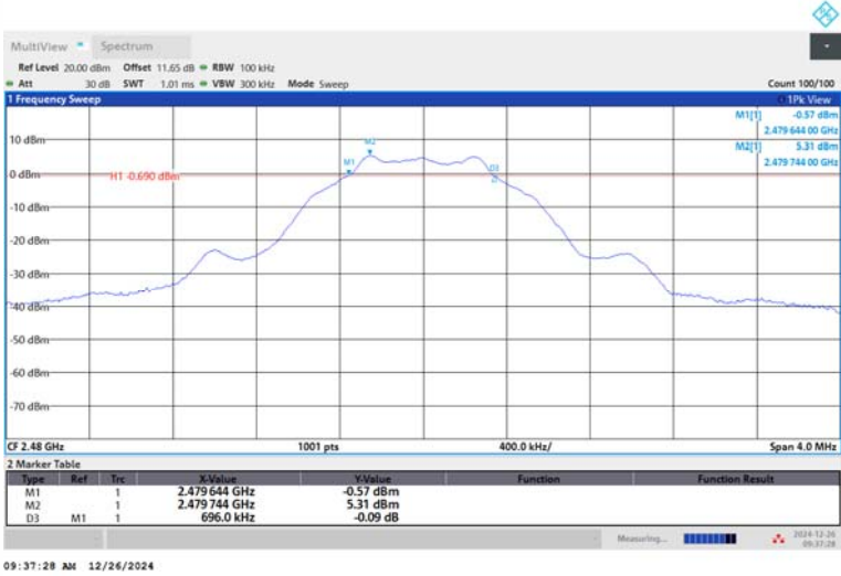
BLE_1M-Ant1-2480-PASS
