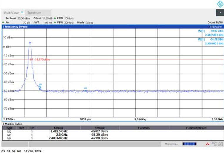
BLE_1M-Ant1-2480-PASS
