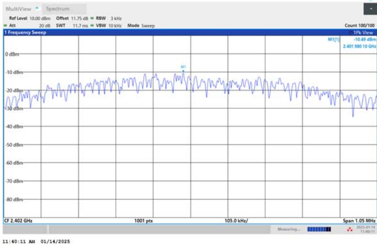
BLE_1M-Ant1-2402-PASS
