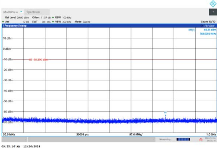
BLE_1M-Ant1-2440-30~1000-PASS
