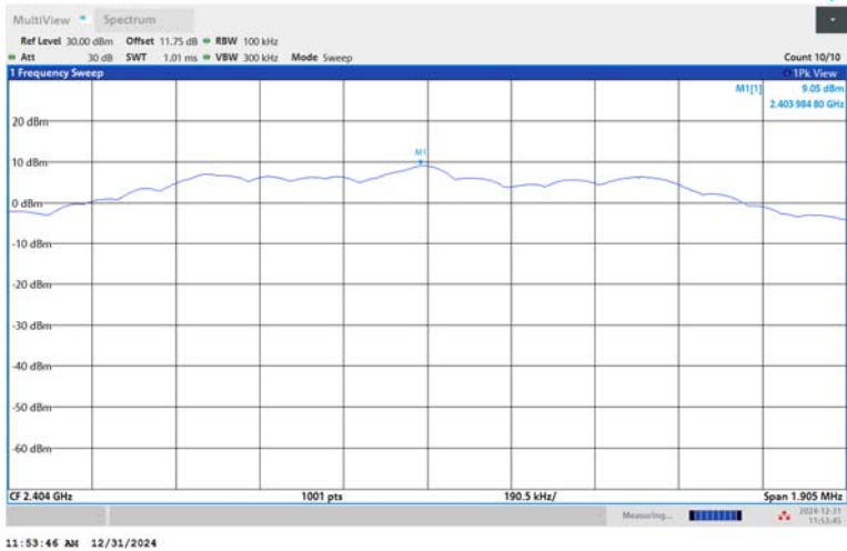
BLE_2M-Ant1-2404-PASS
