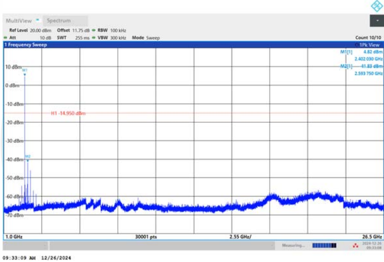
BLE_1M-Ant1-2402-1000~26500-PASS
