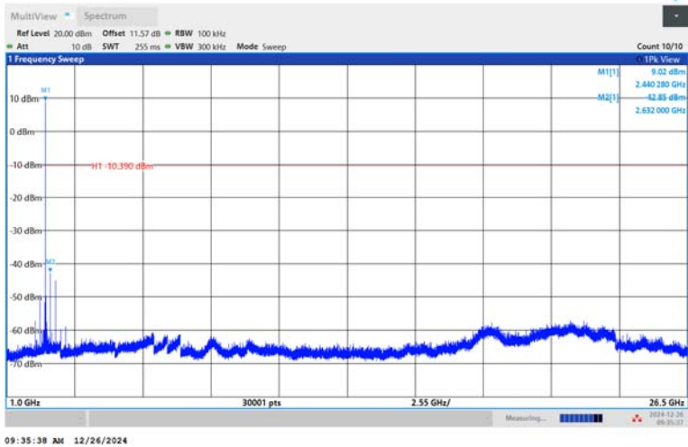
BLE_1M-Ant1-2440-1000~26500-PASS
