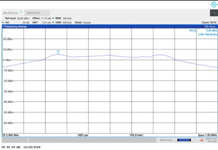
BLE_1M-Ant1-2402-PASS
