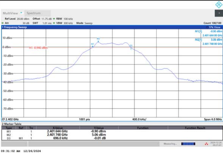
BLE_1M-Ant1-2402-PASS
