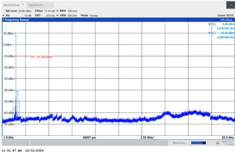
BLE_2M-Ant1-2478-1000~26500-PASS
