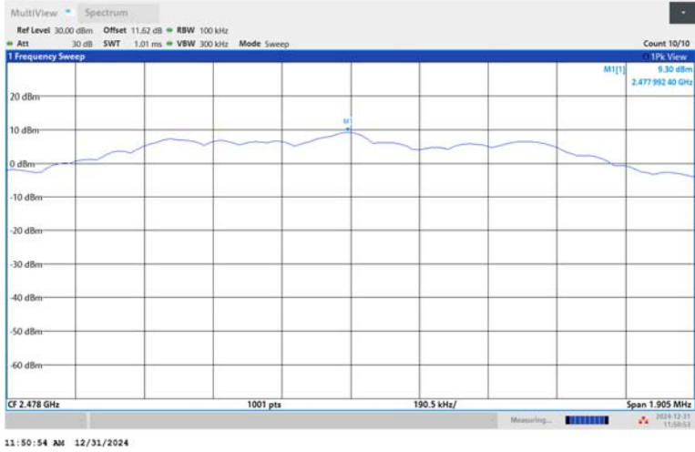
BLE_2M-Ant1-2478-PASS
