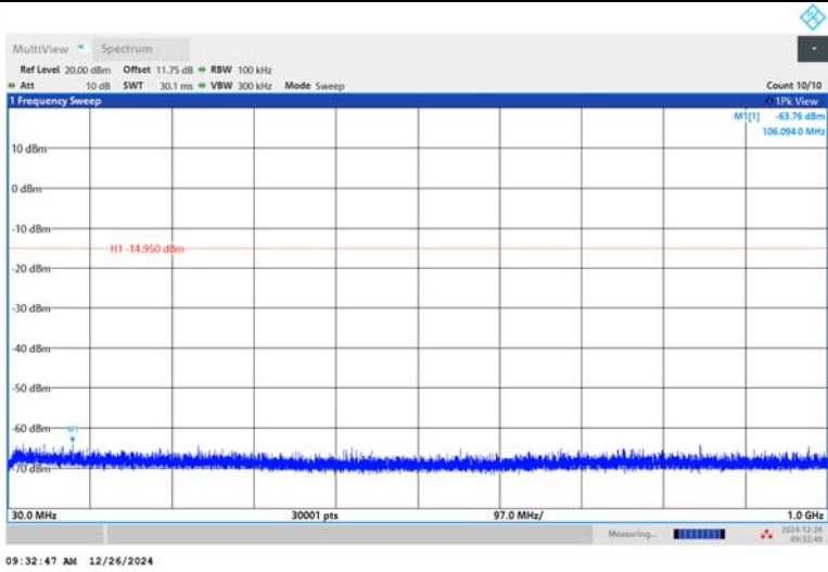
BLE_1M-Ant1-2402-30~1000-PASS
