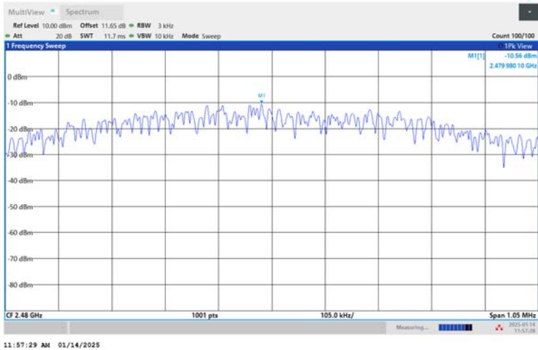
BLE_1M-Ant1-2480-PASS
