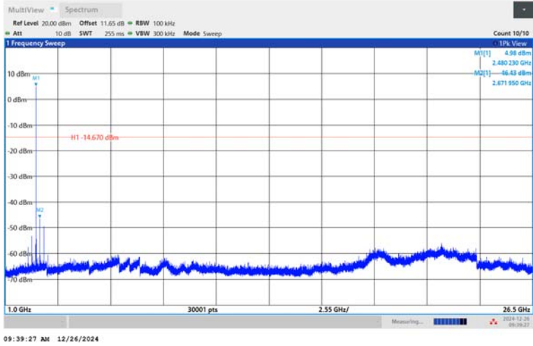
BLE_1M-Ant1-2480-1000~26500-PASS
