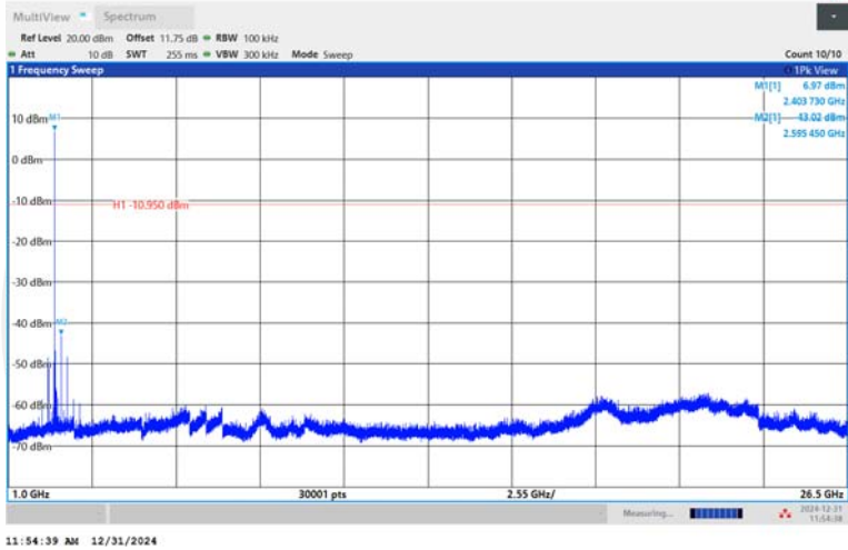
BLE_2M-Ant1-2404-1000~26500-PASS
