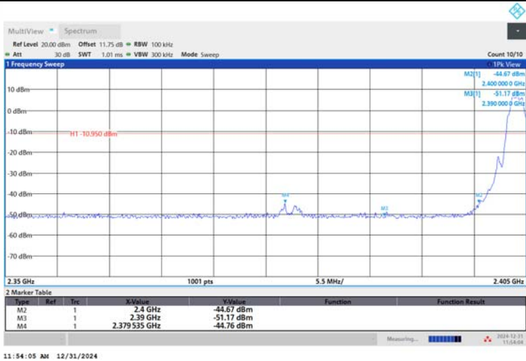
BLE_2M-Ant1-2404-PASS
