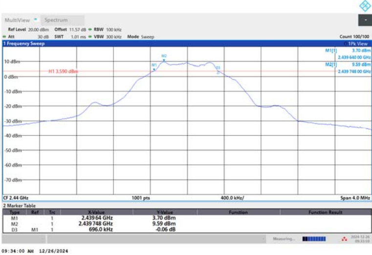
BLE_1M-Ant1-2440-PASS
