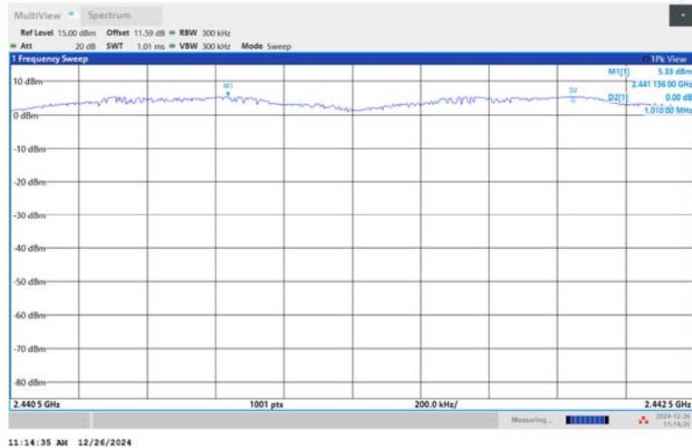
3DH5-Ant1-Hop_2441-PASS
