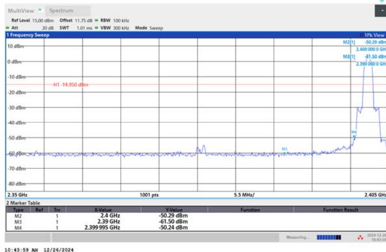
2DH5-Ant1-2402-PASS
