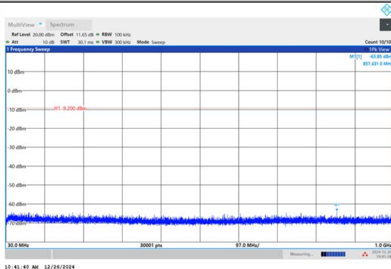
DH5-Ant1-2480-30~1000-PASS
