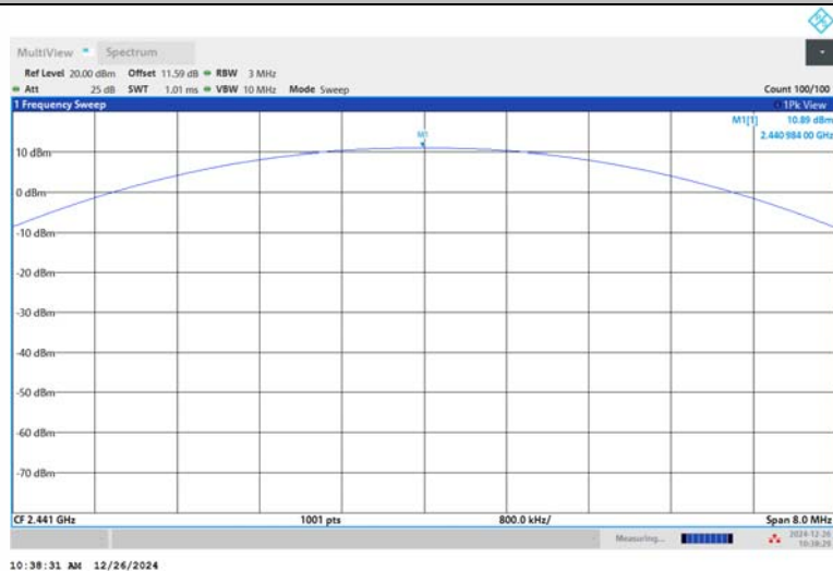
DH5-Ant1-2441-PASS
