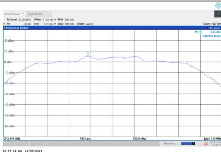
2DH5-Ant1-2441-PASS
