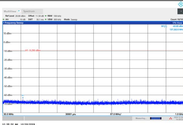
DH5-Ant1-2441-30~1000-PASS
