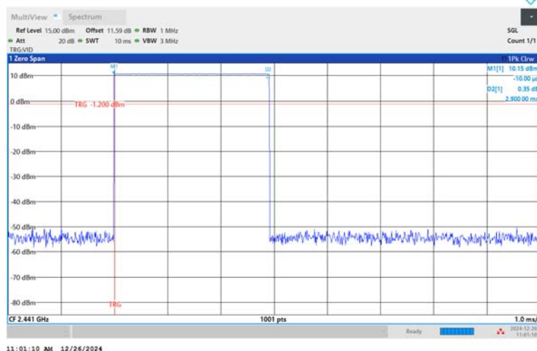
DH5-Ant1-Hop-PASS
