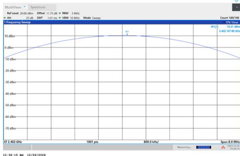
DH5-Ant1-2402-PASS
