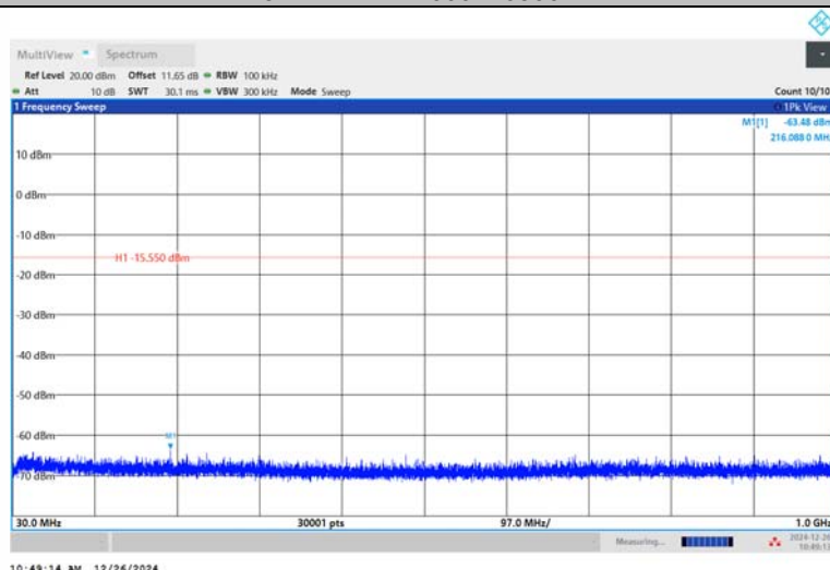
2DH5-Ant1-2480-30~1000-PASS
