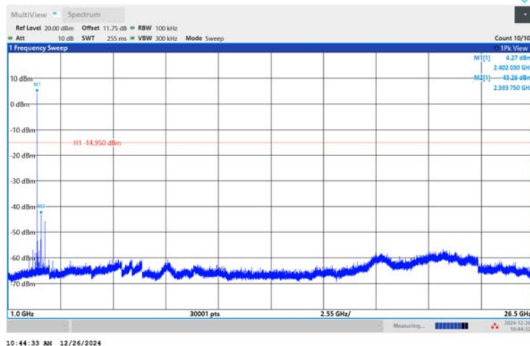
2DH5-Ant1-2402-1000~26500-PASS
