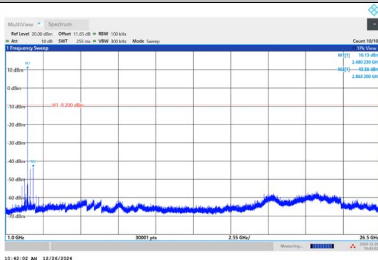
DH5-Ant1-2480-1000~26500-PASS
