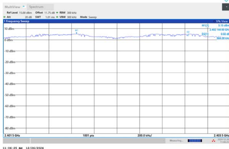
2DH5-Ant1-Hop_2402-PASS
