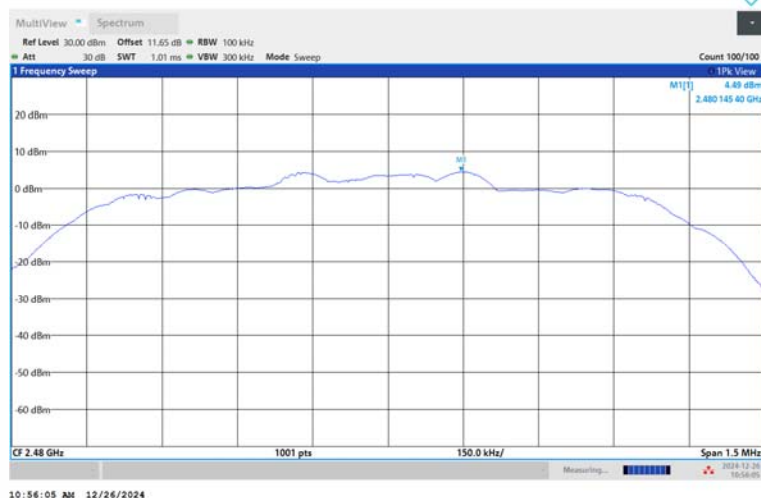
3DH5-Ant1-2480-PASS
