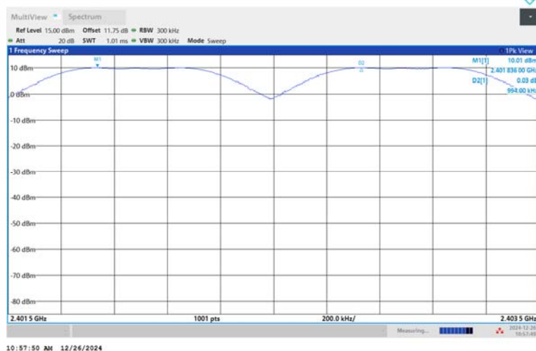
DH5-Ant1-Hop_2402-PASS
