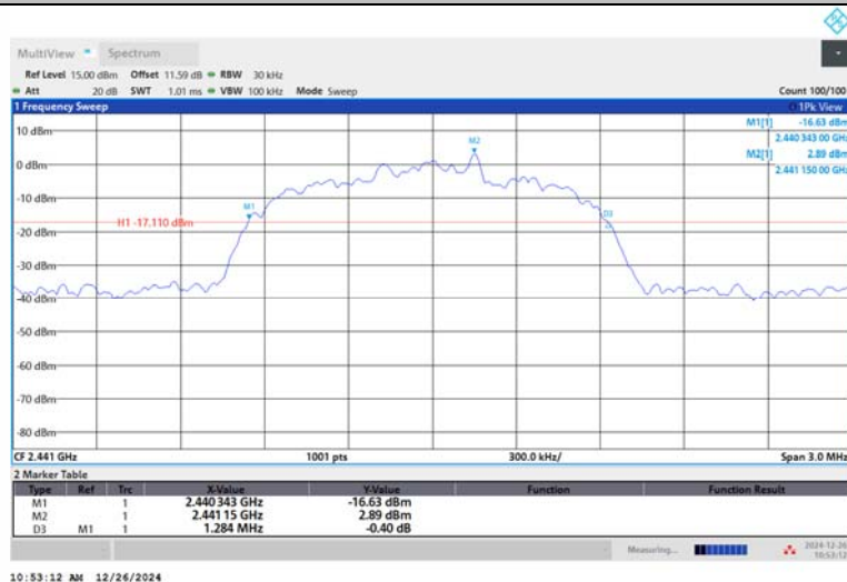
3DH5-Ant1-2441
