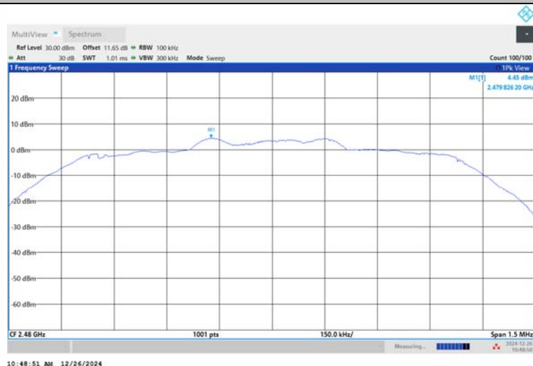
2DH5-Ant1-2480-PASS
