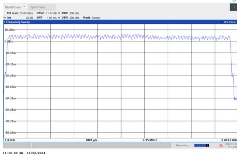
2DH5-Ant1-Hop-PASS
