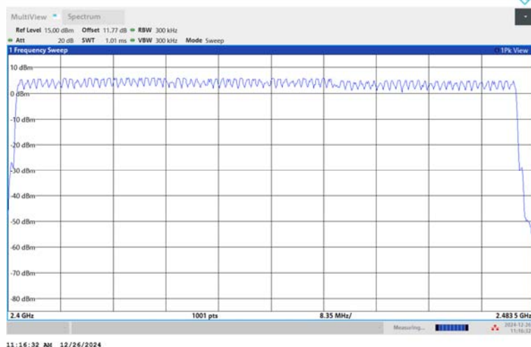
3DH5-Ant1-Hop-PASS
