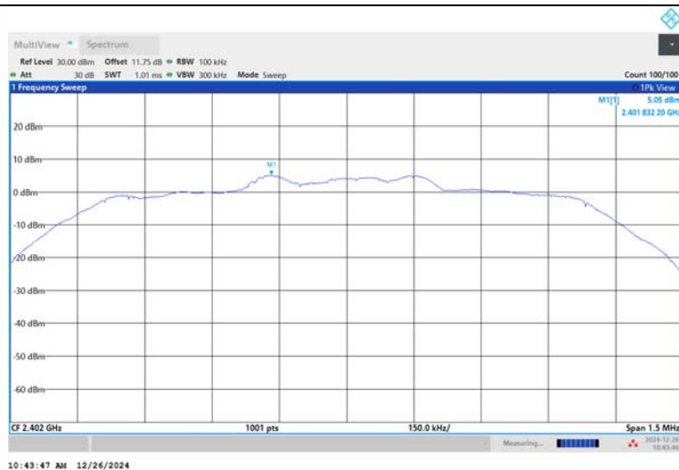
2DH5-Ant1-2402-PASS
