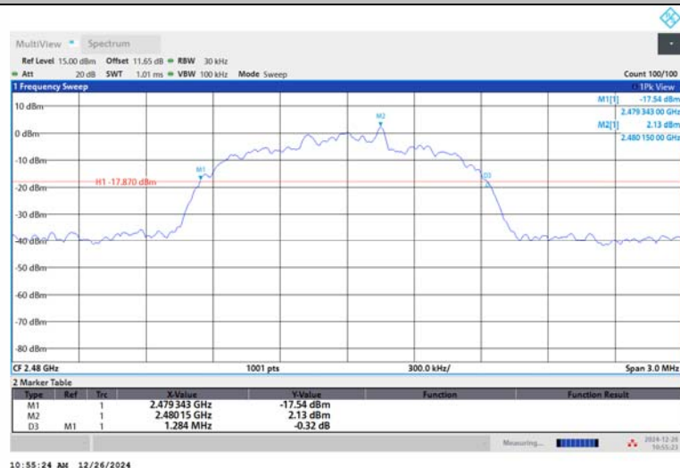
3DH5-Ant1-2480
