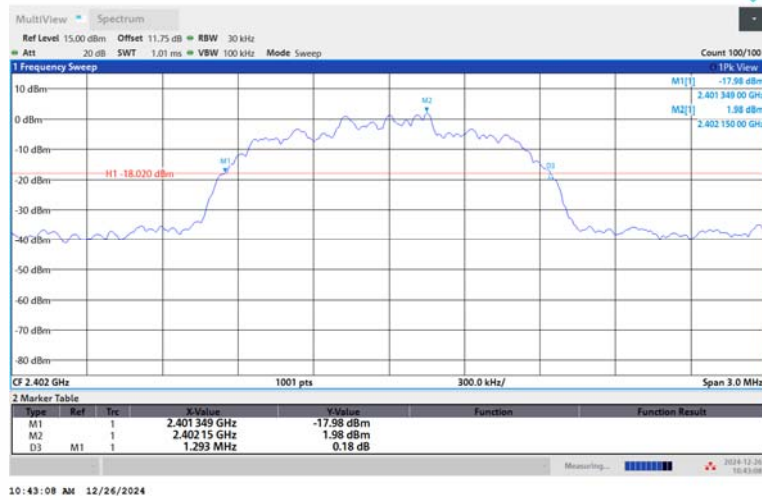
2DH5-Ant1-2402
