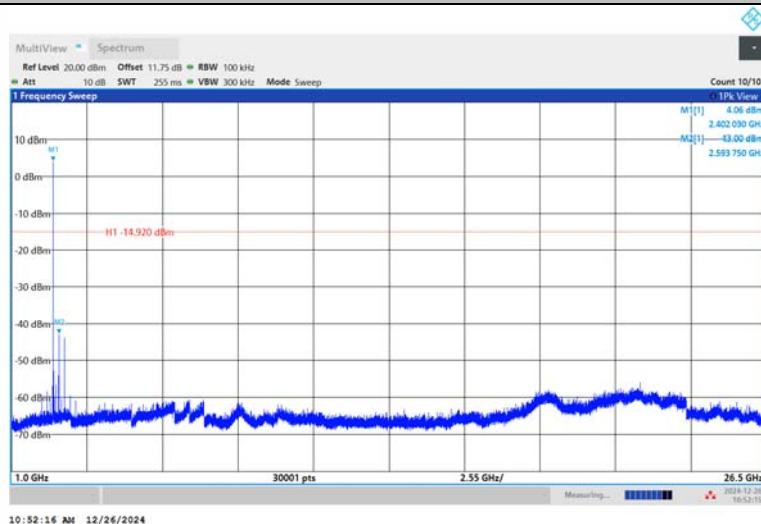
3DH5-Ant1-2402-1000~26500-PASS
