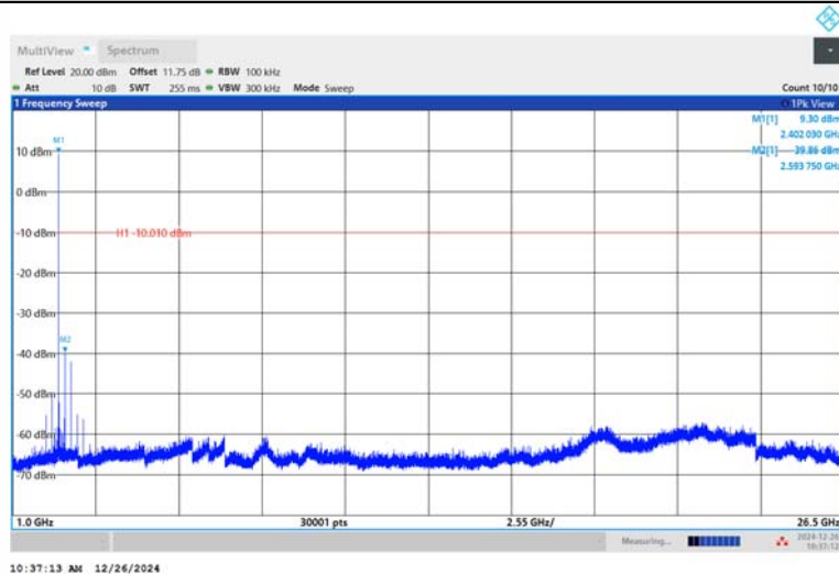
DH5-Ant1-2402-1000~26500-PASS
