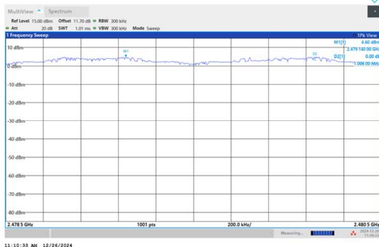
2DH5-Ant1-Hop_2480-PASS
