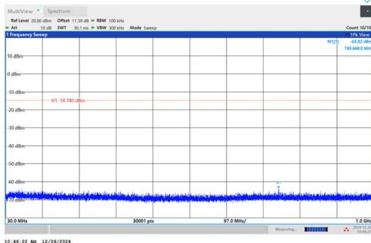
2DH5-Ant1-2441-30~1000-PASS
