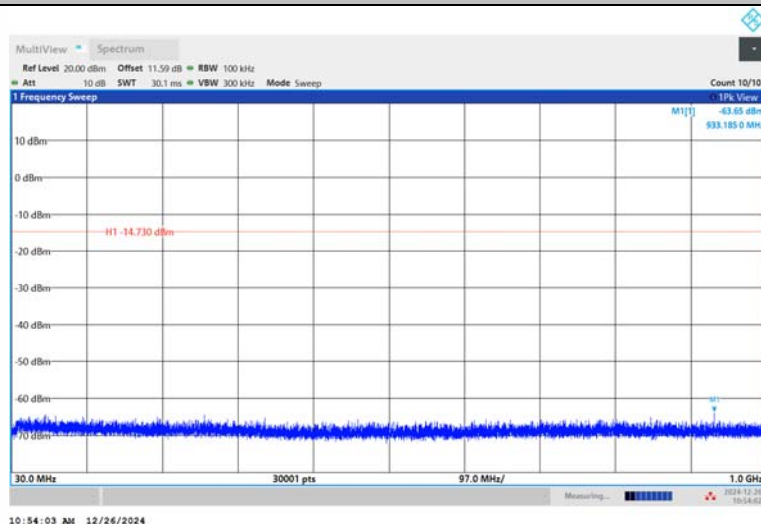
3DH5-Ant1-2441-30~1000-PASS
