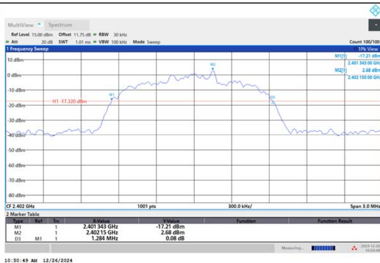
3DH5-Ant1-2402
