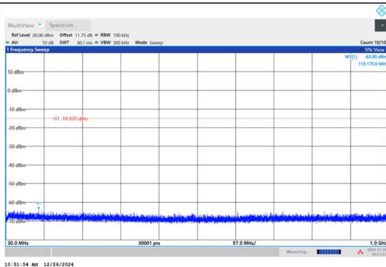
3DH5-Ant1-2402-30~1000-PASS
