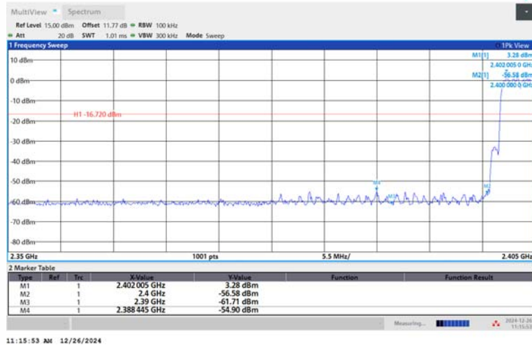
3DH5-Ant1-Hop_2402-PASS
