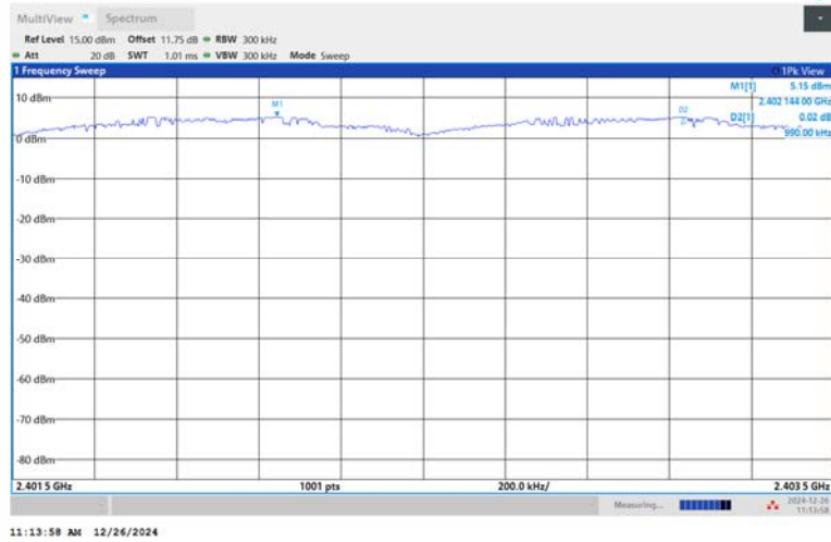
3DH5-Ant1-Hop_2402-PASS
