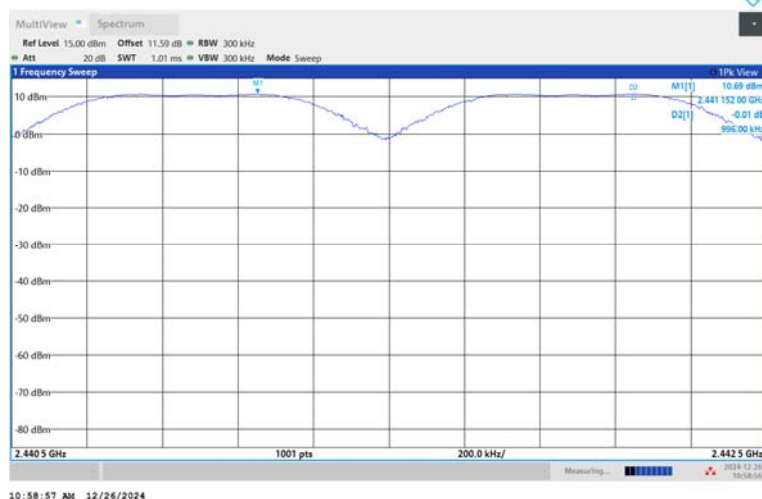
DH5-Ant1-Hop_2441-PASS
