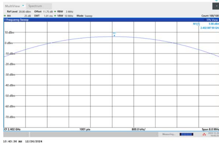
2DH5-Ant1-2402-PASS
