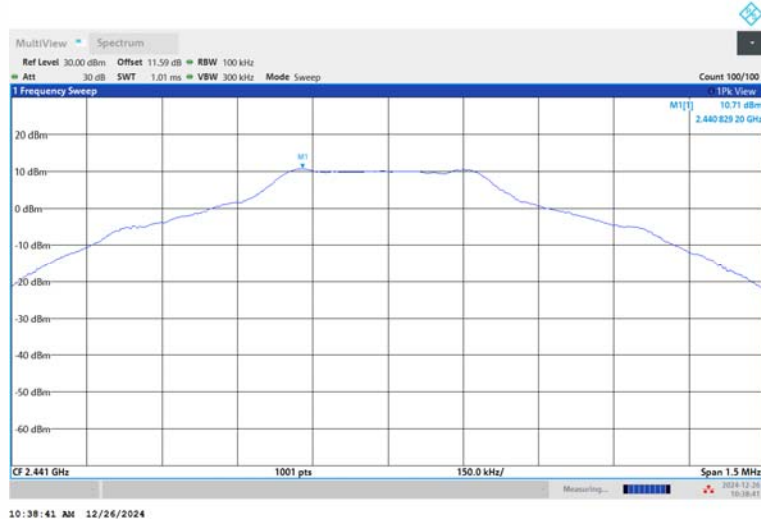
DH5-Ant1-2441-PASS
