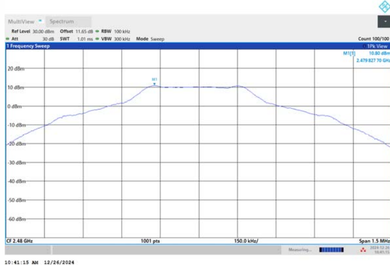
DH5-Ant1-2480-PASS
