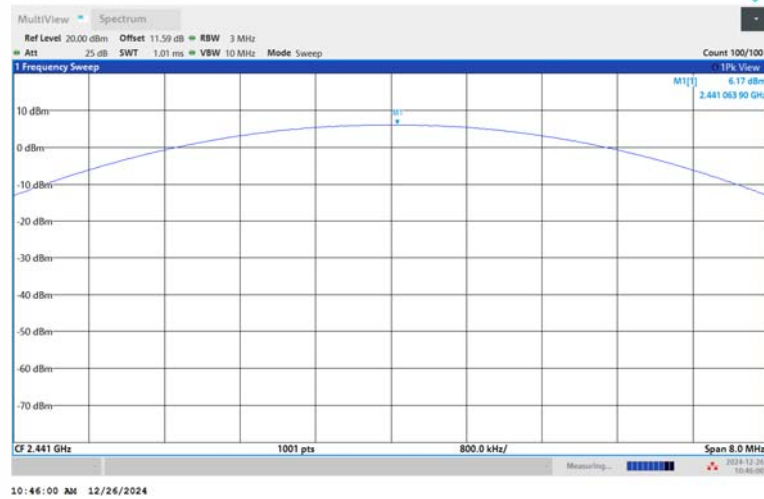
2DH5-Ant1-2441-PASS
