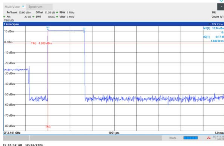
DH3-Ant1-Hop-PASS
