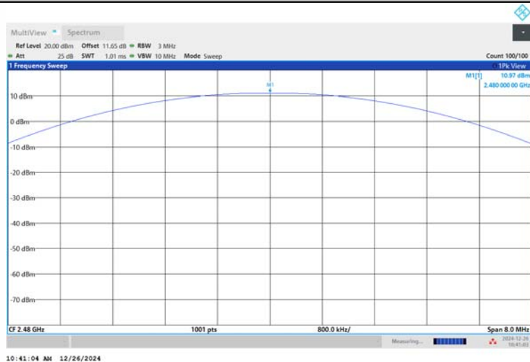
DH5-Ant1-2480-PASS
