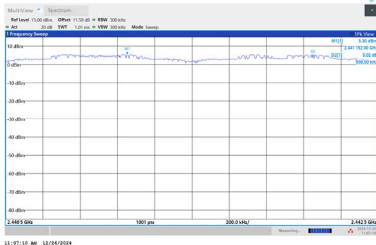
2DH5-Ant1-Hop_2441-PASS
