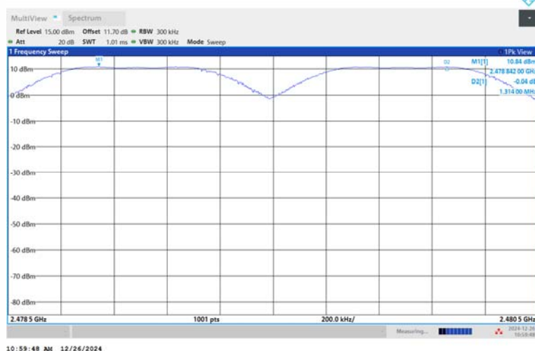
DH5-Ant1-Hop_2480-PASS
