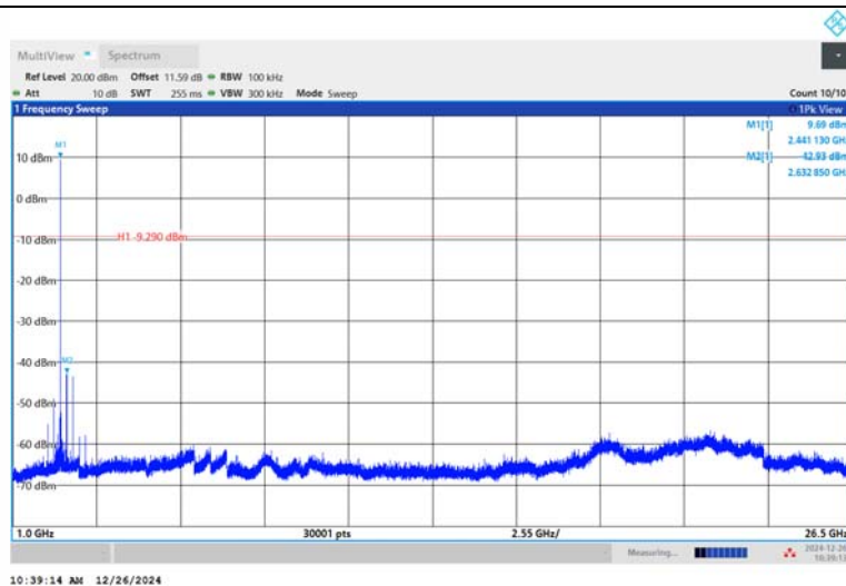
DH5-Ant1-2441-1000~26500-PASS
