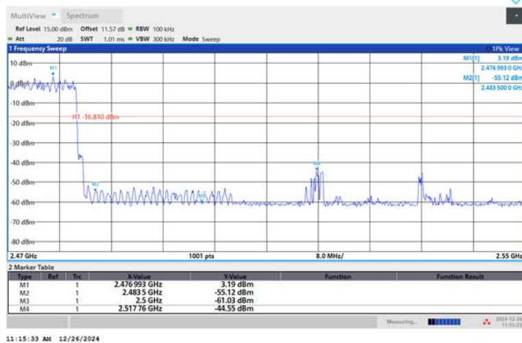
3DH5-Ant1-Hop_2480-PASS
