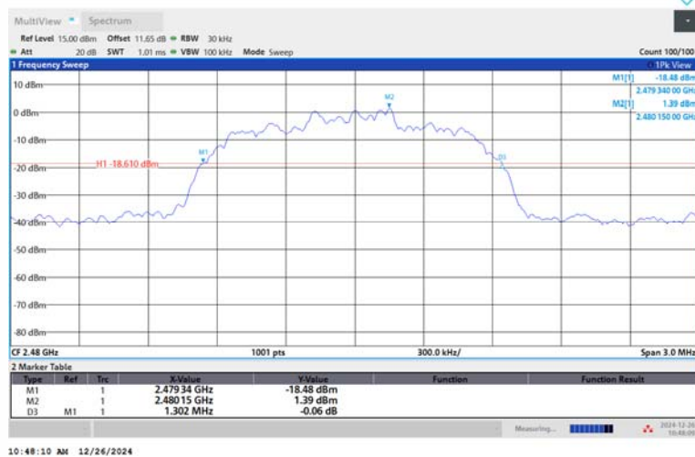
2DH5-Ant1-2480
