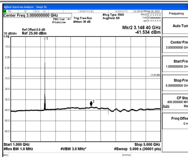
Band25-10MHz-QPSK-26640-1-0-High-1000-5000--41.53-PASS
