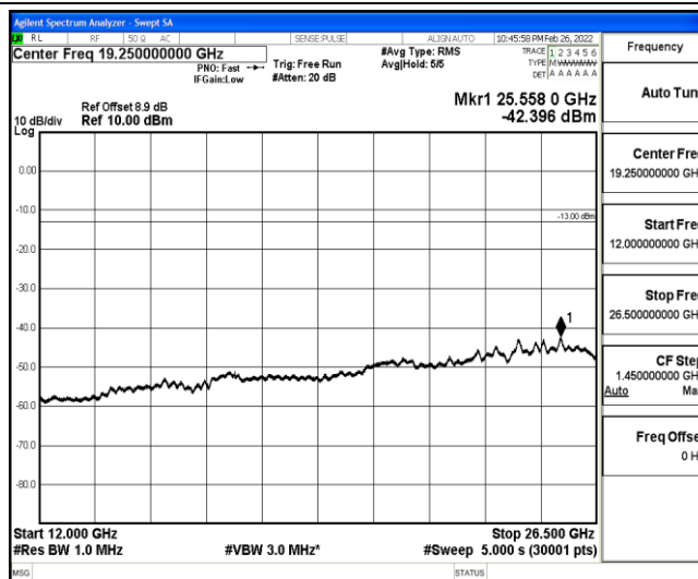
Band25-5MHz-16QAM-26365-1-0-Low-12000-26500--42.4-PASS
