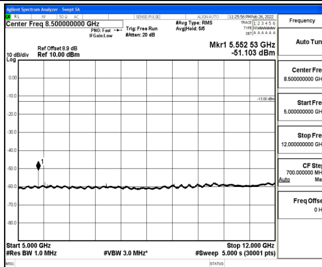
Band25-10MHz-QPSK-26090-1-0-Low-5000-12000--51.1-PASS
