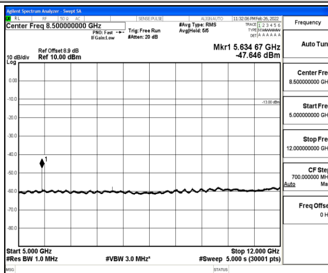
Band25-10MHz-16QAM-26365-1-0-Low-5000-12000--47.65-PASS
