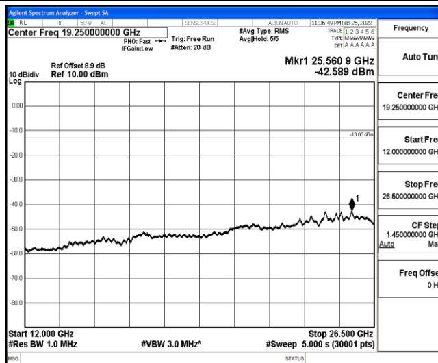
Band25-10MHz-16QAM-26640-1-0-High-12000-26500--42.59-PASS
