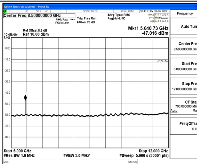
Band25-5MHz-QPSK-26365-1-0-Low-5000-12000--47.02-PASS
