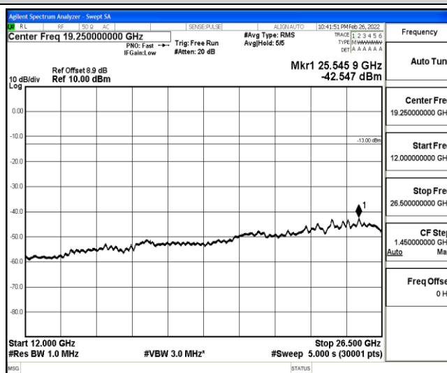
Band25-5MHz-16QAM-26065-1-0-Low-12000-26500--42.55-PASS
