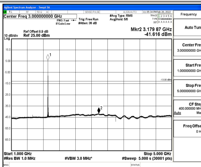
Band25-10MHz-16QAM-26640-1-0-High-1000-5000--41.62-PASS
