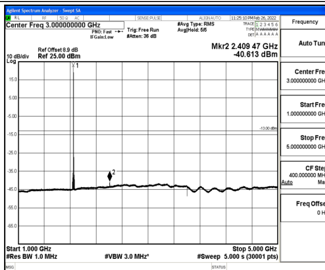
Band25-10MHz-QPSK-26090-1-0-Low-1000-5000--40.61-PASS
