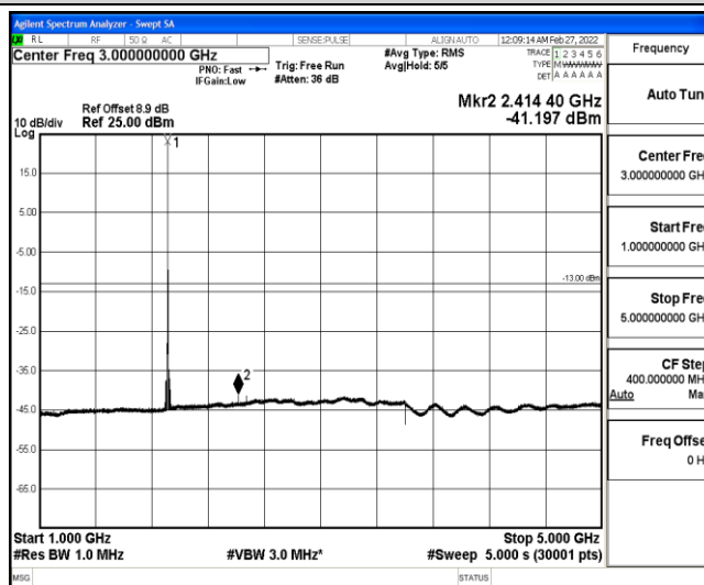
Band25-15MHz-QPSK-26615-1-0-High-1000-5000--41.2-PASS
