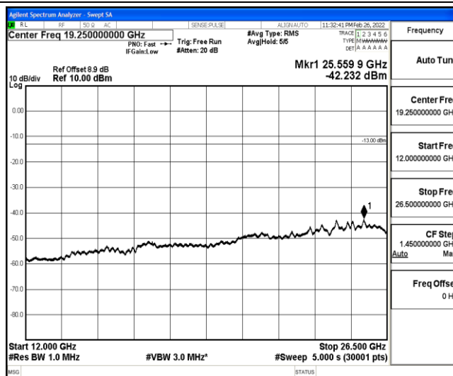
Band25-10MHz-16QAM-26365-1-0-Low-12000-26500--42.23-PASS
