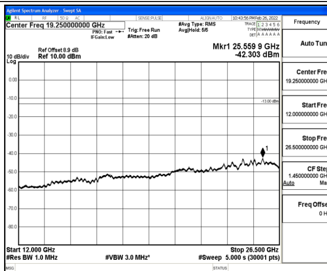
Band25-5MHz-QPSK-26365-1-0-Low-12000-26500--42.3-PASS
