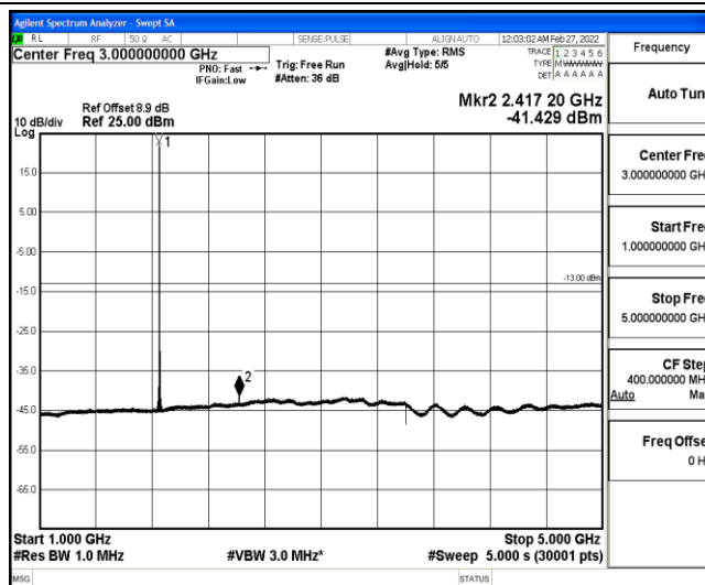
Band25-15MHz-16QAM-26115-1-0-Low-1000-5000--41.43-PASS
