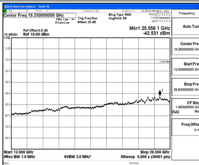
Band25-20MHz-QPSK-26365-1-0-Low-12000-26500--42.53-PASS
