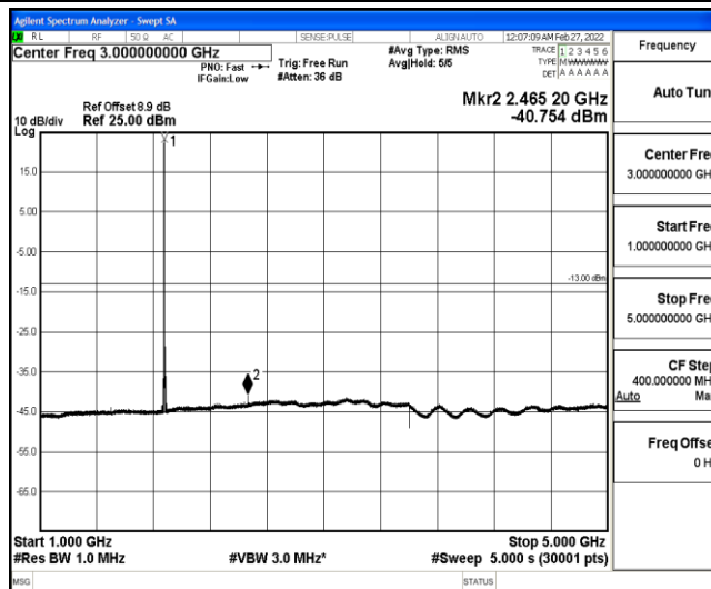
Band25-15MHz-16QAM-26365-1-0-Low-1000-5000--40.75-PASS
