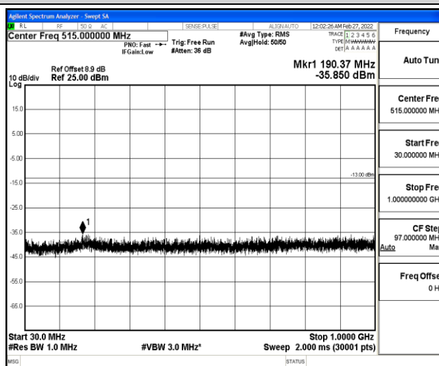
Band25-15MHz-16QAM-26115-1-0-Low-30-1000--35.85-PASS
