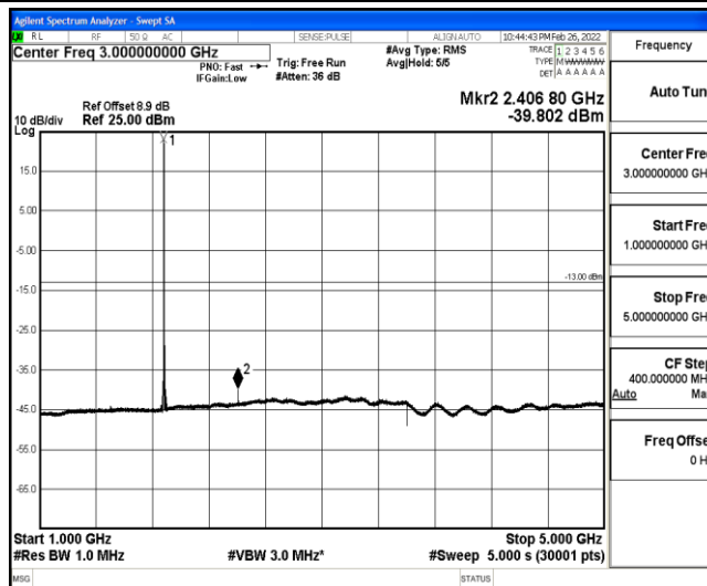
Band25-5MHz-16QAM-26365-1-0-Low-1000-5000--39.8-PASS
