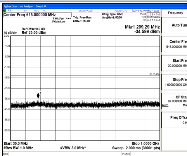
Band25-20MHz-QPSK-26590-1-0-High-30-1000--34.6-PASS
