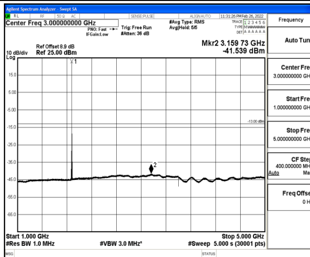
Band25-10MHz-16QAM-26365-1-0-Low-1000-5000--41.54-PASS
