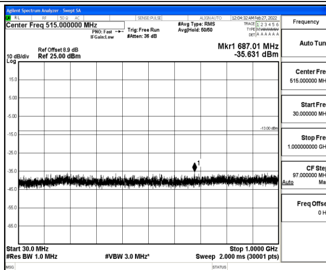
Band25-15MHz-QPSK-26365-1-0-Low-30-1000--35.63-PASS
