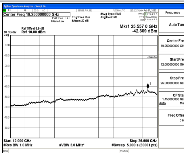
Band25-15MHz-16QAM-26615-1-0-High-12000-26500--42.31-PASS
