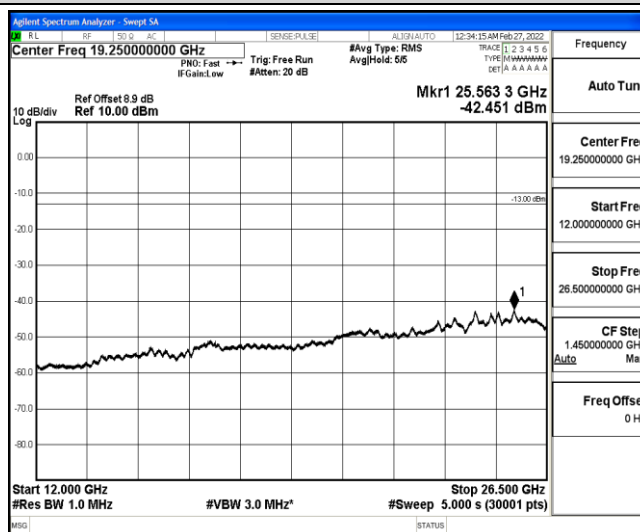
Band25-20MHz-QPSK-26140-1-0-Low-12000-26500--42.45-PASS
