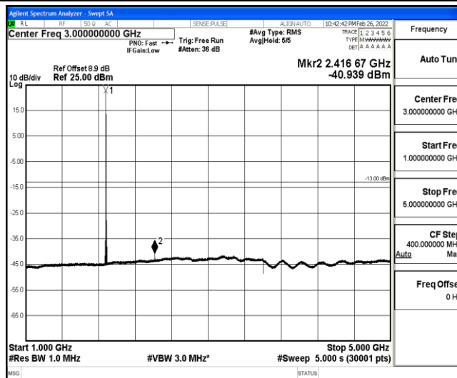
Band25-5MHz-QPSK-26365-1-0-Low-1000-5000--40.94-PASS
