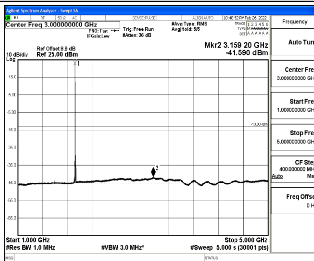
Band25-5MHz-16QAM-26665-1-0-High-1000-5000--41.59-PASS
