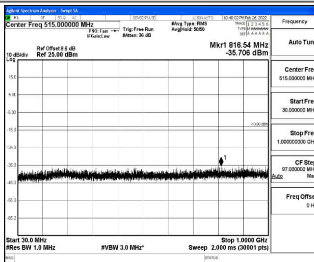
Band25-5MHz-16QAM-26065-1-0-Low-30-1000--35.71-PASS
