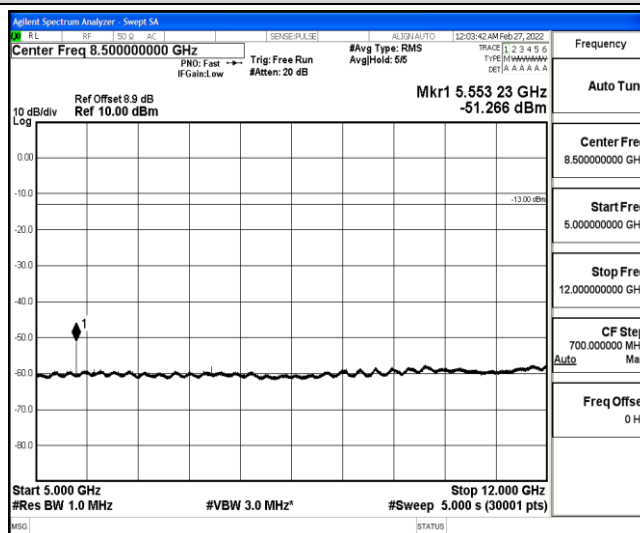
Band25-15MHz-16QAM-26115-1-0-Low-5000-12000--51.27-PASS
