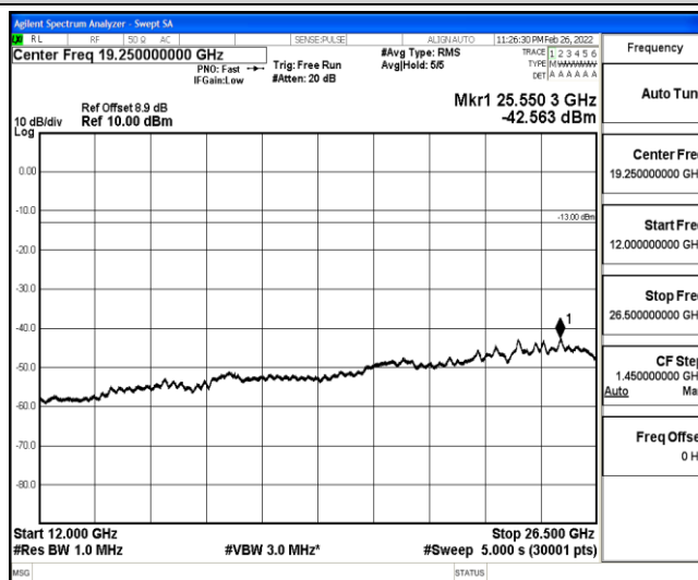
Band25-10MHz-QPSK-26090-1-0-Low-12000-26500--42.56-PASS
