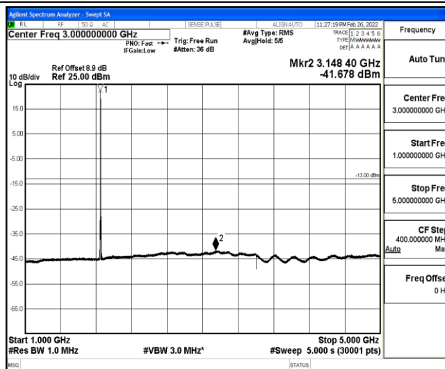
Band25-10MHz-16QAM-26090-1-0-Low-1000-5000--41.68-PASS
