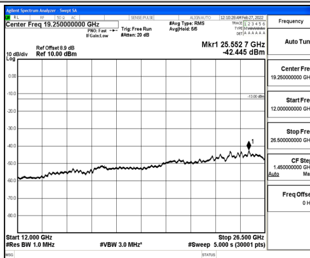
Band25-15MHz-QPSK-26615-1-0-High-12000-26500--42.45-PASS
