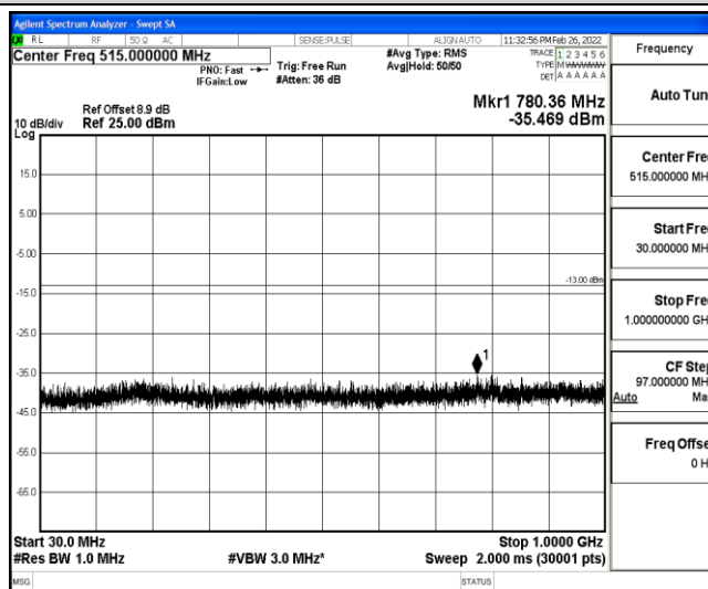
Band25-10MHz-QPSK-26640-1-0-High-30-1000--35.47-PASS
