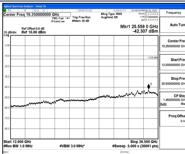
Band25-5MHz-QPSK-26665-1-0-High-12000-26500--42.31-PASS
