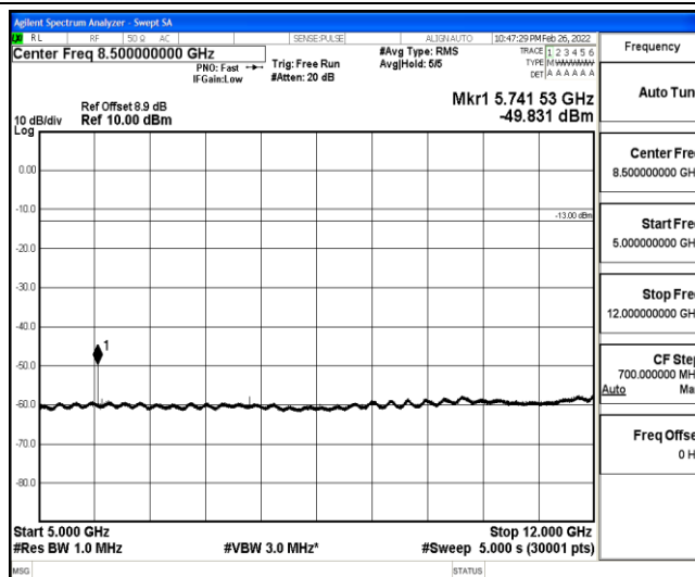
Band25-5MHz-QPSK-26665-1-0-High-5000-12000--49.83-PASS
