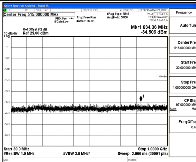
Band25-15MHz-QPSK-26615-1-0-High-30-1000--34.51-PASS
