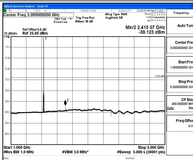
Band25-15MHz-QPSK-26115-1-0-Low-1000-5000--39.12-PASS
