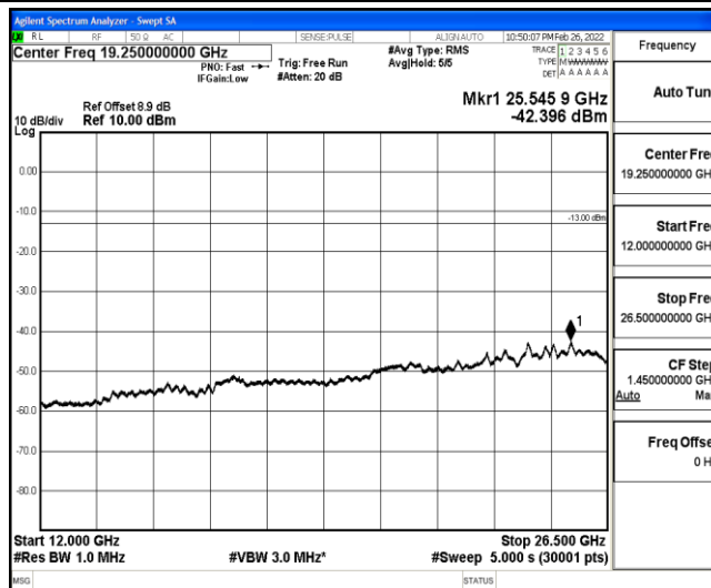
Band25-5MHz-16QAM-26665-1-0-High-12000-26500--42.4-PASS
