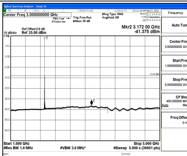
Band25-15MHz-16QAM-26615-1-0-High-1000-5000--41.38-PASS
