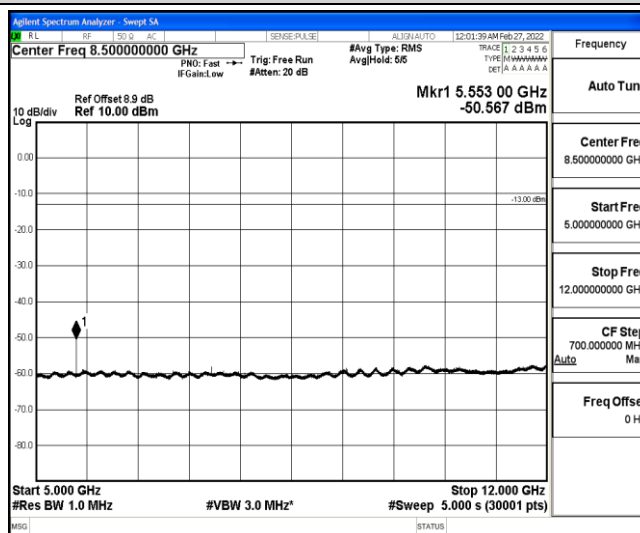
Band25-15MHz-QPSK-26115-1-0-Low-5000-12000--50.57-PASS
