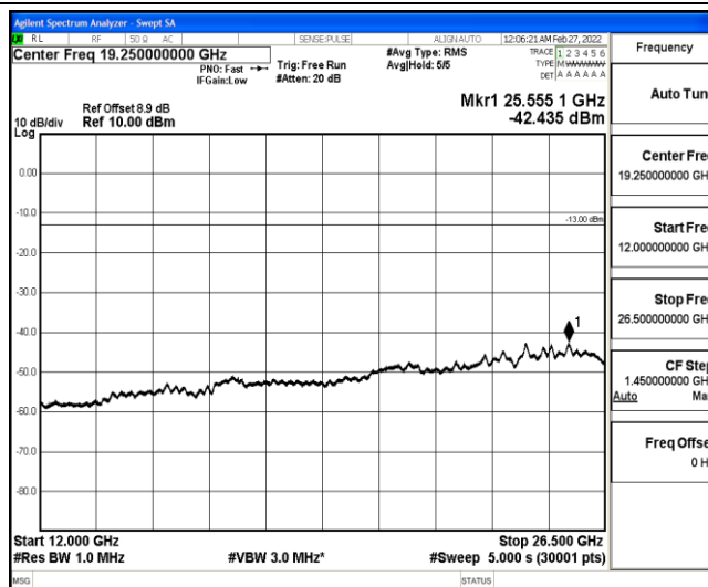
Band25-15MHz-QPSK-26365-1-0-Low-12000-26500--42.44-PASS
