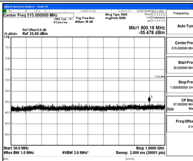
Band25-15MHz-QPSK-26115-1-0-Low-30-1000--35.48-PASS
