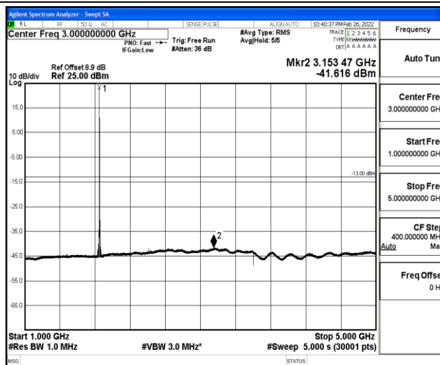
Band25-5MHz-16QAM-26065-1-0-Low-1000-5000--41.62-PASS
