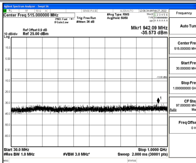
Band25-15MHz-16QAM-26365-1-0-Low-30-1000--35.57-PASS
