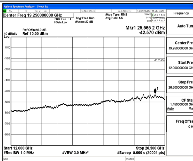
Band25-10MHz-QPSK-26640-1-0-High-12000-26500--42.57-PASS
