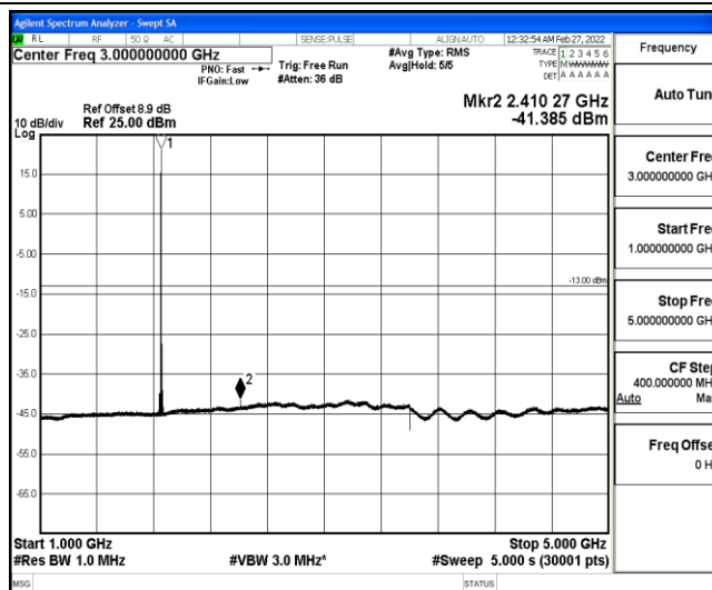
Band25-20MHz-QPSK-26140-1-0-Low-1000-5000--41.39-PASS
