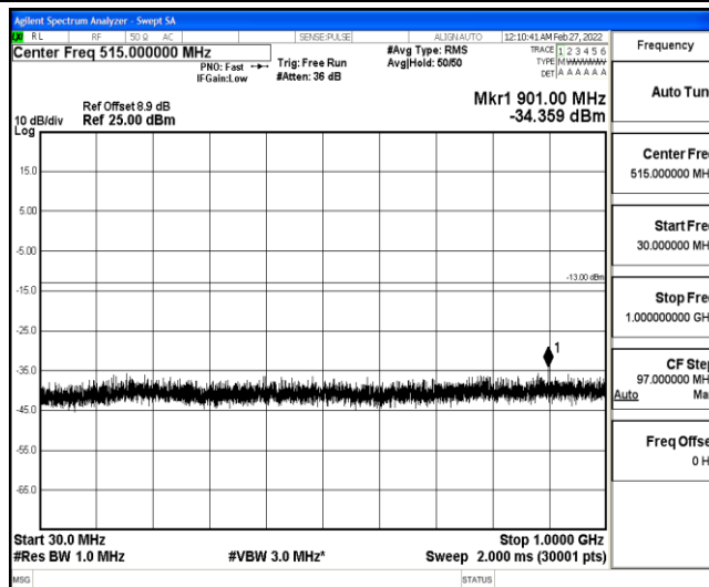
Band25-15MHz-16QAM-26615-1-0-High-30-1000--34.36-PASS
