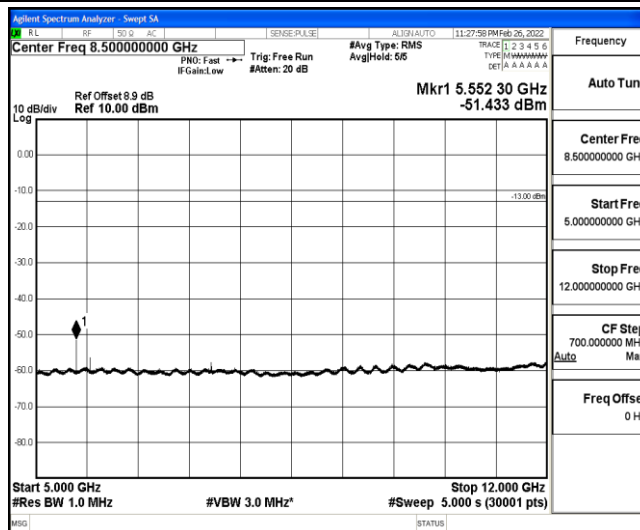
Band25-10MHz-16QAM-26090-1-0-Low-5000-12000--51.43-PASS
