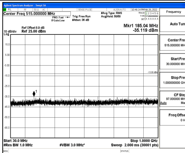
Band25-5MHz-QPSK-26665-1-0-High-30-1000--35.12-PASS
