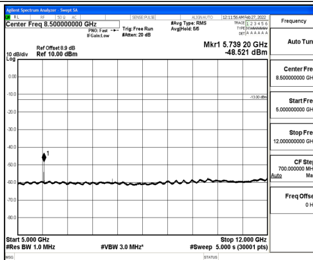
Band25-15MHz-16QAM-26615-1-0-High-5000-12000--48.52-PASS
