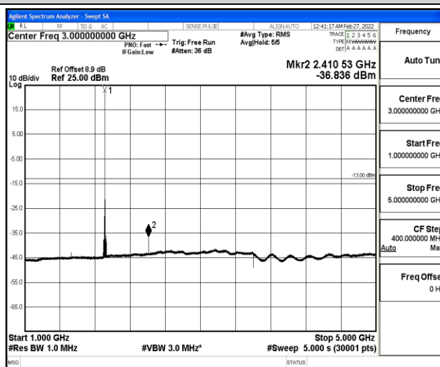
Band25-20MHz-QPSK-26590-1-0-High-1000-5000--36.84-PASS
