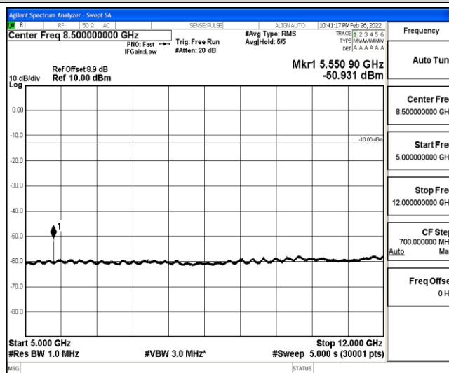
Band25-5MHz-16QAM-26065-1-0-Low-5000-12000--50.93-PASS
