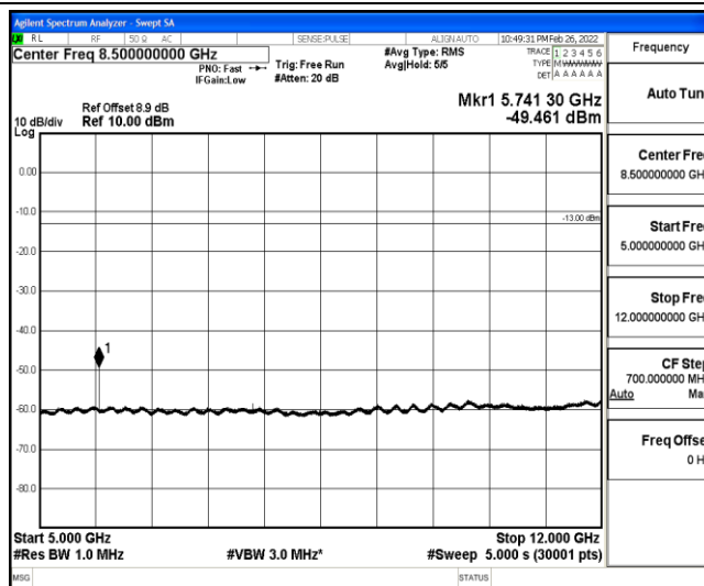
Band25-5MHz-16QAM-26665-1-0-High-5000-12000--49.46-PASS
