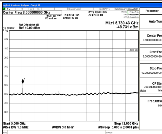
Band25-15MHz-QPSK-26615-1-0-High-5000-12000--48.73-PASS
