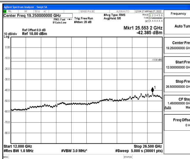
Band25-15MHz-16QAM-26115-1-0-Low-12000-26500--42.39-PASS
