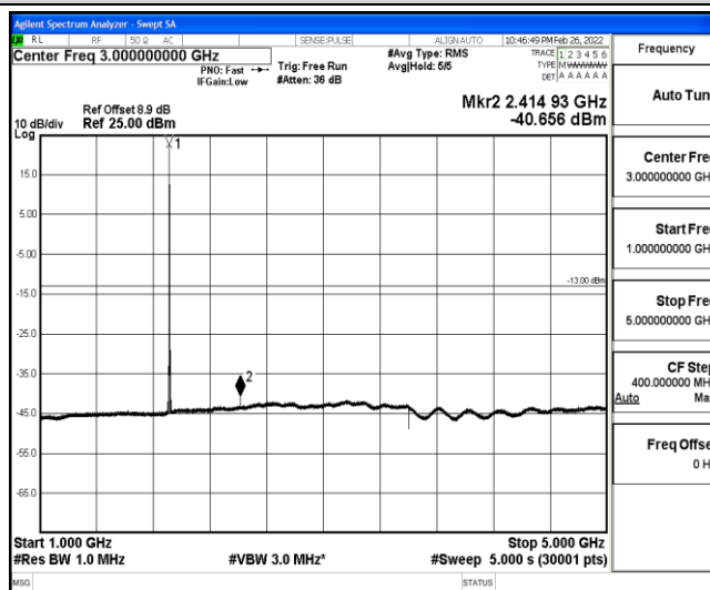
Band25-5MHz-QPSK-26665-1-0-High-1000-5000--40.66-PASS
