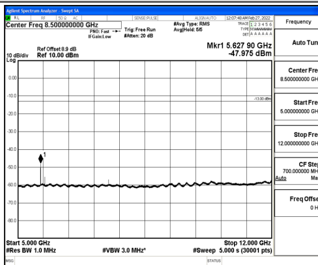
Band25-15MHz-16QAM-26365-1-0-Low-5000-12000--47.98-PASS
