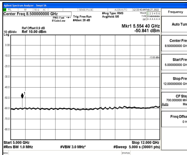
Band25-20MHz-QPSK-26140-1-0-Low-5000-12000--50.84-PASS
