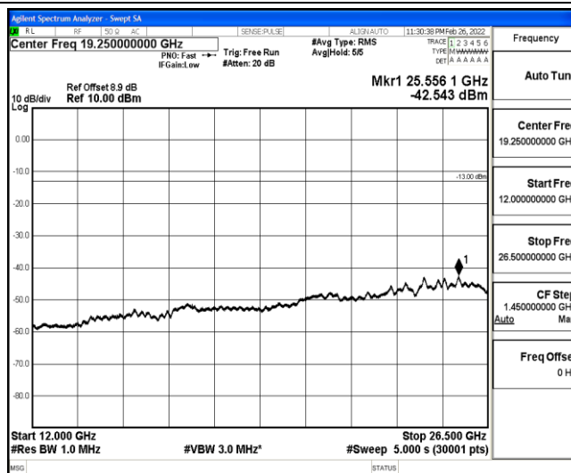
Band25-10MHz-QPSK-26365-1-0-Low-12000-26500--42.54-PASS
