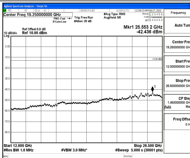
Band25-15MHz-16QAM-26365-1-0-Low-12000-26500--42.44-PASS
