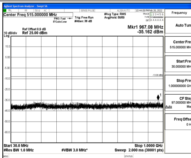
Band25-5MHz-16QAM-26365-1-0-Low-30-1000--35.16-PASS
