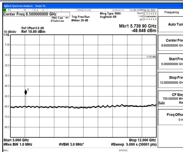
Band25-10MHz-16QAM-26640-1-0-High-5000-12000--48.65-PASS
