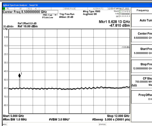
Band25-15MHz-QPSK-26365-1-0-Low-5000-12000--47.81-PASS
