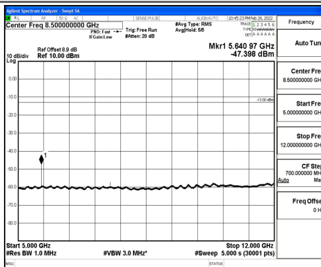
Band25-5MHz-16QAM-26365-1-0-Low-5000-12000--47.4-PASS
