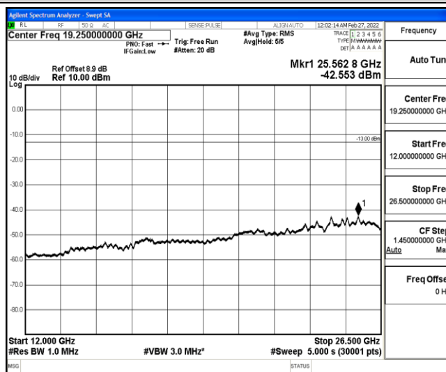
Band25-15MHz-QPSK-26115-1-0-Low-12000-26500--42.55-PASS
