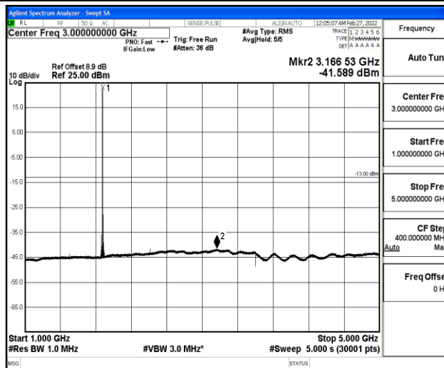
Band25-15MHz-QPSK-26365-1-0-Low-1000-5000--41.59-PASS
