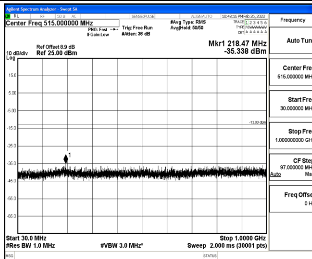
Band25-5MHz-16QAM-26665-1-0-High-30-1000--35.34-PASS
