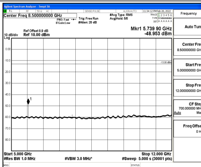
Band25-10MHz-QPSK-26640-1-0-High-5000-12000--48.95-PASS
