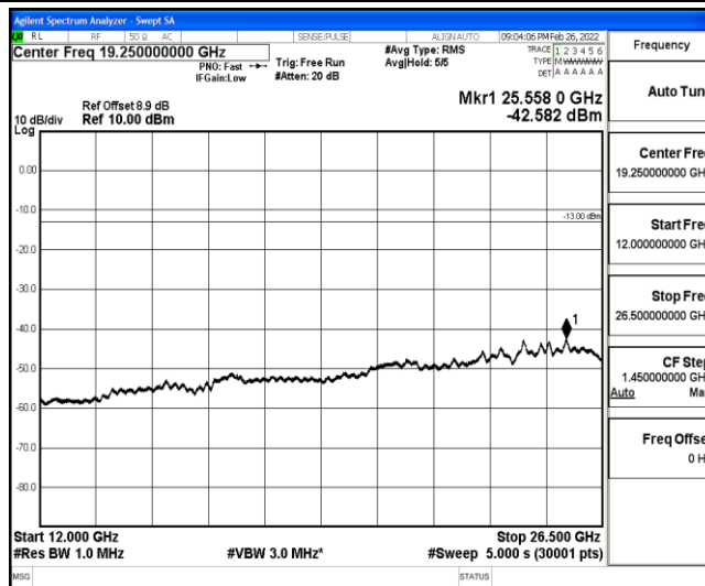
Band25-1.4MHz-QPSK-26683-1-0-High-12000-26500--42.58-PASS
