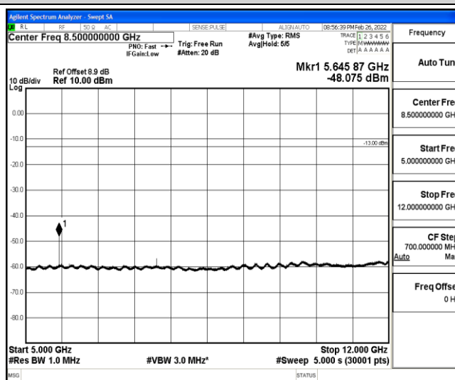
Band25-1.4MHz-QPSK-26365-1-0-Low-5000-12000--48.08-PASS
