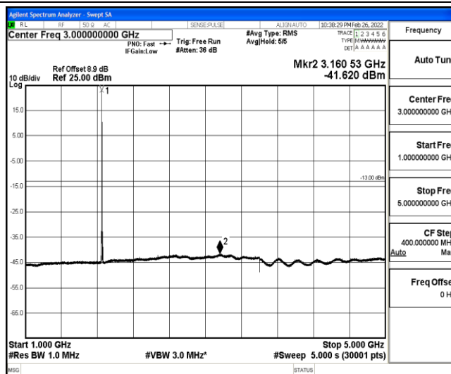
Band25-5MHz-QPSK-26065-1-0-Low-1000-5000--41.62-PASS
