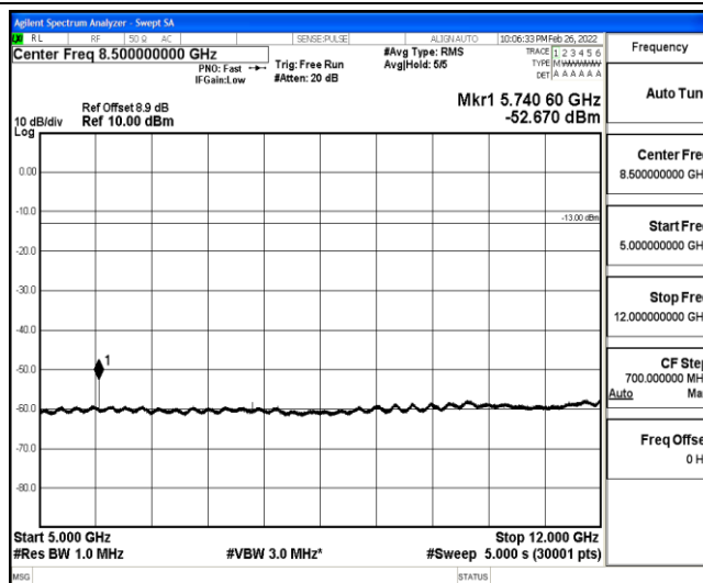
Band25-3MHz-QPSK-26675-1-0-High-5000-12000--52.67-PASS
