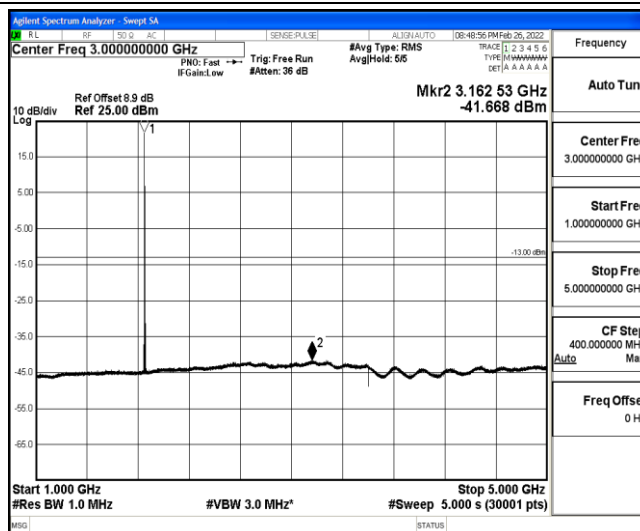
Band25-1.4MHz-16QAM-26047-1-0-Low-1000-5000--41.67-PASS
