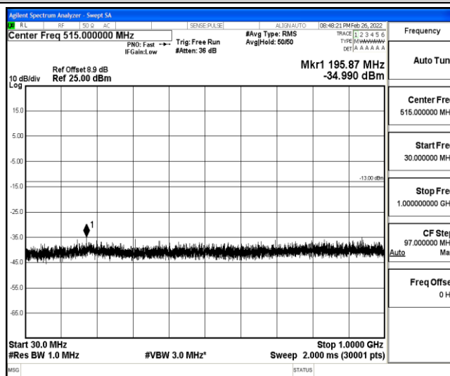
Band25-1.4MHz-16QAM-26047-1-0-Low-30-1000--34.99-PASS
