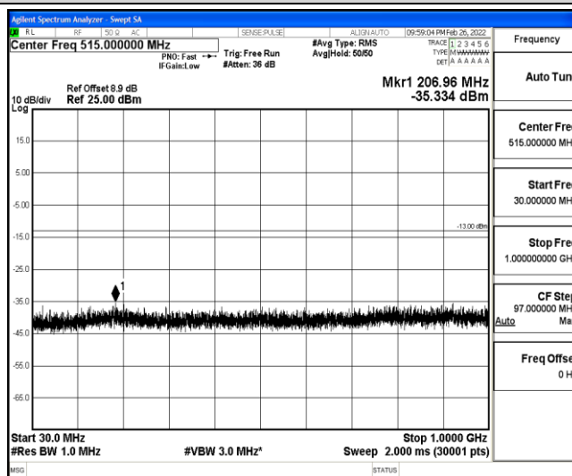
Band25-3MHz-16QAM-26055-1-0-Low-30-1000--35.33-PASS
