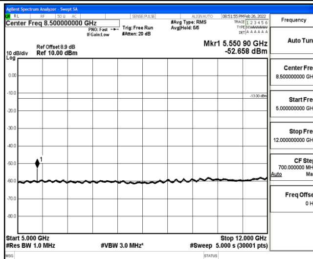
Band25-1.4MHz-16QAM-26047-1-0-Low-5000-12000--52.66-PASS
