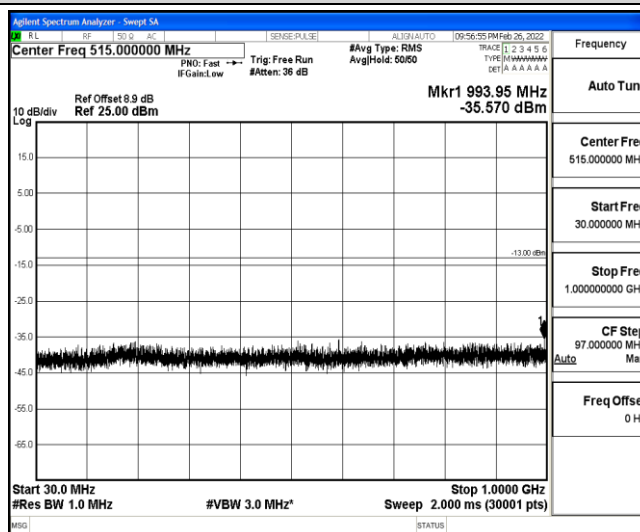
Band25-3MHz-QPSK-26055-1-0-Low-30-1000--35.57-PASS
