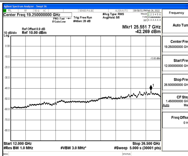
Band25-3MHz-QPSK-26055-1-0-Low-12000-26500--42.27-PASS
