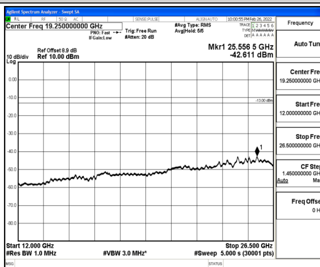
Band25-3MHz-16QAM-26055-1-0-Low-12000-26500--42.61-PASS
