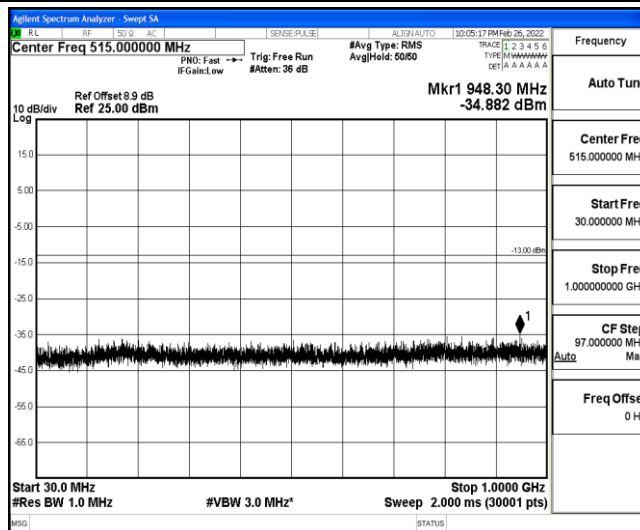
Band25-3MHz-QPSK-26675-1-0-High-30-1000--34.88-PASS
