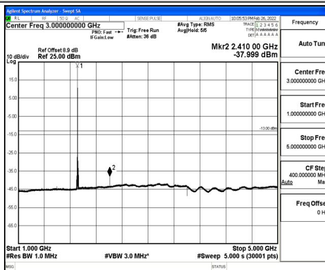
Band25-3MHz-QPSK-26675-1-0-High-1000-5000--38-PASS
