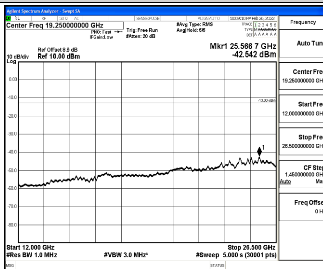
Band25-3MHz-16QAM-26675-1-0-High-12000-26500--42.54-PASS
