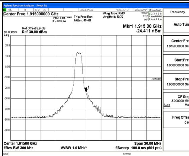
Band25-15MHz-16QAM-26615-6-0-High--24.41-PASS
