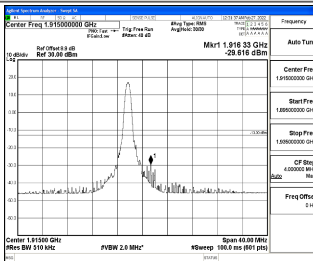
Band25-20MHz-QPSK-26590-1-0-High--29.62-PASS
