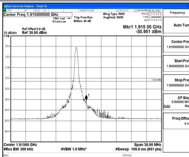
Band25-15MHz-16QAM-26615-1-0-High--30.95-PASS
