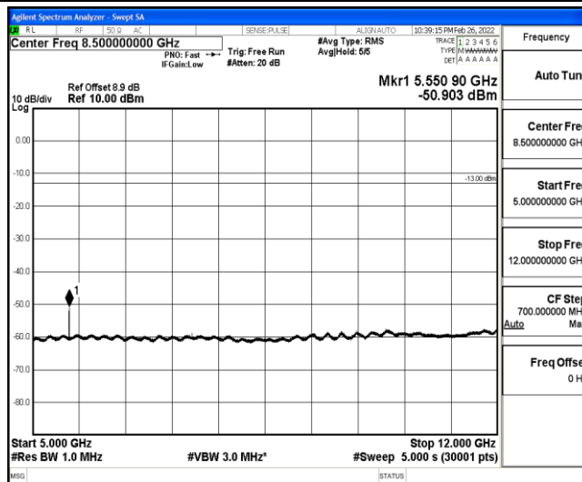
Band25-5MHz-QPSK-26065-1-0-Low-5000-12000--50.9-PASS
