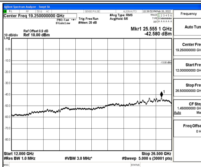
Band25-5MHz-QPSK-26065-1-0-Low-12000-26500--42.58-PASS
