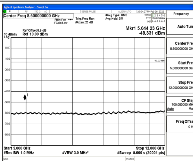
Band25-3MHz-16QAM-26365-1-0-Low-5000-12000--48.33-PASS
