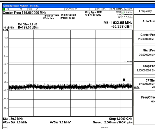
Band25-5MHz-QPSK-26065-1-0-Low-30-1000--35.27-PASS
