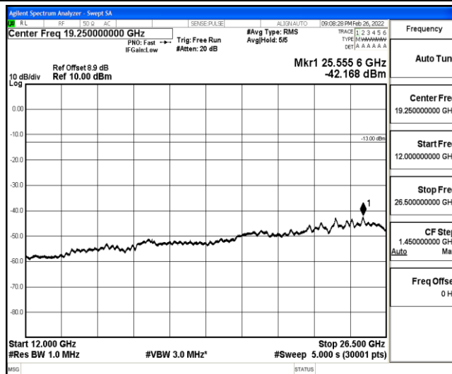
Band25-1.4MHz-16QAM-26683-1-0-High-12000-26500--42.17-PASS
