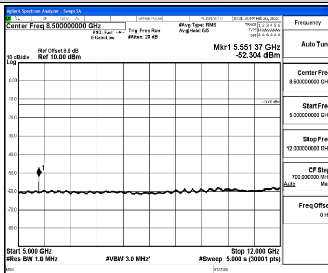
Band25-3MHz-16QAM-26055-1-0-Low-5000-12000--52.3-PASS
