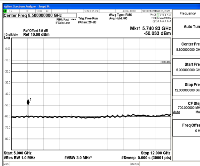
Band25-3MHz-16QAM-26675-1-0-High-5000-12000--50.03-PASS
