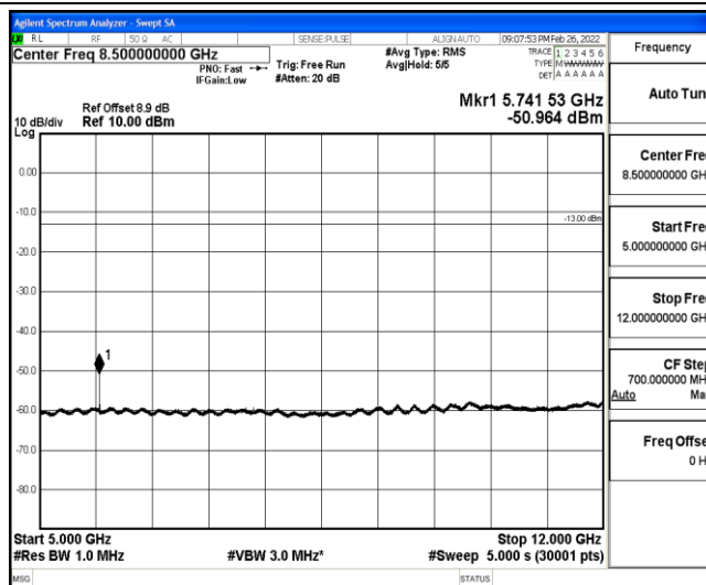
Band25-1.4MHz-16QAM-26683-1-0-High-5000-12000--50.96-PASS
