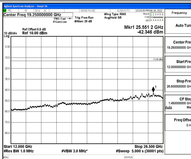
Band25-3MHz-QPSK-26365-1-0-Low-12000-26500--42.35-PASS
