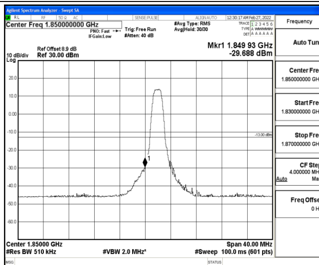
Band25-20MHz-QPSK-26140-6-0-Low--29.69-PASS
