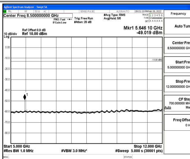
Band25-1.4MHz-16QAM-26365-1-0-Low-5000-12000--49.02-PASS
