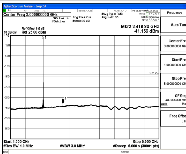
Band25-1.4MHz-QPSK-26365-1-0-Low-1000-5000--41.16-PASS
