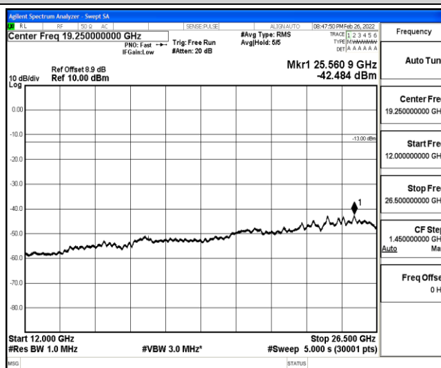
Band25-1.4MHz-QPSK-26047-1-0-Low-12000-26500--42.48-PASS
