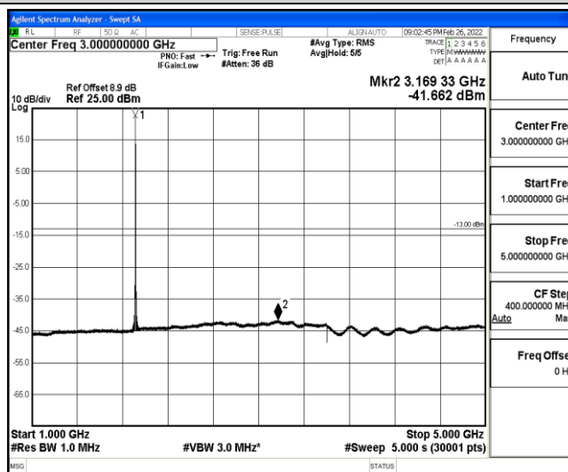
Band25-1.4MHz-QPSK-26683-1-0-High-1000-5000--41.66-PASS
