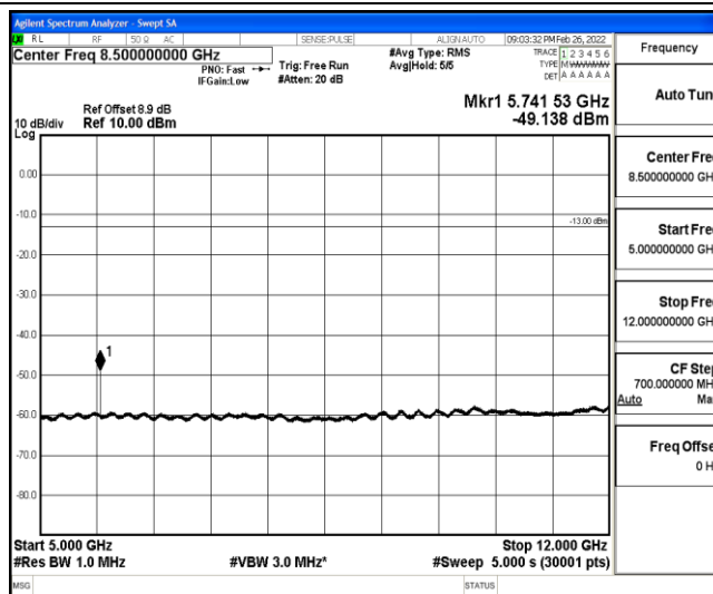
Band25-1.4MHz-QPSK-26683-1-0-High-5000-12000--49.14-PASS
