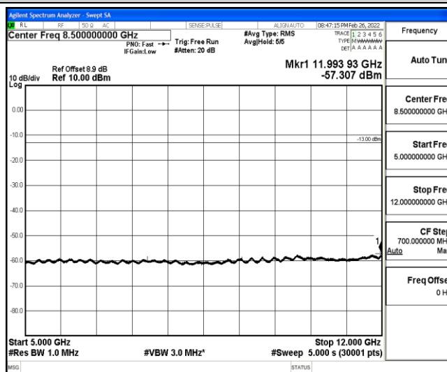
Band25-1.4MHz-QPSK-26047-1-0-Low-5000-12000--57.31-PASS
