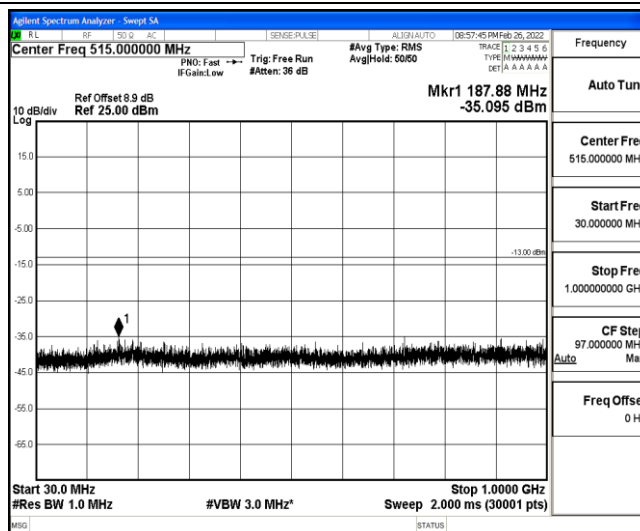
Band25-1.4MHz-16QAM-26365-1-0-Low-30-1000--35.1-PASS
