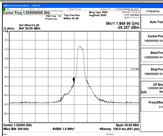
Band25-15MHz-QPSK-26115-6-0-Low--25.26-PASS
