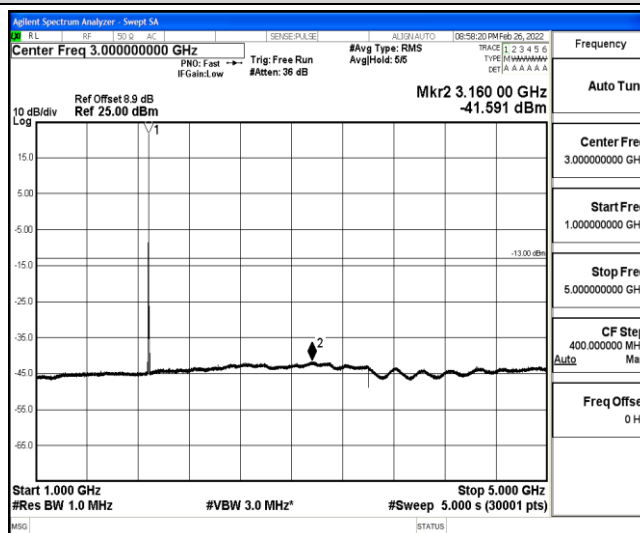
Band25-1.4MHz-16QAM-26365-1-0-Low-1000-5000--41.59-PASS
