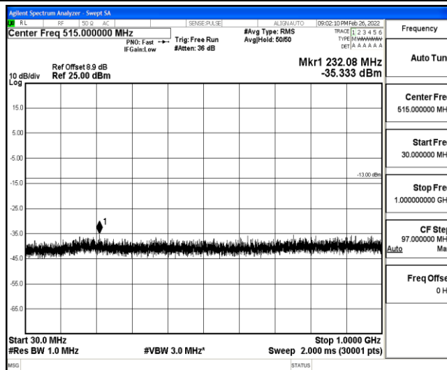
Band25-1.4MHz-QPSK-26683-1-0-High-30-1000--35.33-PASS
