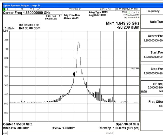
Band25-15MHz-16QAM-26115-1-0-Low--20.21-PASS
