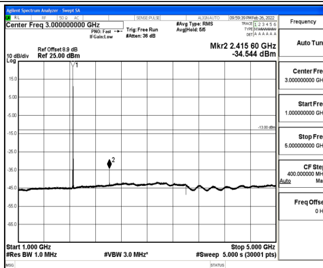
Band25-3MHz-16QAM-26055-1-0-Low-1000-5000--34.54-PASS
