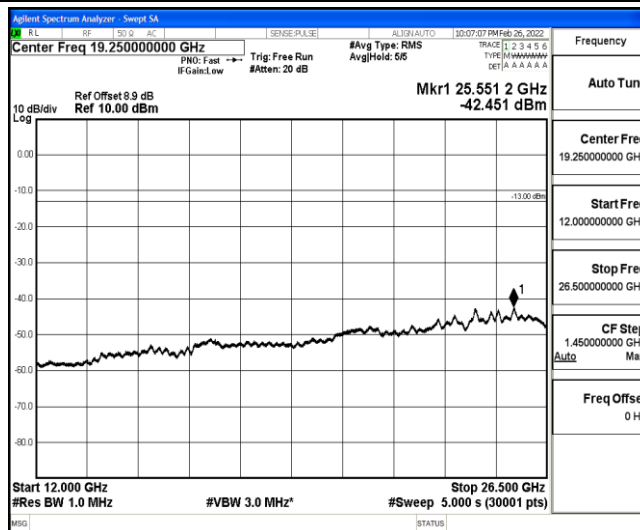
Band25-3MHz-QPSK-26675-1-0-High-12000-26500--42.45-PASS
