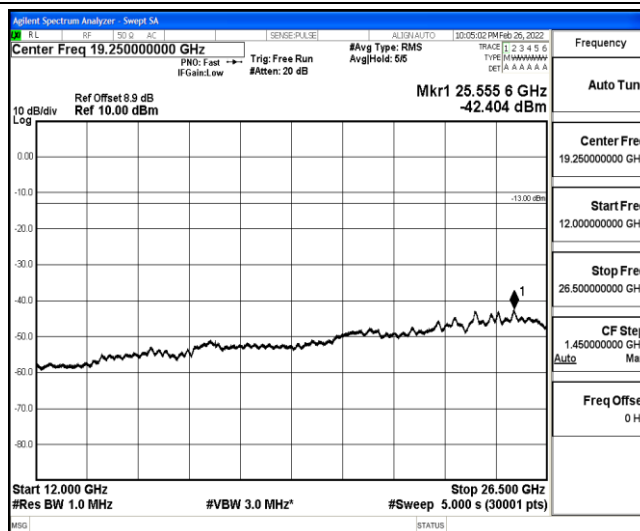
Band25-3MHz-16QAM-26365-1-0-Low-12000-26500--42.4-PASS
