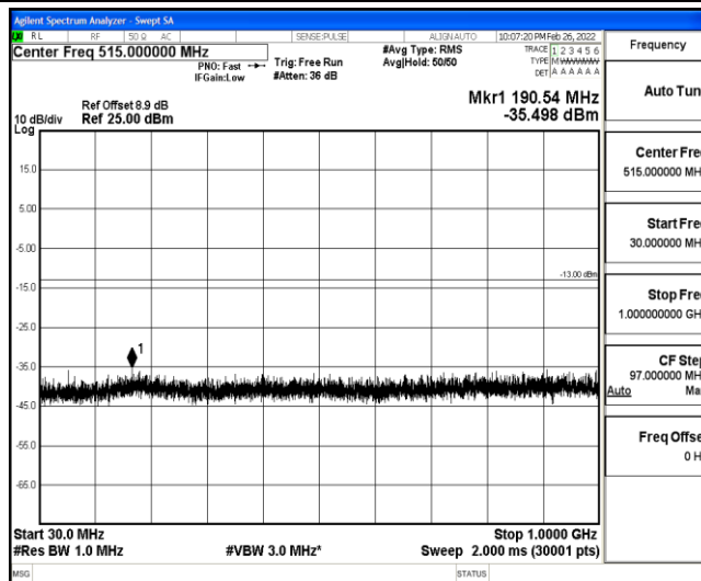
Band25-3MHz-16QAM-26675-1-0-High-30-1000--35.5-PASS
