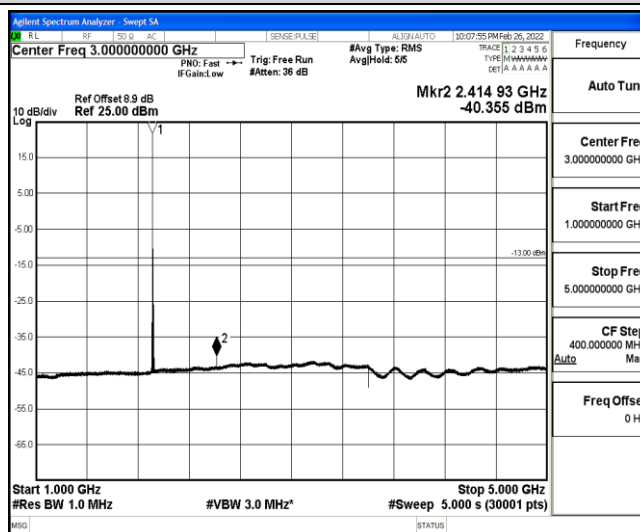
Band25-3MHz-16QAM-26675-1-0-High-1000-5000--40.36-PASS
