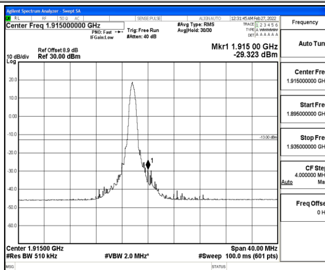
Band25-20MHz-16QAM-26590-1-0-High--29.32-PASS
