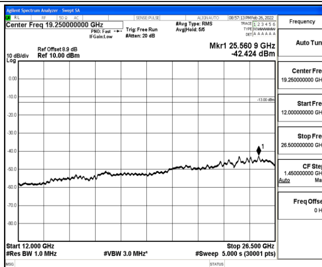
Band25-1.4MHz-QPSK-26365-1-0-Low-12000-26500--42.42-PASS
