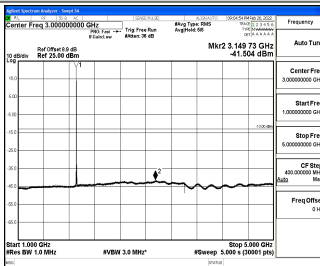
Band25-1.4MHz-16QAM-26683-1-0-High-1000-5000--41.5-PASS
