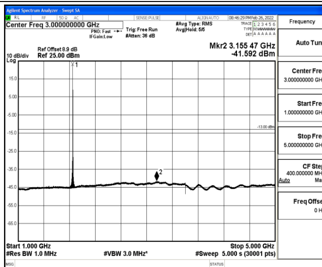
Band25-1.4MHz-QPSK-26047-1-0-Low-1000-5000--41.59-PASS
