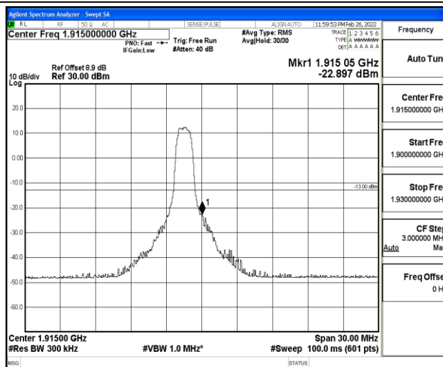
Band25-15MHz-QPSK-26615-6-0-High--22.90-PASS
