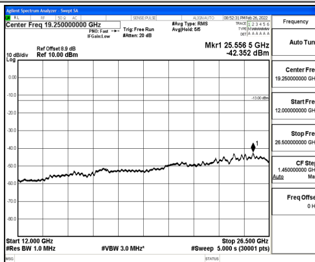
Band25-1.4MHz-16QAM-26047-1-0-Low-12000-26500--42.35-PASS
