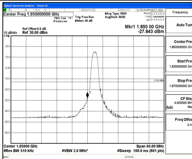
Band25-20MHz-16QAM-26140-6-0-Low--27.84-PASS
