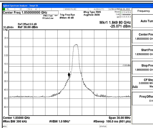
Band25-15MHz-16QAM-26115-6-0-Low--25.07-PASS
