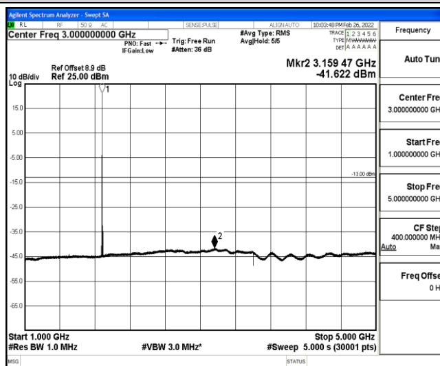
Band25-3MHz-16QAM-26365-1-0-Low-1000-5000--41.62-PASS
