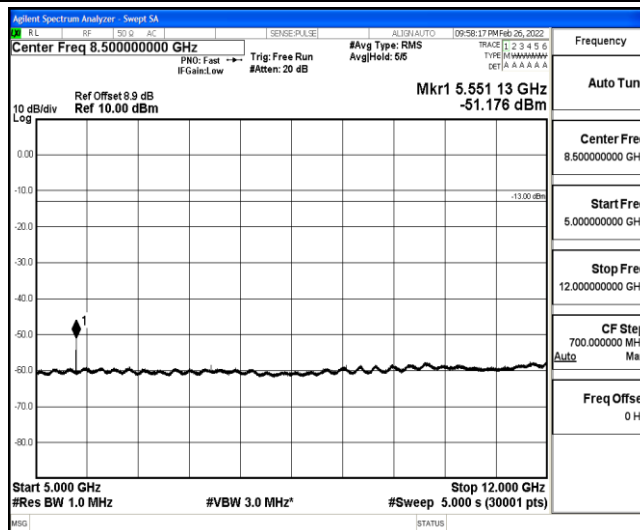
Band25-3MHz-QPSK-26055-1-0-Low-5000-12000--51.18-PASS
