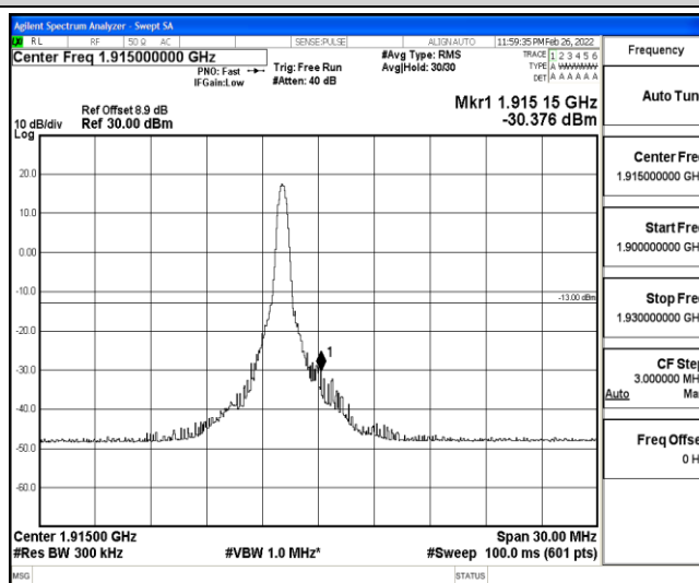
Band25-15MHz-QPSK-26615-1-0-High--30.38-PASS
