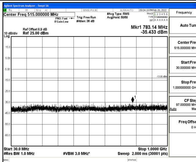
Band25-1.4MHz-16QAM-26683-1-0-High-30-1000--35.43-PASS
