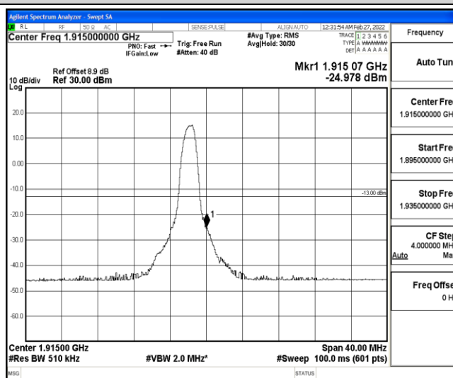
Band25-20MHz-QPSK-26590-6-0-High--24.98-PASS
