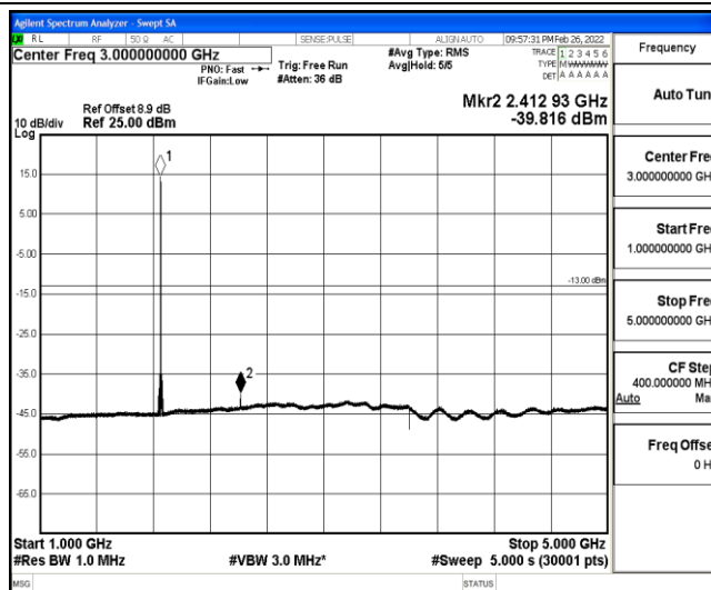
Band25-3MHz-QPSK-26055-1-0-Low-1000-5000--39.82-PASS
