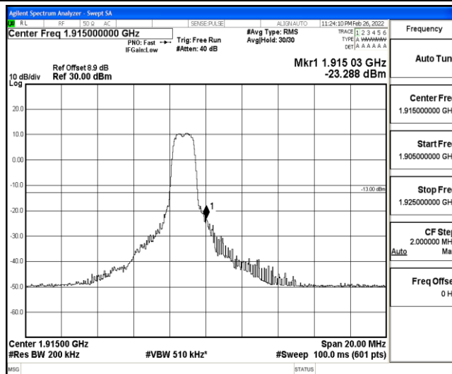
Band25-10MHz-QPSK-26640-6-0-High--23.29-PASS
