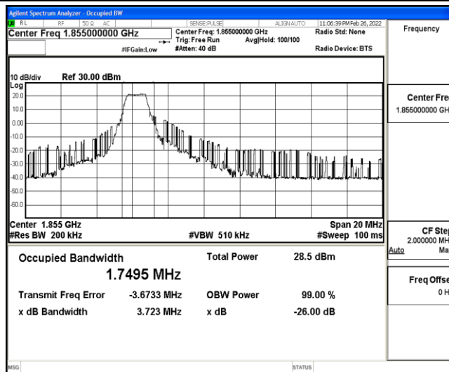
Band25-10MHz-16QAM-26090-6-0-Low-1.7495-3.723-PASS
