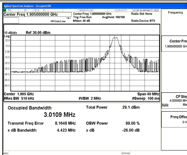
Band25-20MHz-QPSK-26590-6-0-High-3.0109-4.423-PASS
