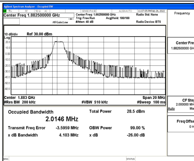
Band25-10MHz-QPSK-26365-6-0-Low-2.0146-4.103-PASS
