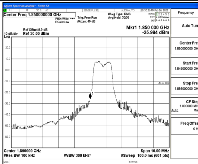
Band25-5MHz-16QAM-26065-6-0-Low--25.98-PASS
