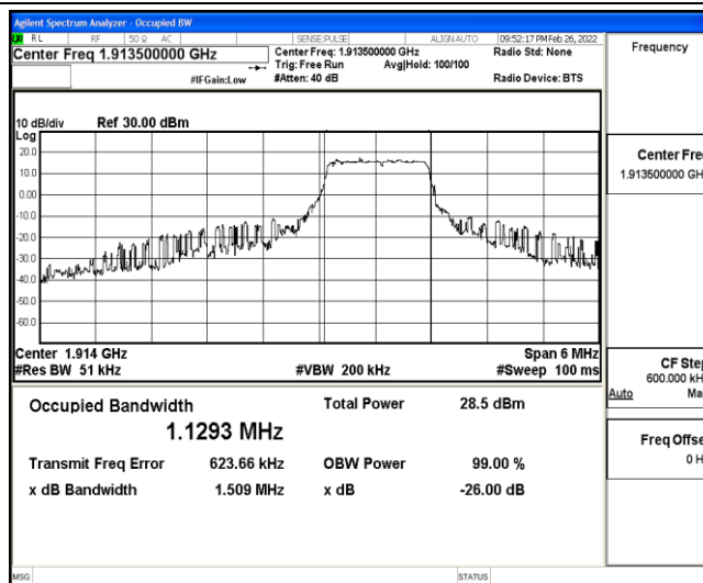
Band25-3MHz-16QAM-26675-6-0-High-1.1293-1.509-PASS
