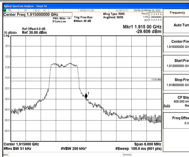
Band25-3MHz-QPSK-26675-6-0-High--29.61-PASS
