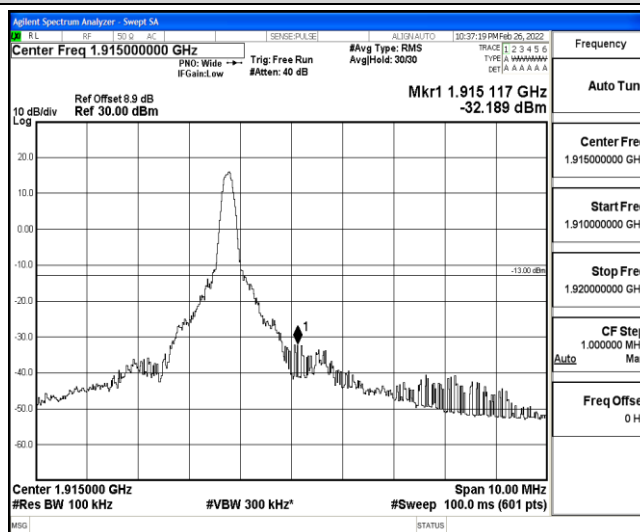
Band25-5MHz-16QAM-26665-1-0-High--32.19-PASS
