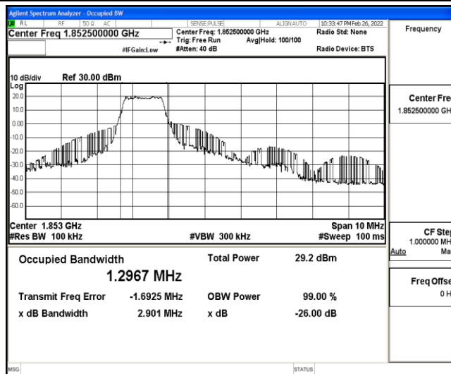
Band25-5MHz-16QAM-26065-6-0-Low-1.2967-2.901-PASS
