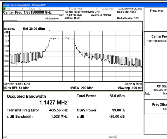
Band25-3MHz-16QAM-26055-6-0-Low-1.1427-1.528-PASS
