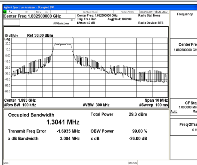
Band25-5MHz-QPSK-26365-6-0-Low-1.3041-3.004-PASS
