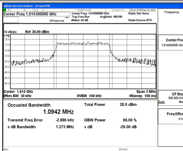
Band25-1.4MHz-QPSK-26683-6-0-High-1.0942-1.273-PASS
