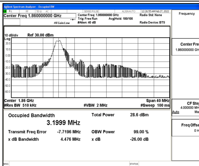
Band25-20MHz-QPSK-26140-6-0-Low-3.1999-4.476-PASS
