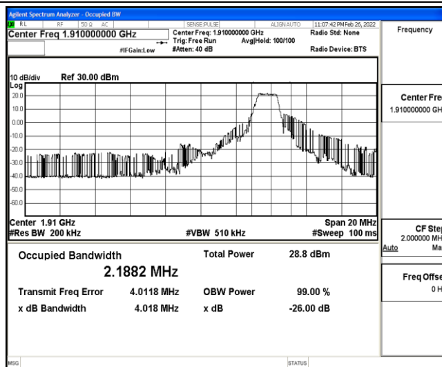
Band25-10MHz-QPSK-26640-6-0-High-2.1882-4.018-PASS
