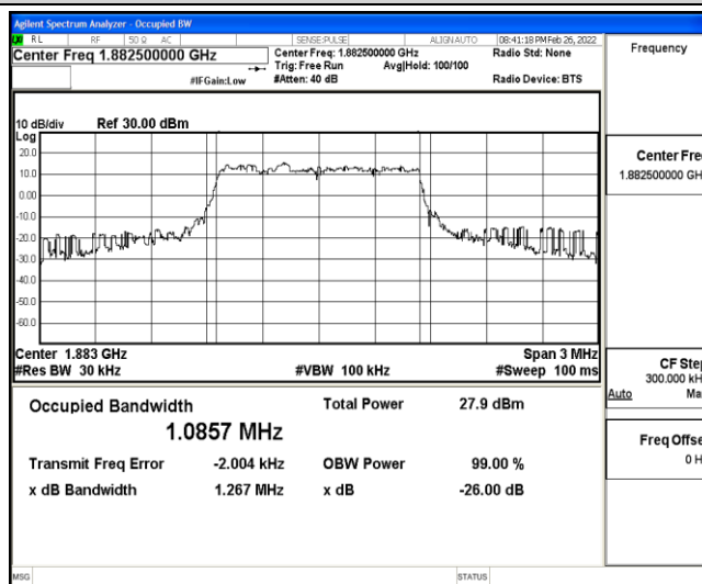
Band25-1.4MHz-16QAM-26365-6-0-Low-1.0857-1.267-PASS
