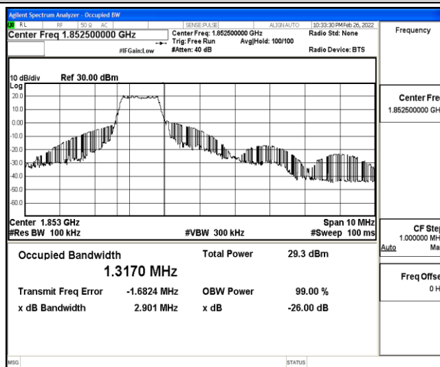
Band25-5MHz-QPSK-26065-6-0-Low-1.3170-2.901-PASS
