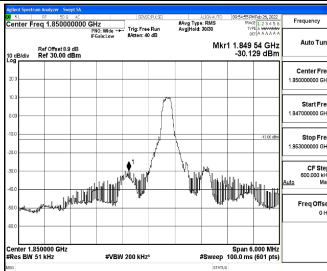
Band25-3MHz-16QAM-26055-1-0-Low--30.13-PASS
