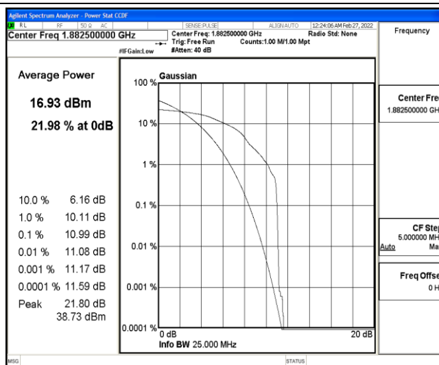
Band25-20MHz-16QAM-26365-1-0-Low-10.99-<=13-PASS
