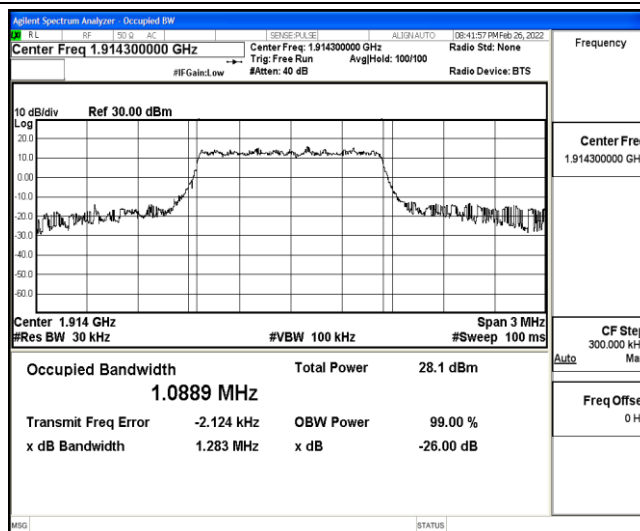
Band25-1.4MHz-16QAM-26683-6-0-High-1.0889-1.283-PASS
