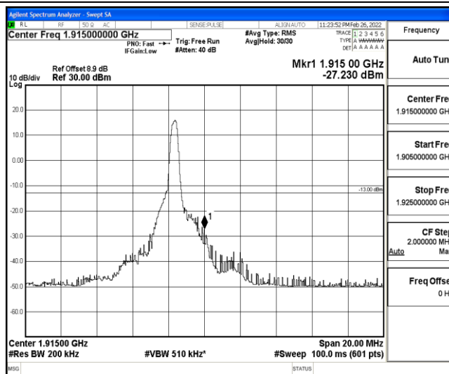
Band25-10MHz-QPSK-26640-1-0-High--27.23-PASS
