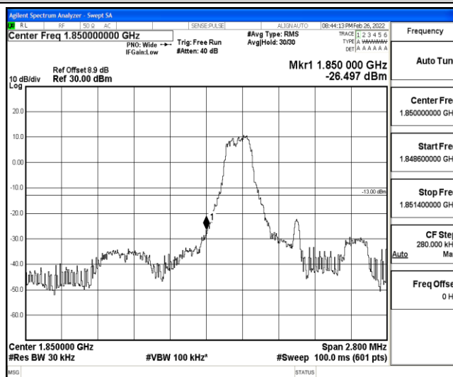
Band25-1.4MHz-16QAM-26047-1-0-Low--26.50-PASS
