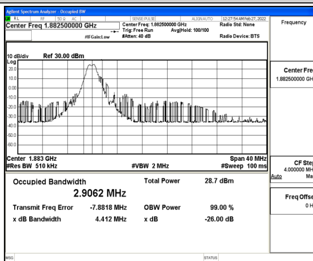
Band25-20MHz-16QAM-26365-6-0-Low-2.9062-4.412-PASS
