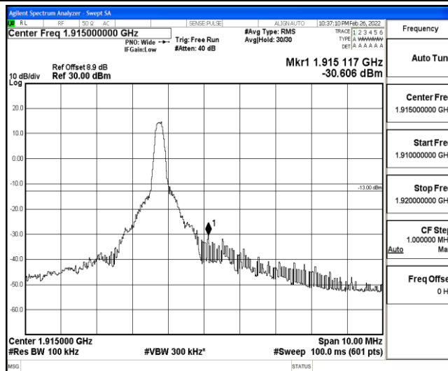
Band25-5MHz-QPSK-26665-1-0-High--30.61-PASS
