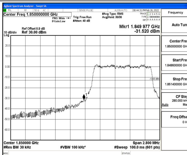
Band25-1.4MHz-16QAM-26047-6-0-Low--31.52-PASS
