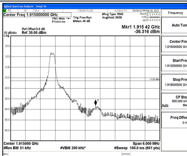
Band25-3MHz-QPSK-26675-1-0-High--36.32-PASS
