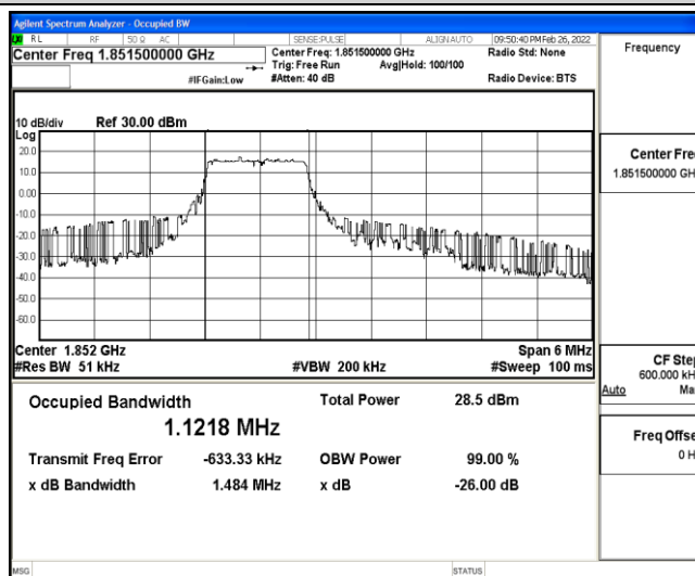
Band25-3MHz-QPSK-26055-6-0-Low-1.1218-1.484-PASS
