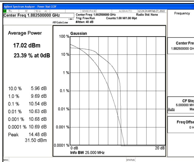
Band25-20MHz-16QAM-26365-6-0-Low-10.54-<=13-PASS
