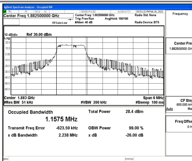
Band25-3MHz-QPSK-26365-6-0-Low-1.1575-2.238-PASS
