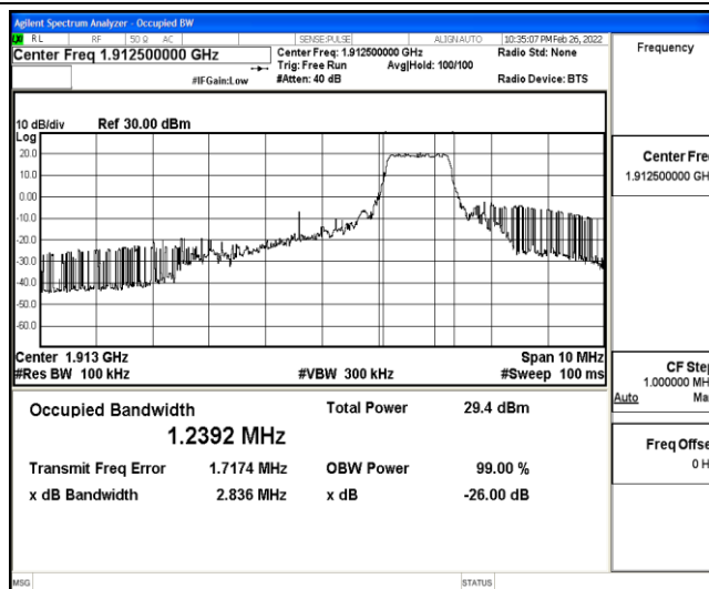
Band25-5MHz-16QAM-26665-6-0-High-1.2392-2.836-PASS
