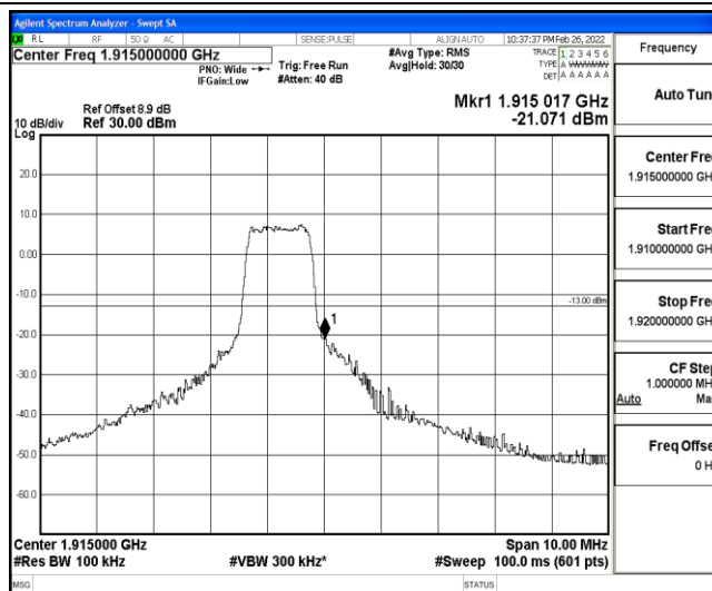
Band25-5MHz-16QAM-26665-6-0-High--21.07-PASS
