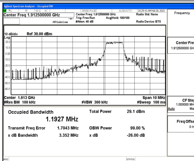
Band25-5MHz-QPSK-26665-6-0-High-1.1927-3.352-PASS
