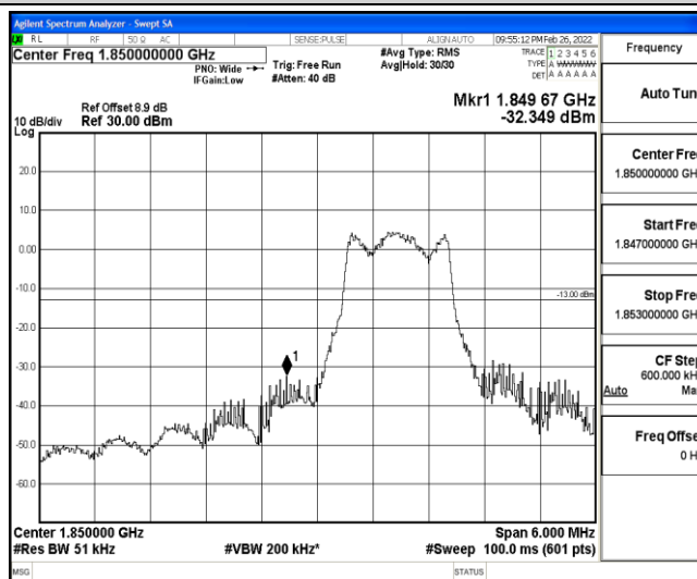
Band25-3MHz-16QAM-26055-6-0-Low--32.35-PASS
