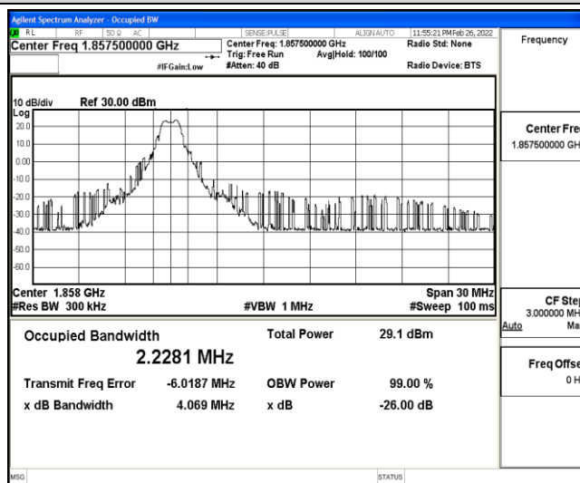
Band25-15MHz-QPSK-26115-6-0-Low-2.2281-4.069-PASS
