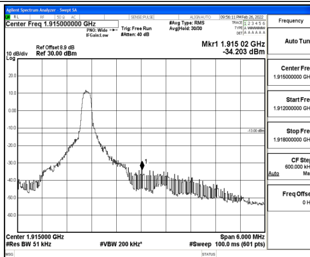
Band25-3MHz-16QAM-26675-1-0-High--34.20-PASS
