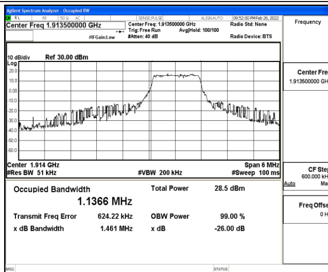
Band25-3MHz-QPSK-26675-6-0-High-1.1366-1.461-PASS
