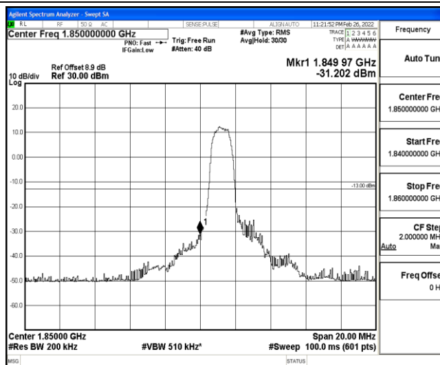
Band25-10MHz-16QAM-26090-6-0-Low--31.20-PASS
