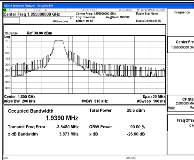
Band25-10MHz-QPSK-26090-6-0-Low-1.9390-3.873-PASS
