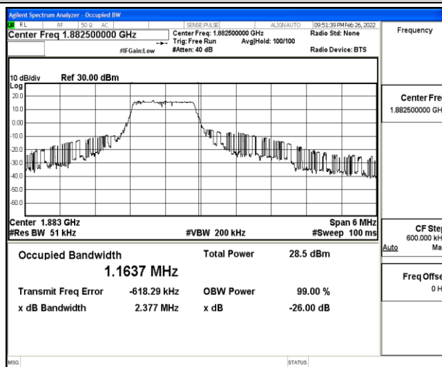
Band25-3MHz-16QAM-26365-6-0-Low-1.1637-2.377-PASS
