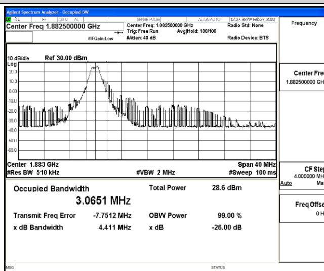
Band25-20MHz-QPSK-26365-6-0-Low-3.0651-4.411-PASS
