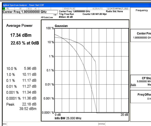
Band25-20MHz-16QAM-26590-1-0-High-11.17-<=13-PASS
