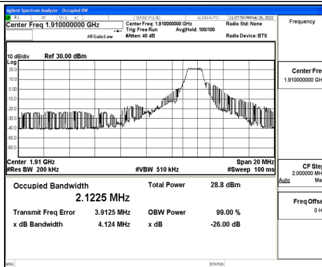
Band25-10MHz-16QAM-26640-6-0-High-2.1225-4.124-PASS
