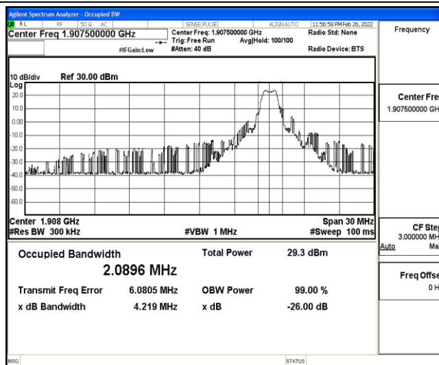
Band25-15MHz-QPSK-26615-6-0-High-2.0896-4.219-PASS
