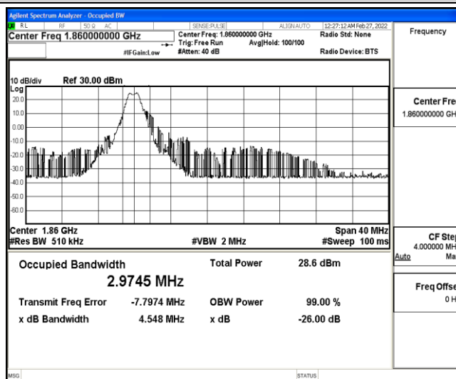
Band25-20MHz-16QAM-26140-6-0-Low-2.9745-4.548-PASS
