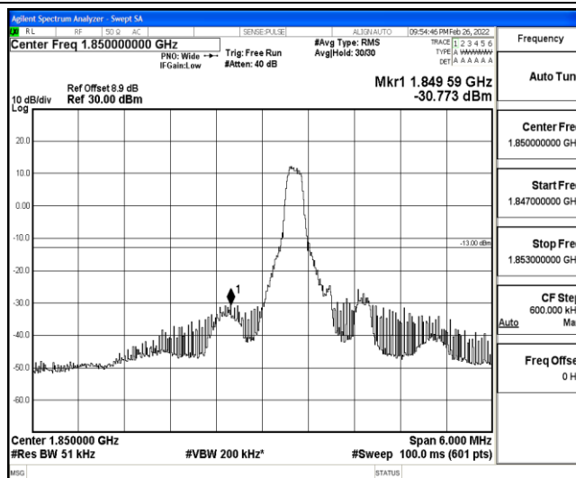
Band25-3MHz-QPSK-26055-1-0-Low--30.77-PASS
