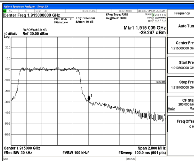
Band25-1.4MHz-16QAM-26683-6-0-High--29.27-PASS
