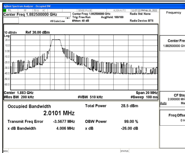
Band25-10MHz-16QAM-26365-6-0-Low-2.0101-4.006-PASS
