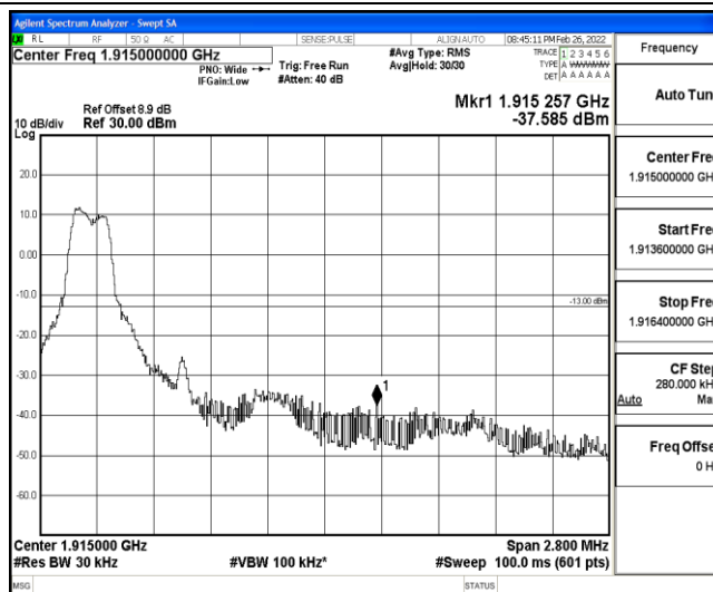
Band25-1.4MHz-QPSK-26683-1-0-High--37.58-PASS
