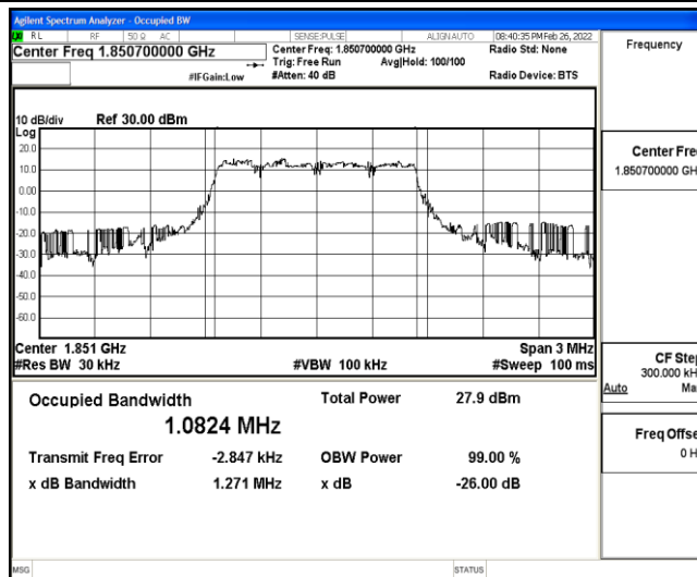
Band25-1.4MHz-16QAM-26047-6-0-Low-1.0824-1.271-PASS
