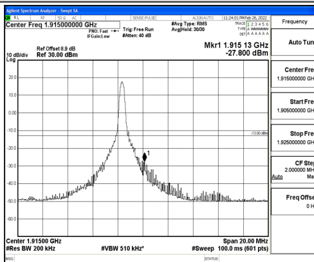
Band25-10MHz-16QAM-26640-1-0-High--27.80-PASS
