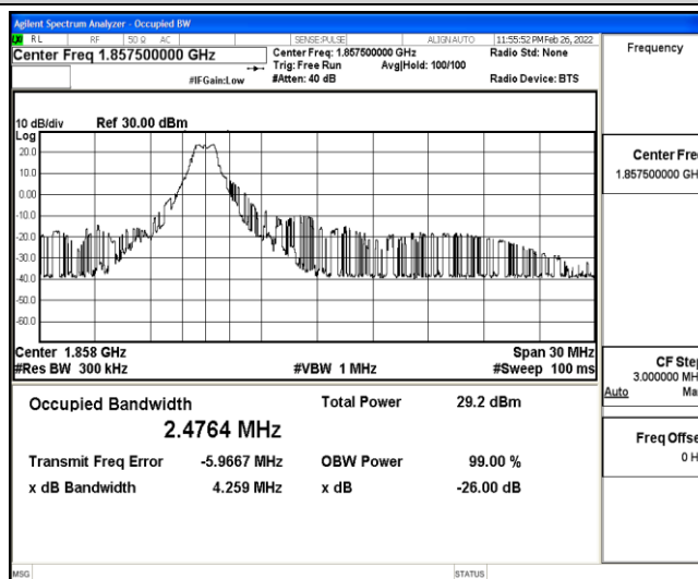
Band25-15MHz-16QAM-26115-6-0-Low-2.4764-4.259-PASS
