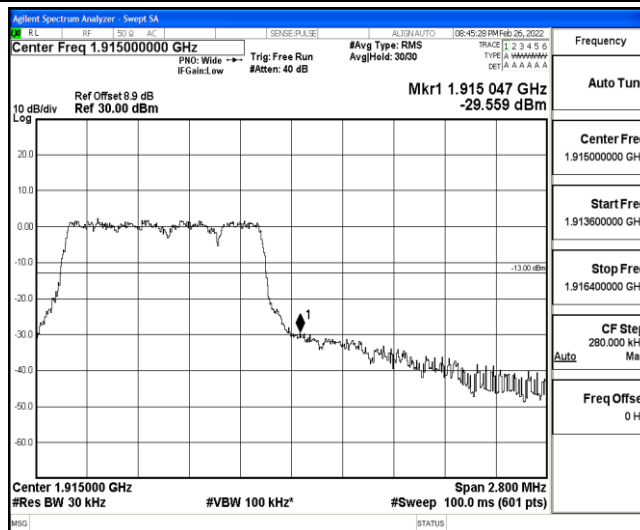
Band25-1.4MHz-QPSK-26683-6-0-High--29.56-PASS
