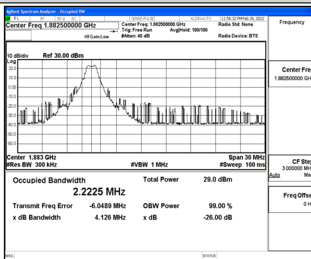
Band25-15MHz-16QAM-26365-6-0-Low-2.2225-4.126-PASS
