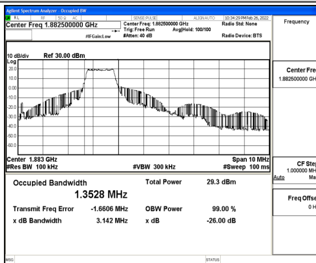
Band25-5MHz-16QAM-26365-6-0-Low-1.3528-3.142-PASS
