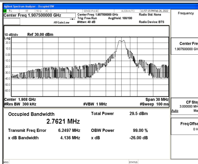
Band25-15MHz-16QAM-26615-6-0-High-2.7621-4.136-PASS
