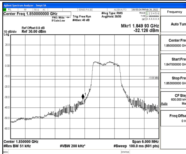
Band25-3MHz-QPSK-26055-6-0-Low--32.13-PASS
