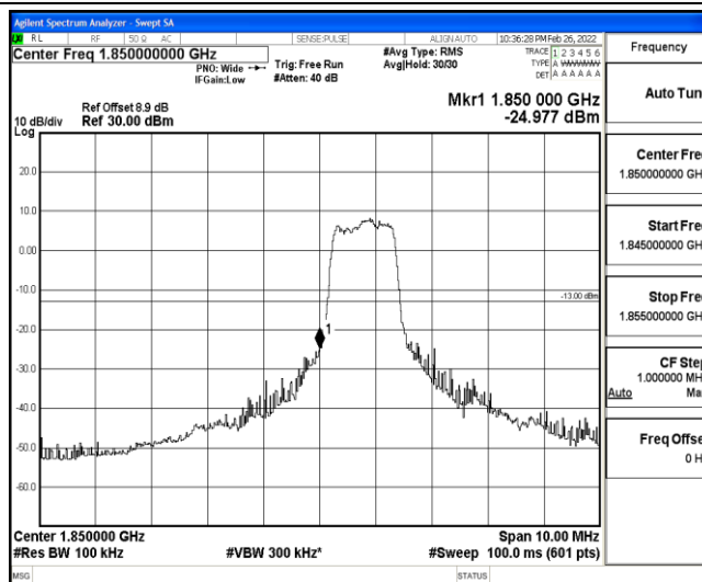
Band25-5MHz-QPSK-26065-6-0-Low--24.98-PASS
