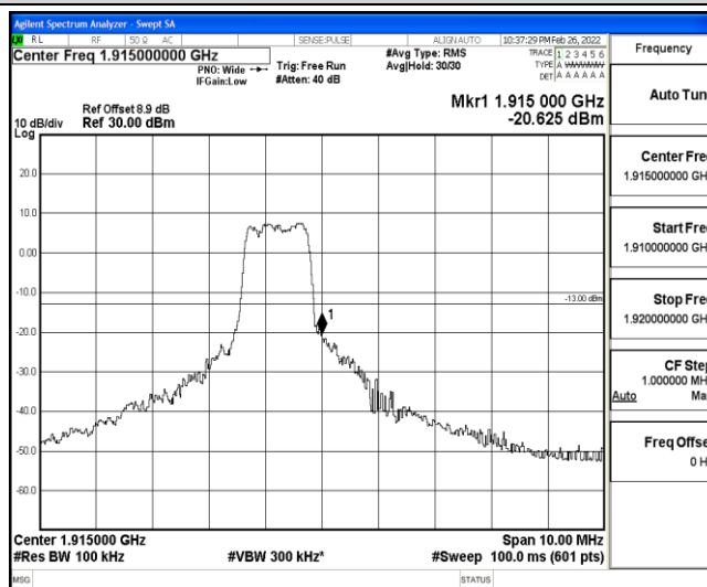
Band25-5MHz-QPSK-26665-6-0-High--20.62-PASS
