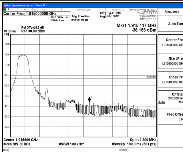
Band25-1.4MHz-16QAM-26683-1-0-High--36.16-PASS
