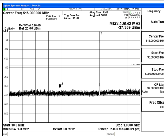
Band12-3MHz-16QAM-23025-1-0-Low-30-1000--37.36-PASS
