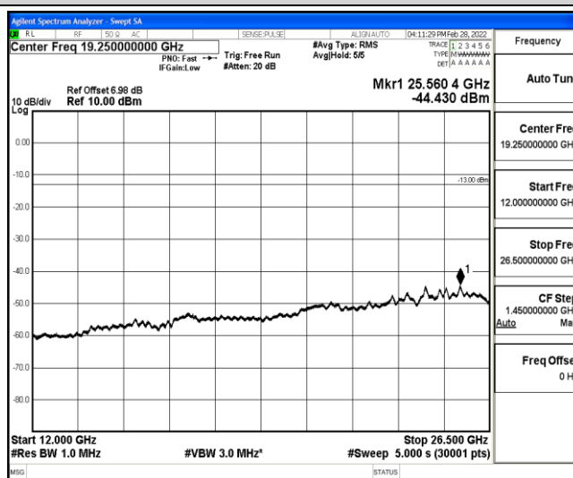
Band12-5MHz-16QAM-23035-1-0-Low-12000-26500--44.43-PASS
