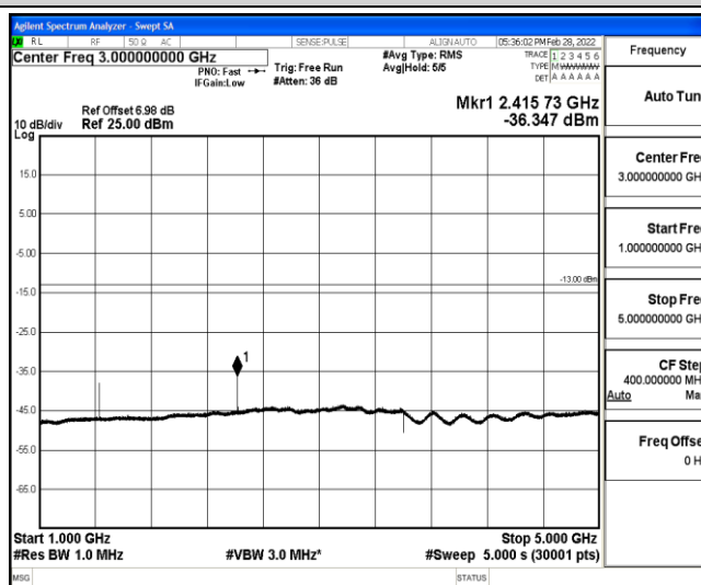
Band12-10MHz-QPSK-23130-1-0-High-1000-5000--36.35-PASS
