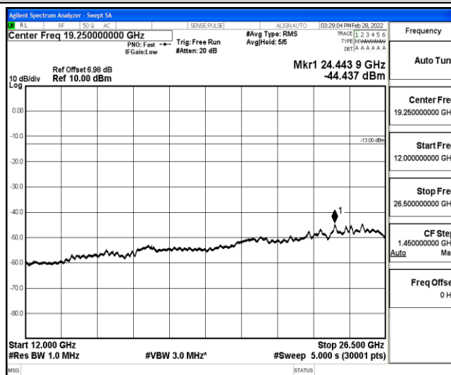
Band12-3MHz-16QAM-23025-1-0-Low-12000-26500--44.44-PASS
