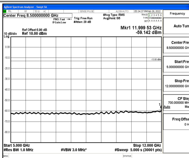
Band12-10MHz-16QAM-23095-1-0-Low-5000-12000--59.14-PASS
