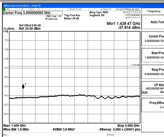
Band12-5MHz-QPSK-23155-1-0-High-1000-5000--37.91-PASS
