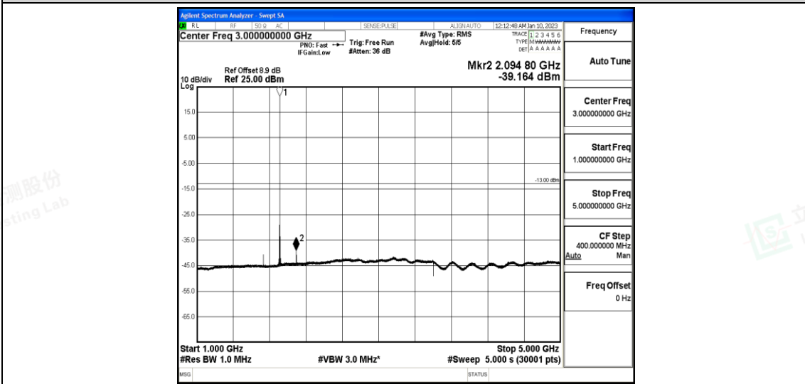
Band25-20MHz-16QAM-26590-1-0-High-1000-5000--39.16-PASS
