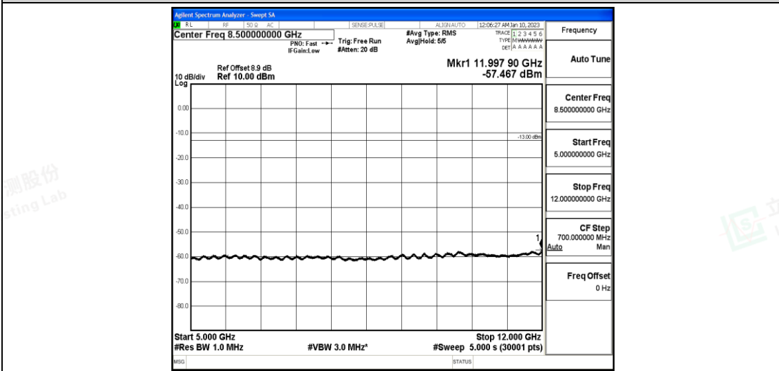
Band25-20MHz-16QAM-26365-1-0-Low-5000-12000--57.47-PASS
