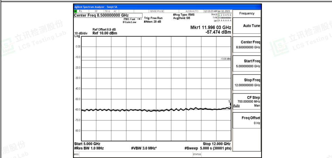
Band25-20MHz-16QAM-26590-1-0-High-5000-12000--57.47-PASS
