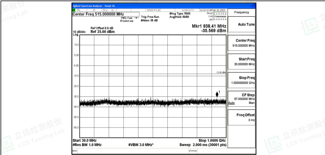
Band25-20MHz-16QAM-26590-1-0-High-30-1000--35.57-PASS
