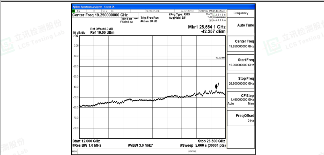
Band25-20MHz-16QAM-26365-1-0-Low-12000-26500--42.26-PASS
