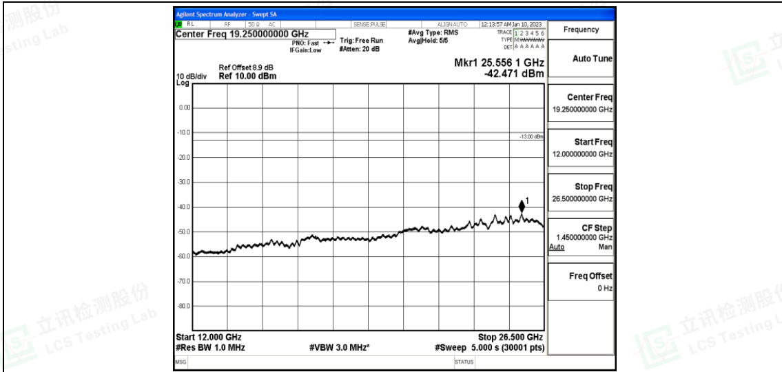
Band25-20MHz-16QAM-26590-1-0-High-12000-26500--42.47-PASS
