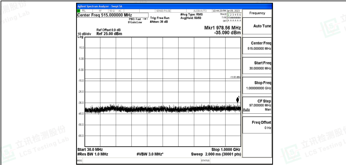
Band25-5MHz-16QAM-26665-1-0-High-30-1000--35.09-PASS
