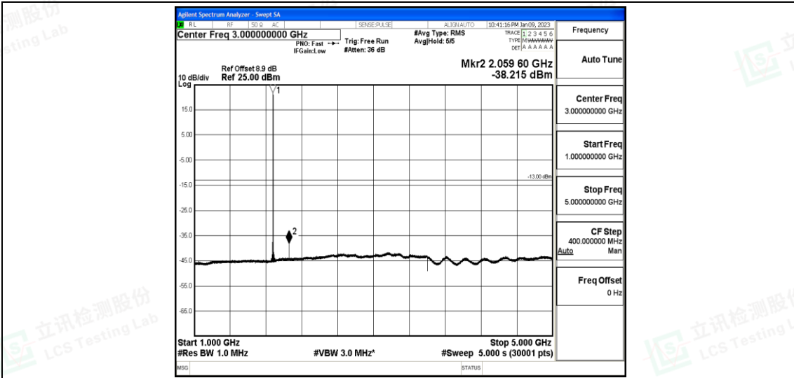
Band25-5MHz-16QAM-26365-1-0-Low-1000-5000--38.22-PASS
