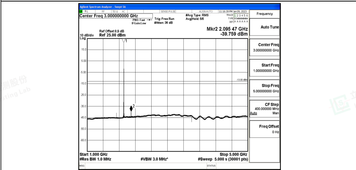
Band25-10MHz-16QAM-26640-1-0-High-1000-5000--39.76-PASS
