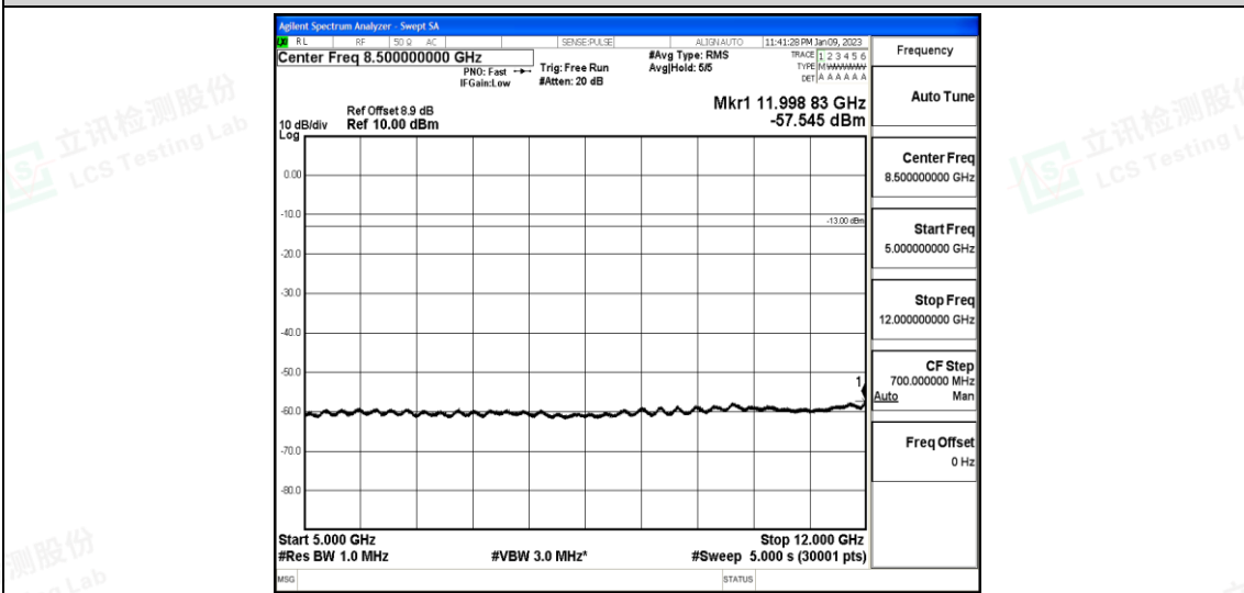
Band25-15MHz-QPSK-26615-1-0-High-5000-12000--57.55-PASS
