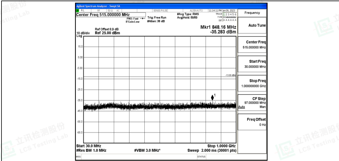
Band25-10MHz-QPSK-26640-1-0-High-30-1000--35.28-PASS
