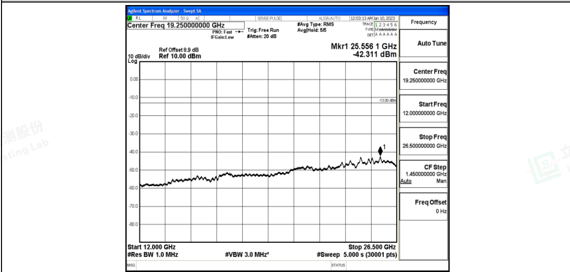
Band25-20MHz-16QAM-26140-1-0-Low-12000-26500--42.31-PASS
