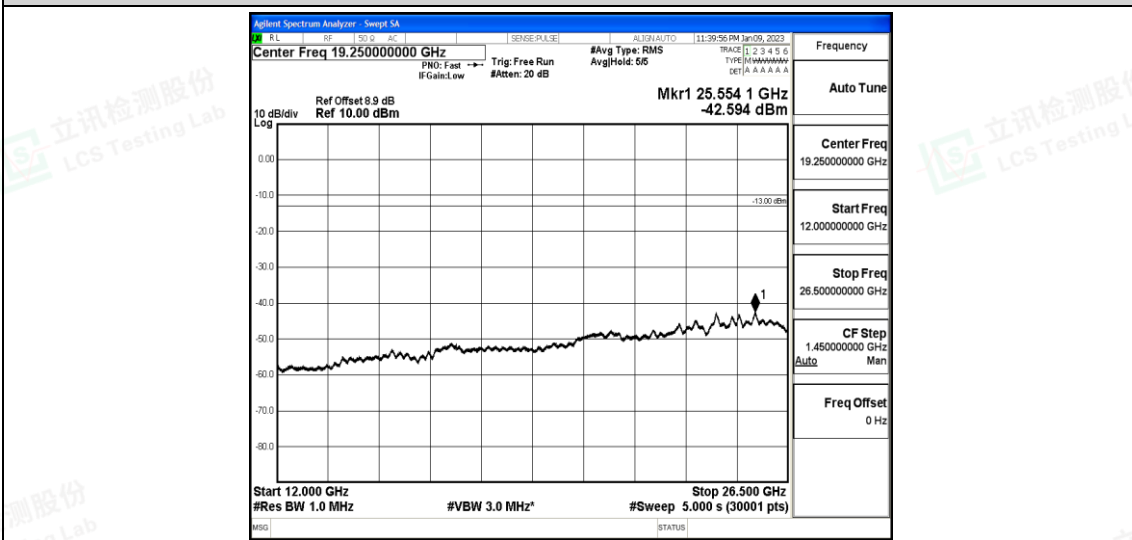
Band25-15MHz-16QAM-26365-1-0-Low-12000-26500--42.59-PASS
