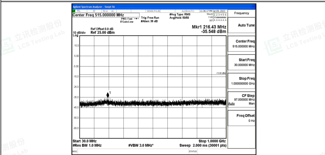
Band25-15MHz-QPSK-26365-1-0-Low-30-1000--35.55-PASS
