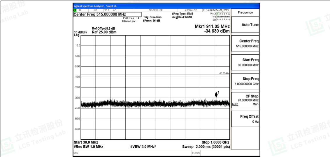
Band25-10MHz-16QAM-26640-1-0-High-30-1000--34.63-PASS
