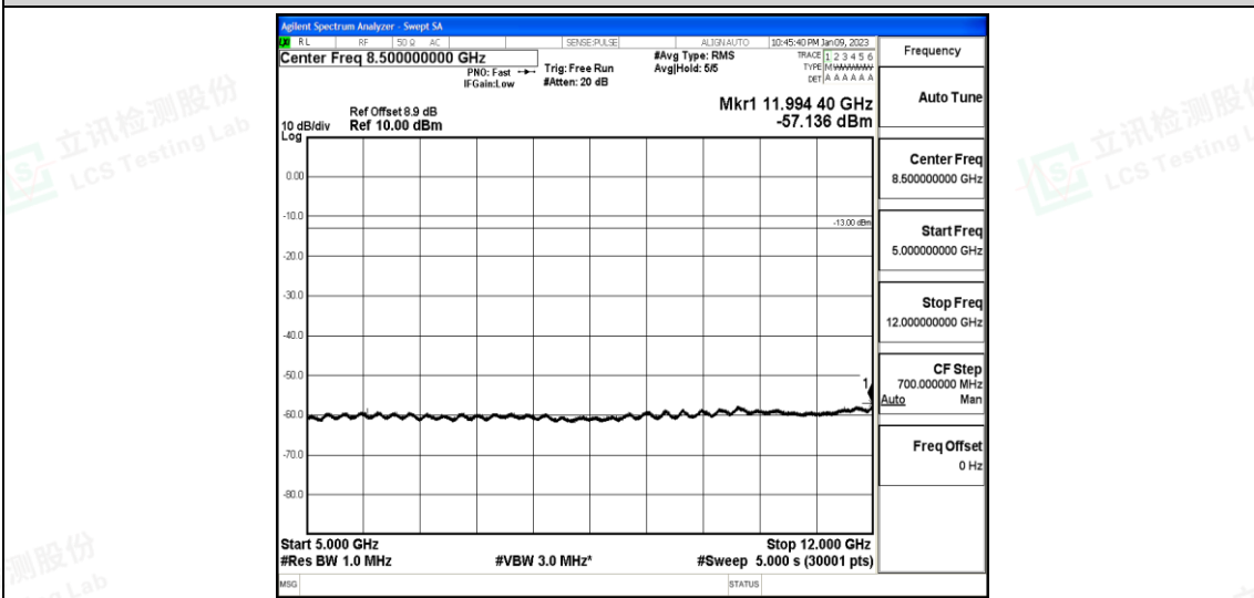
Band25-5MHz-16QAM-26665-1-0-High-5000-12000--57.14-PASS
