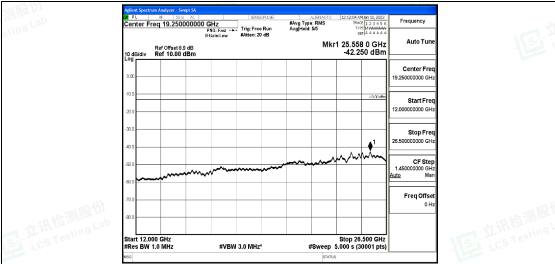
Band25-20MHz-QPSK-26590-1-0-High-12000-26500--42.25-PASS
