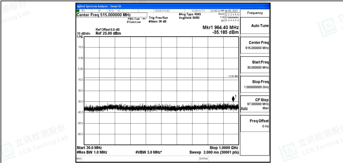
Band25-15MHz-16QAM-26615-1-0-High-30-1000--35.19-PASS
