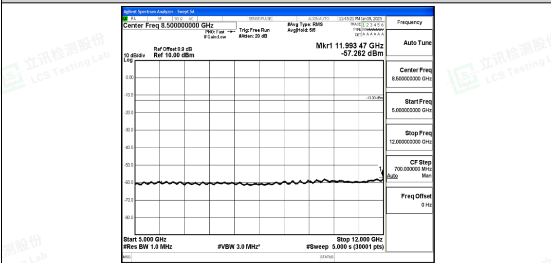
Band25-15MHz-16QAM-26615-1-0-High-5000-12000--57.26-PASS
