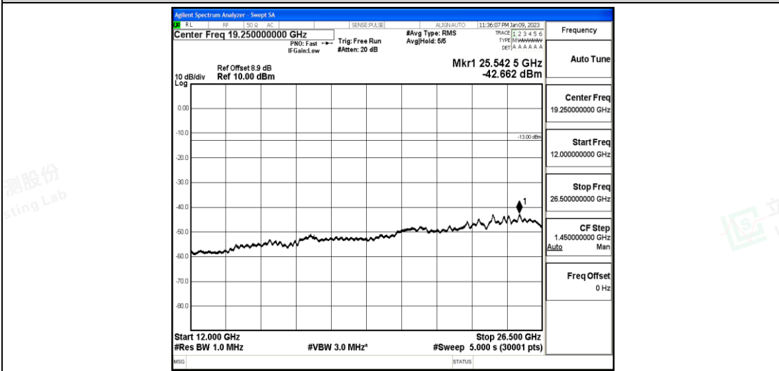
Band25-15MHz-16QAM-26115-1-0-Low-12000-26500--42.66-PASS
