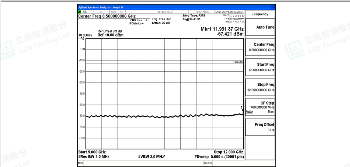
Band25-20MHz-QPSK-26590-1-0-High-5000-12000--57.42-PASS
