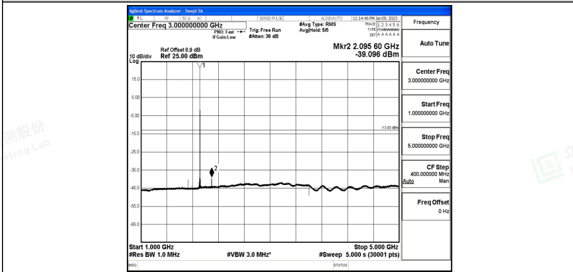
Band25-10MHz-QPSK-26640-1-0-High-1000-5000--39.1-PASS
