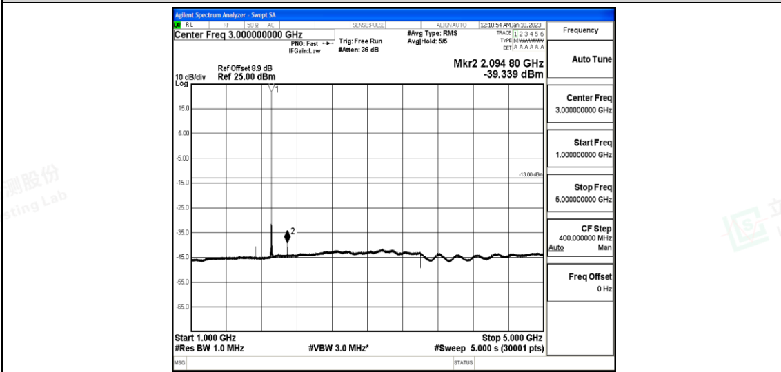
Band25-20MHz-QPSK-26590-1-0-High-1000-5000--39.34-PASS
