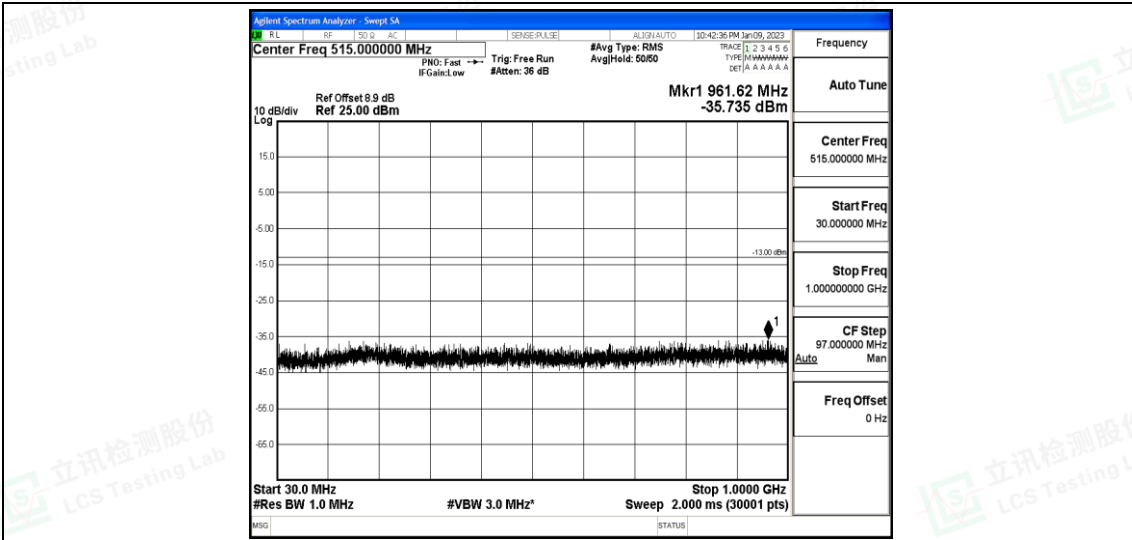
Band25-5MHz-QPSK-26665-1-0-High-30-1000--35.74-PASS
