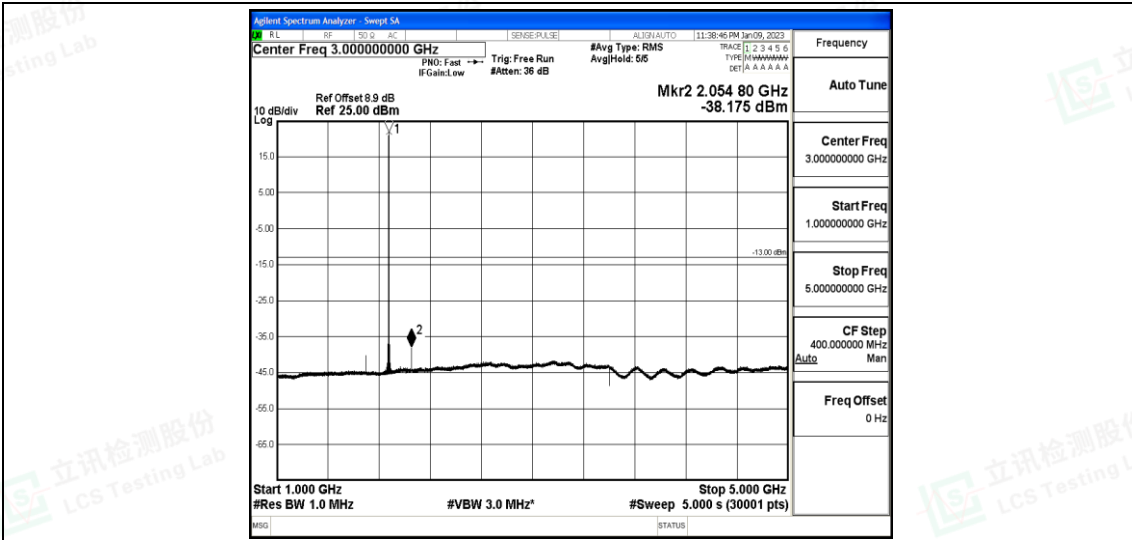
Band25-15MHz-16QAM-26365-1-0-Low-1000-5000--38.18-PASS
