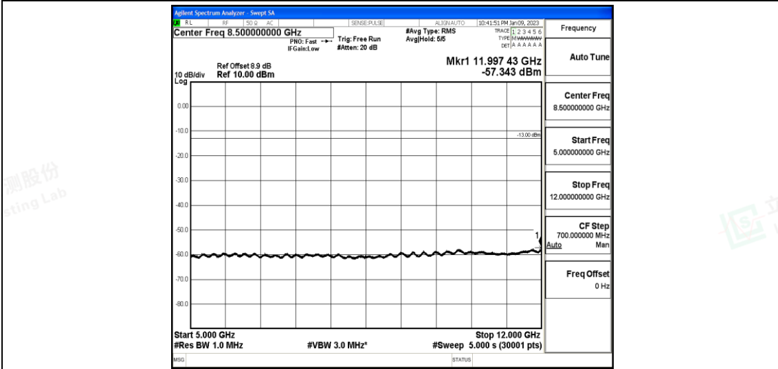
Band25-5MHz-16QAM-26365-1-0-Low-5000-12000--57.34-PASS
