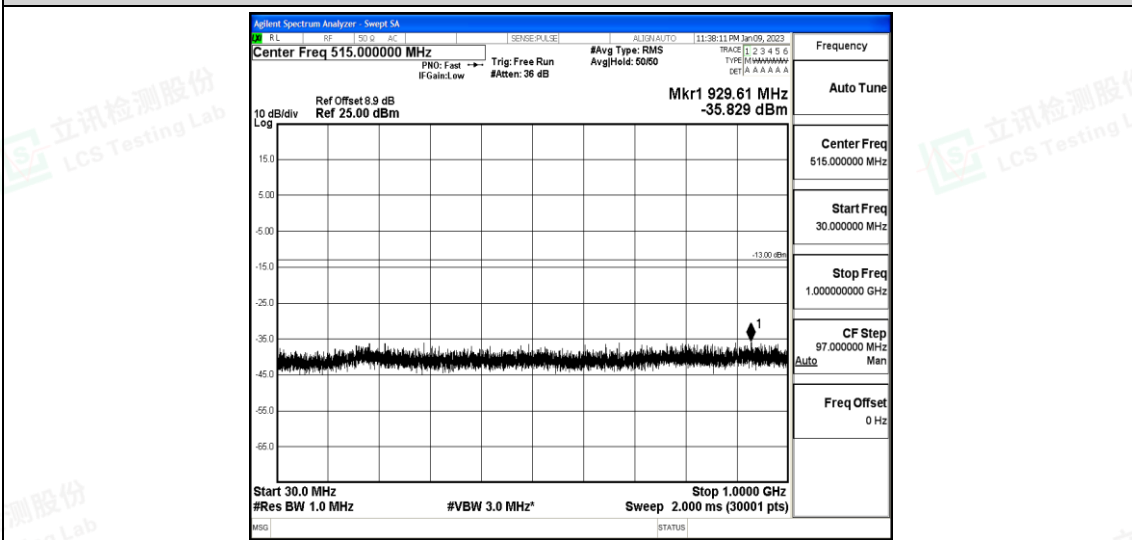
Band25-15MHz-16QAM-26365-1-0-Low-30-1000--35.83-PASS
