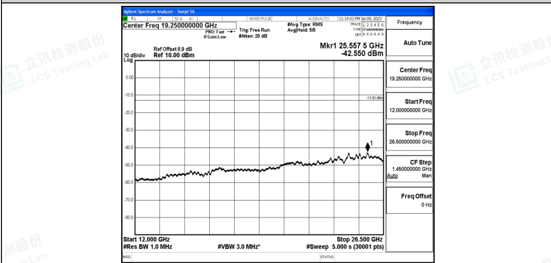
Band25-10MHz-16QAM-26365-1-0-Low-12000-26500--42.55-PASS
