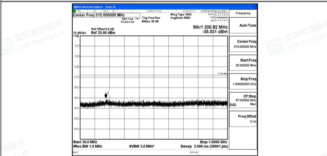
Band25-20MHz-16QAM-26365-1-0-Low-30-1000--35.53-PASS
