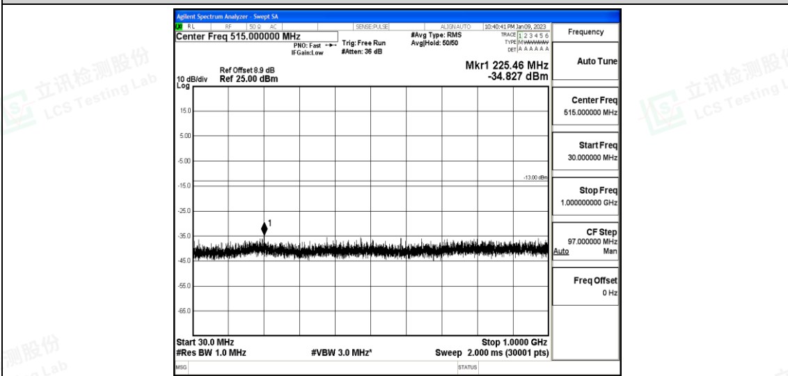
Band25-5MHz-16QAM-26365-1-0-Low-30-1000--34.83-PASS
