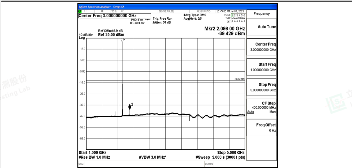
Band25-5MHz-16QAM-26665-1-0-High-1000-5000--39.43-PASS
