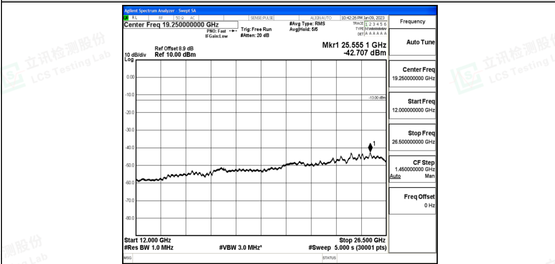
Band25-5MHz-16QAM-26365-1-0-Low-12000-26500--42.71-PASS
