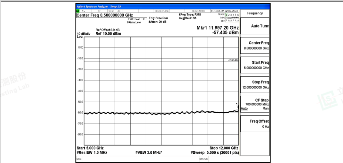
Band25-10MHz-16QAM-26365-1-0-Low-5000-12000--57.44-PASS
