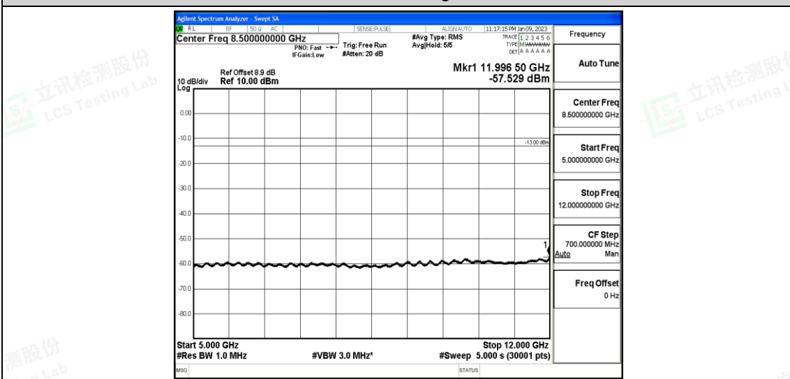
Band25-10MHz-16QAM-26640-1-0-High-5000-12000--57.53-PASS
