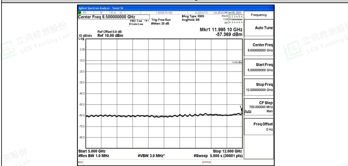
Band25-10MHz-QPSK-26640-1-0-High-5000-12000--57.37-PASS
