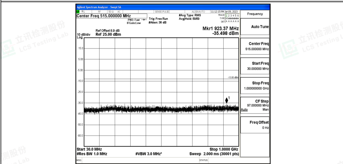
Band25-10MHz-16QAM-26365-1-0-Low-30-1000--35.5-PASS
