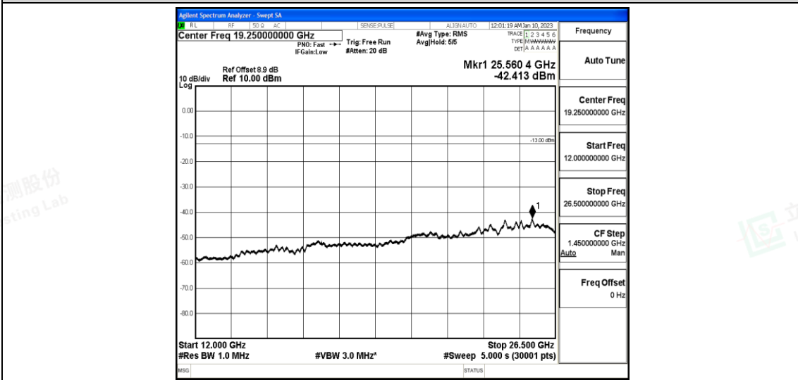
Band25-20MHz-QPSK-26140-1-0-Low-12000-26500--42.41-PASS
