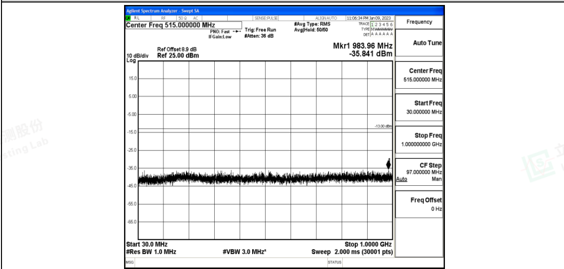
Band25-10MHz-QPSK-26090-1-0-Low-30-1000--35.84-PASS
