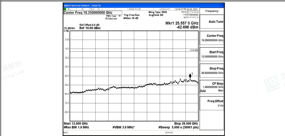
Band25-5MHz-16QAM-26065-1-0-Low-12000-26500--42.7-PASS
