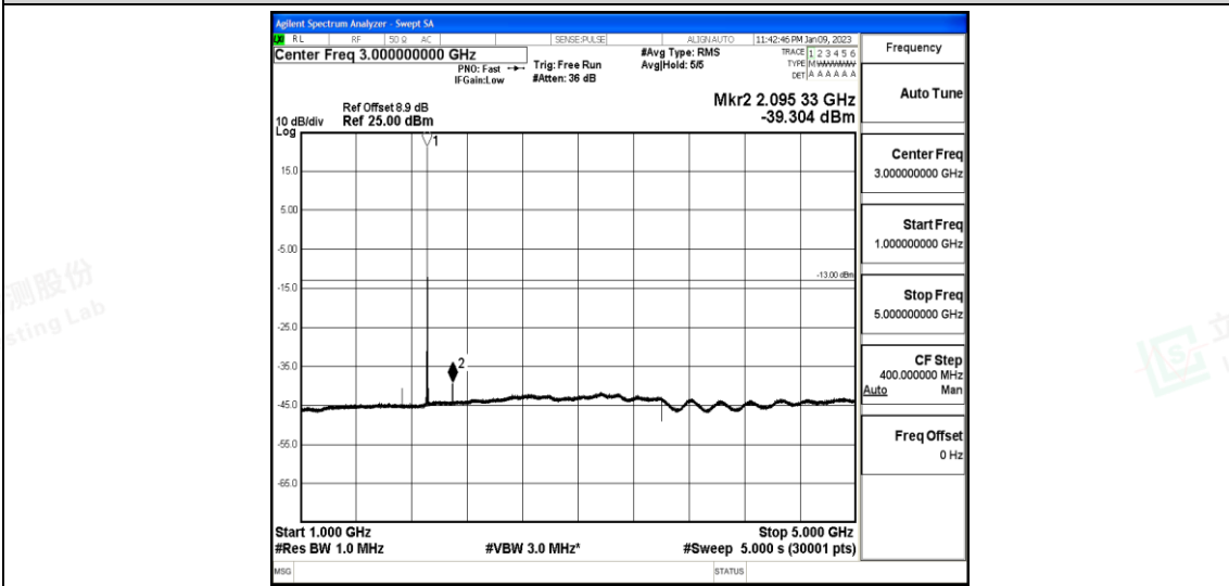
Band25-15MHz-16QAM-26615-1-0-High-1000-5000--39.3-PASS
