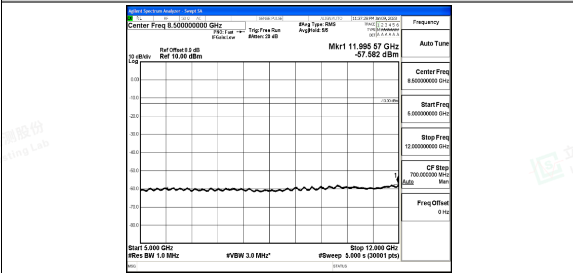
Band25-15MHz-QPSK-26365-1-0-Low-5000-12000--57.58-PASS
