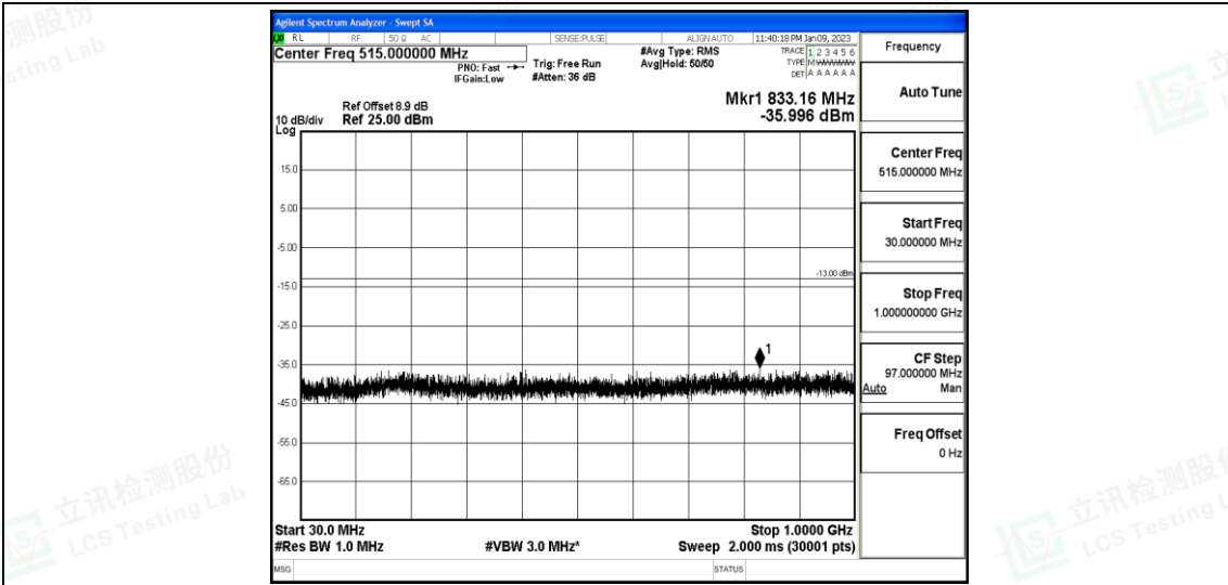
Band25-15MHz-QPSK-26615-1-0-High-30-1000--36-PASS
