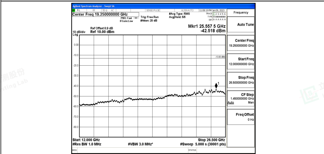
Band25-10MHz-QPSK-26090-1-0-Low-12000-26500--42.52-PASS
