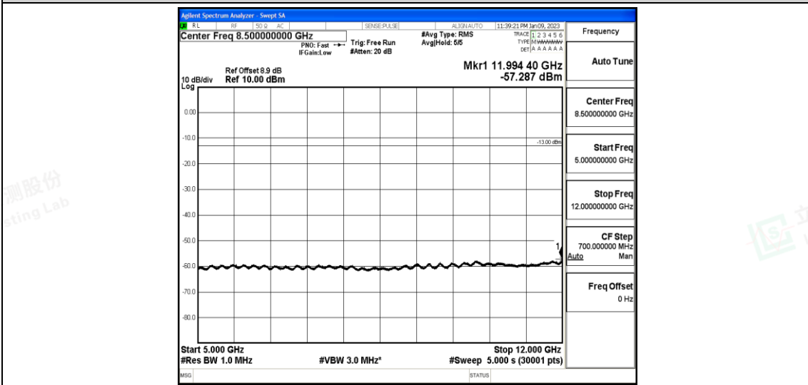
Band25-15MHz-16QAM-26365-1-0-Low-5000-12000--57.29-PASS
