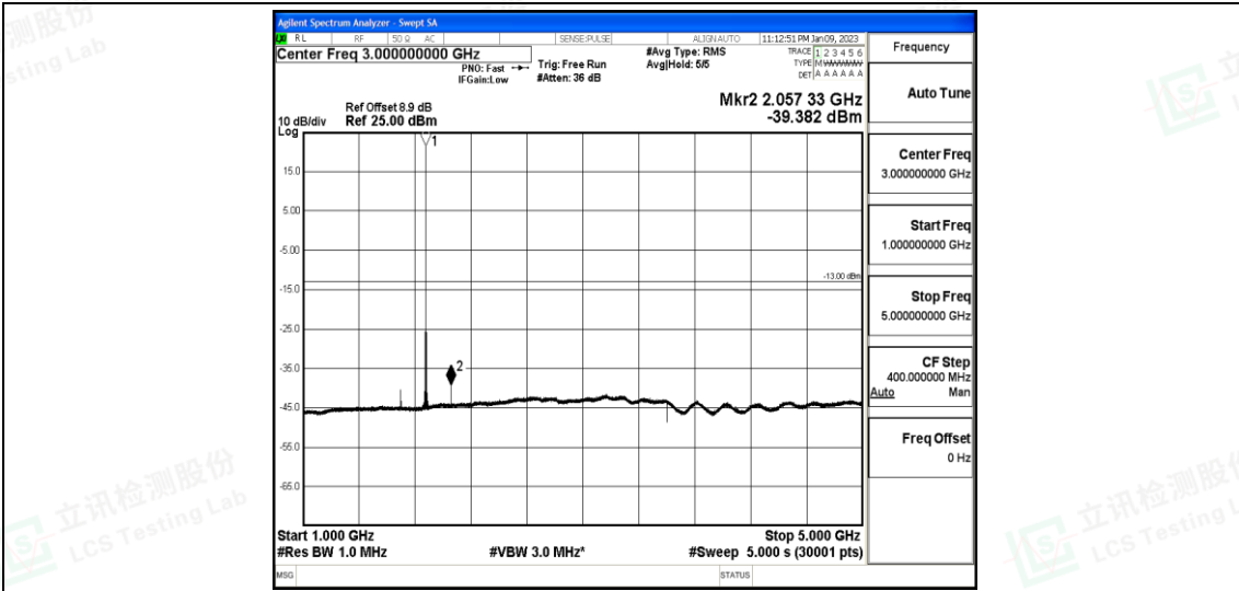
Band25-10MHz-16QAM-26365-1-0-Low-1000-5000--39.38-PASS
