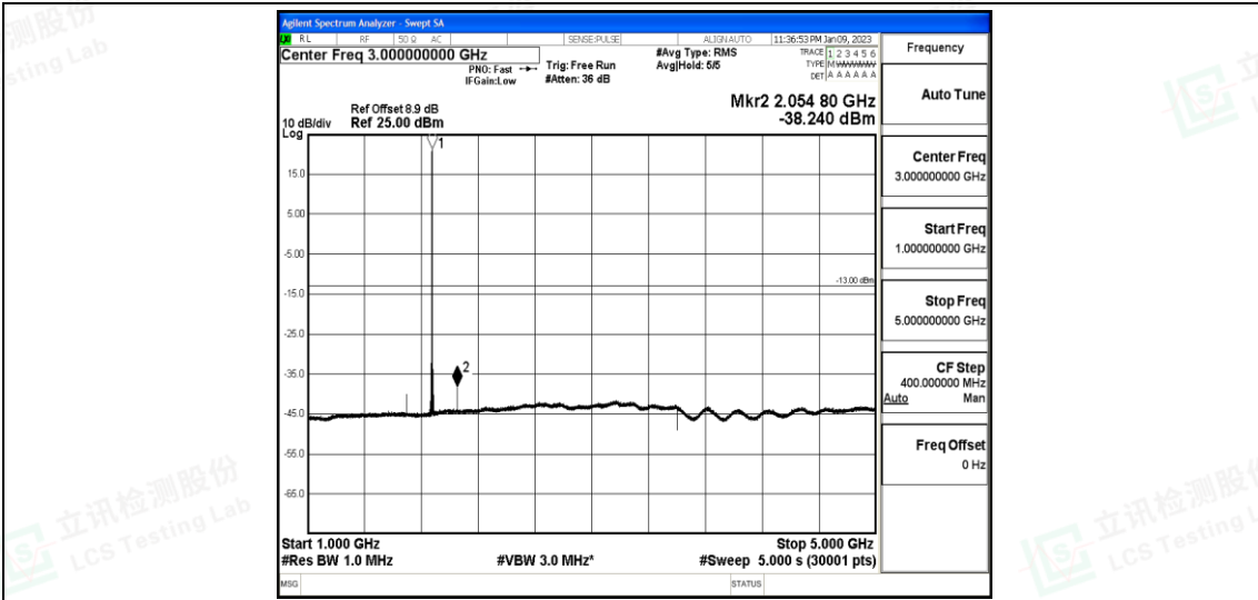
Band25-15MHz-QPSK-26365-1-0-Low-1000-5000--38.24-PASS
