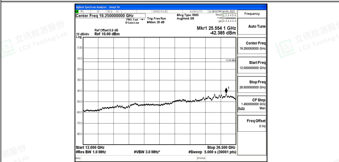
Band25-15MHz-QPSK-26365-1-0-Low-12000-26500--42.39-PASS
