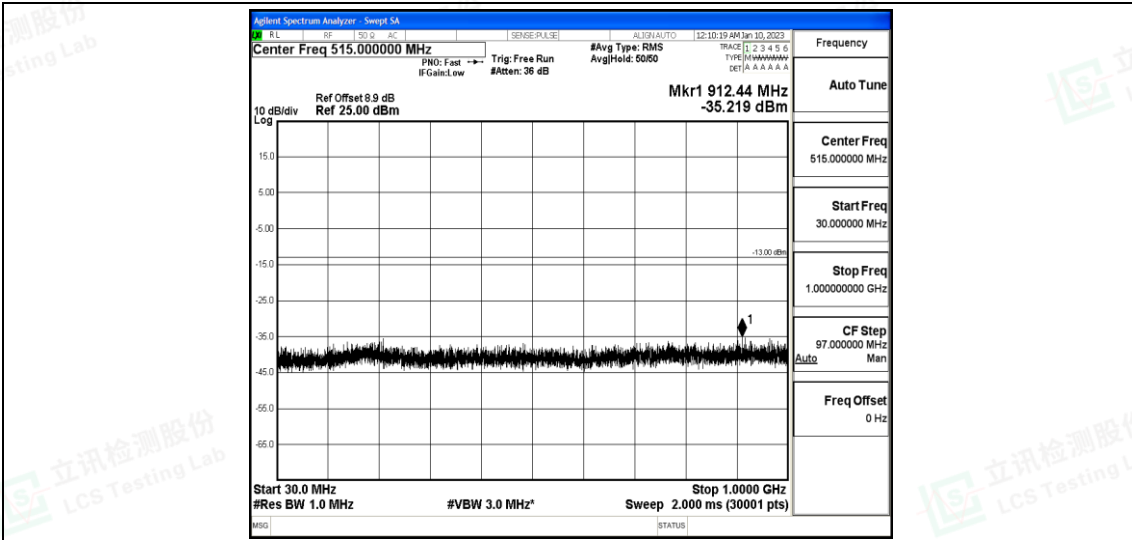
Band25-20MHz-QPSK-26590-1-0-High-30-1000--35.22-PASS
