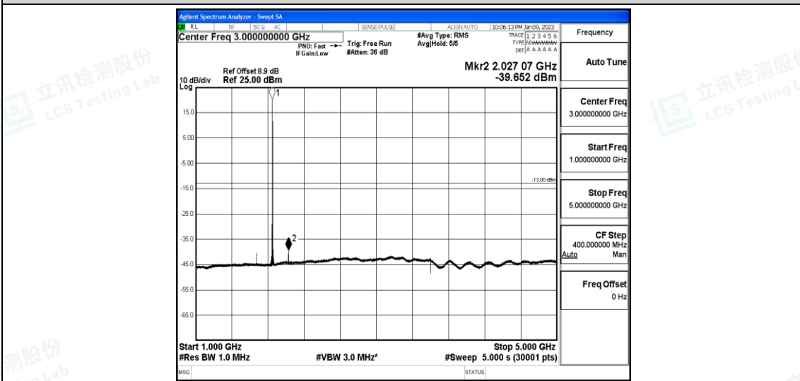
Band25-3MHz-QPSK-26055-1-0-Low-1000-5000--39.65-PASS
