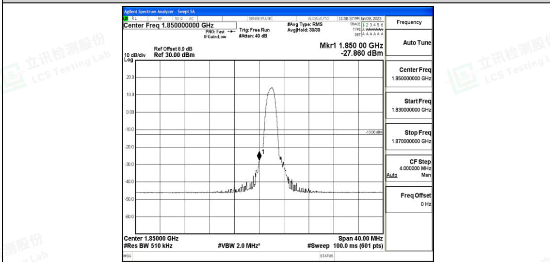
Band25-20MHz-16QAM-26140-6-0-Low--27.86-PASS
