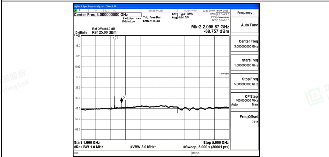
Band25-3MHz-QPSK-26675-1-0-High-1000-5000--39.76-PASS
