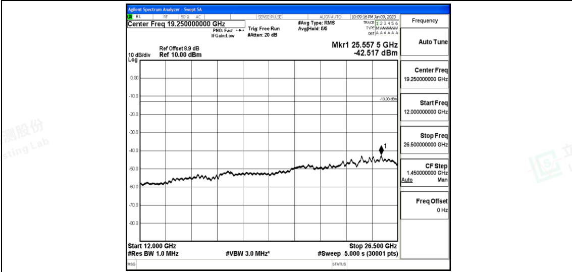
Band25-3MHz-16QAM-26055-1-0-Low-12000-26500--42.52-PASS
