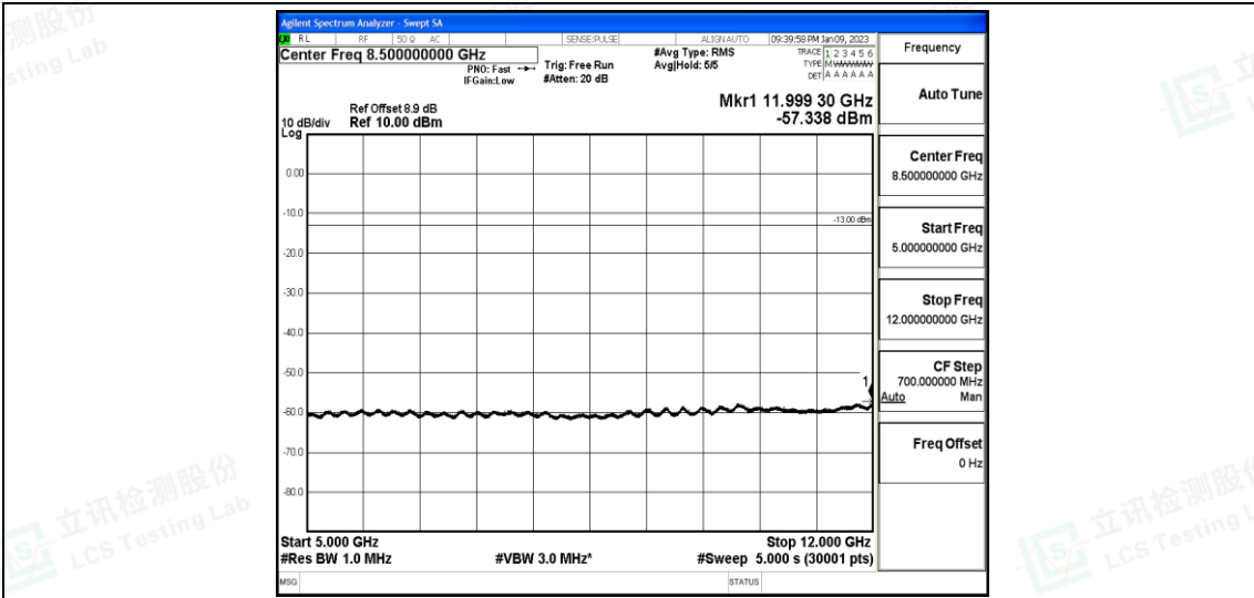
Band25-1.4MHz-16QAM-26047-1-0-Low-5000-12000--57.34-PASS
