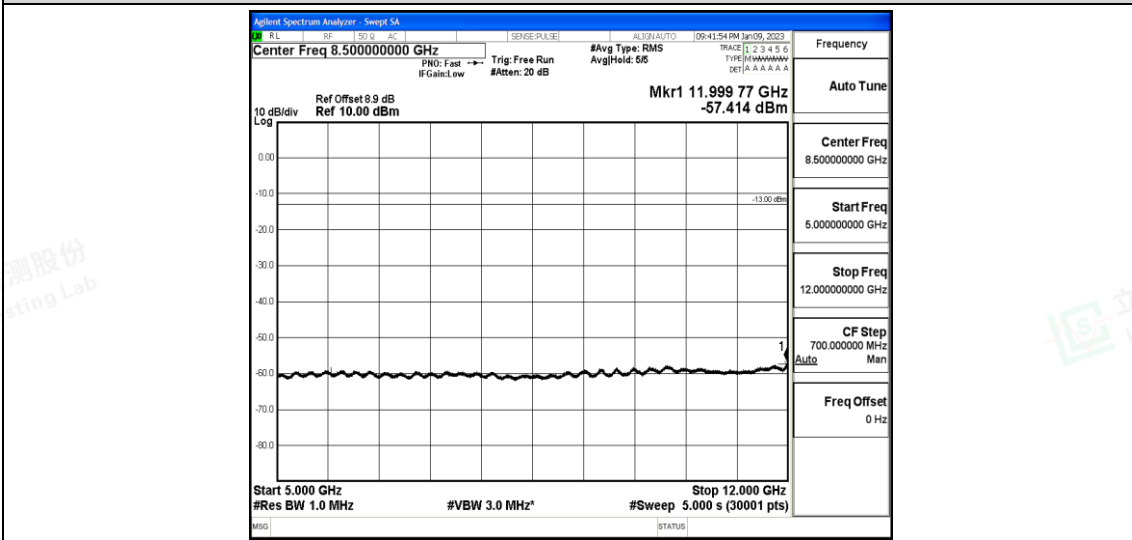
Band25-1.4MHz-QPSK-26365-1-0-Low-5000-12000--57.41-PASS
