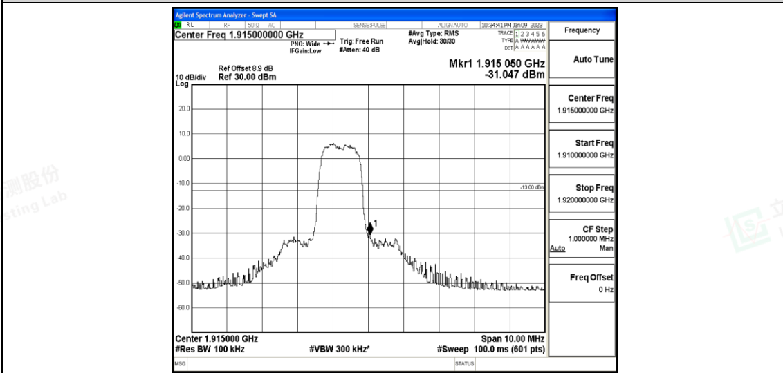
Band25-5MHz-QPSK-26665-6-0-High--31.05-PASS
