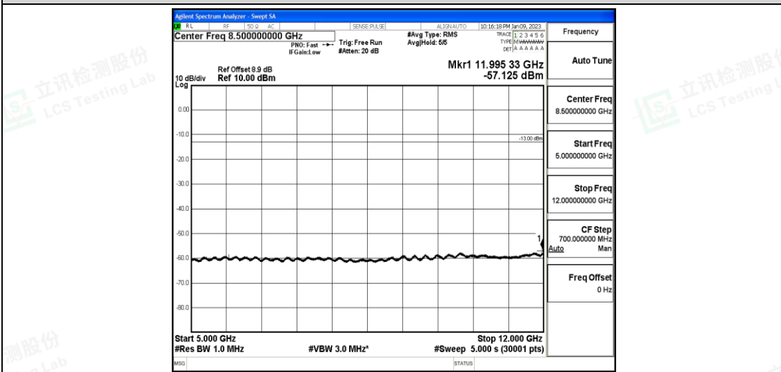
Band25-3MHz-16QAM-26675-1-0-High-5000-12000--57.13-PASS
