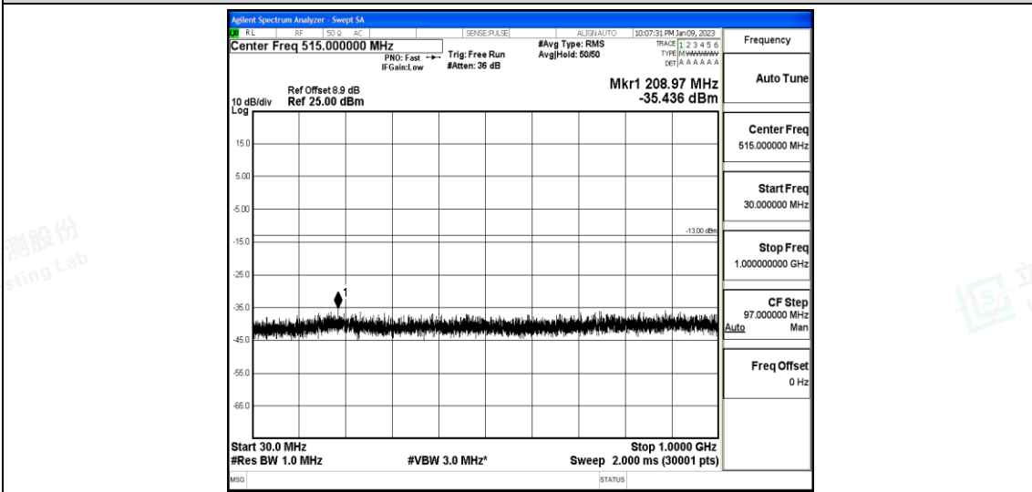
Band25-3MHz-16QAM-26055-1-0-Low-30-1000--35.44-PASS
