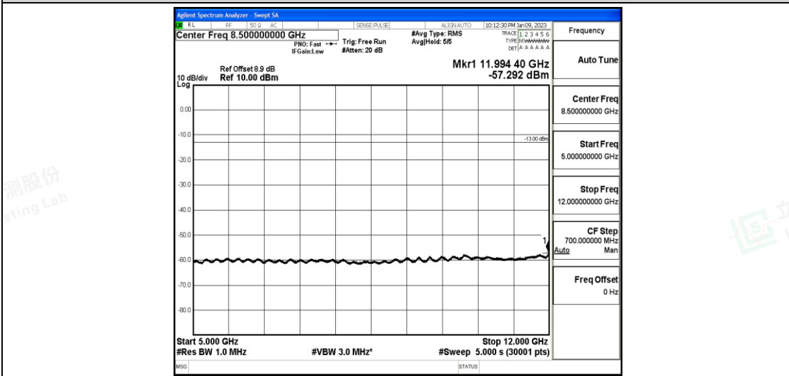
Band25-3MHz-16QAM-26365-1-0-Low-5000-12000--57.29-PASS
