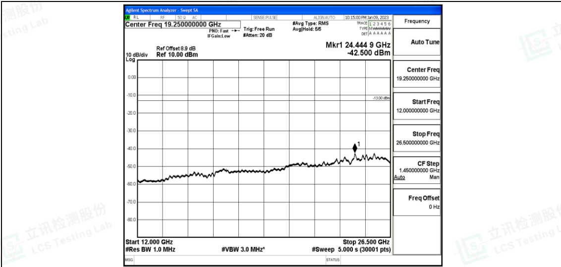
Band25-3MHz-QPSK-26675-1-0-High-12000-26500--42.5-PASS
