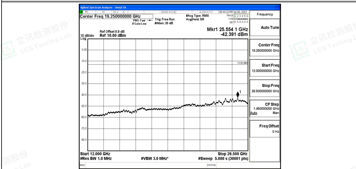
Band25-1.4MHz-16QAM-26365-1-0-Low-12000-26500--42.39-PASS
