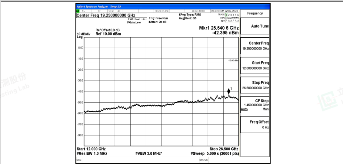
Band25-1.4MHz-16QAM-26047-1-0-Low-12000-26500--42.4-PASS
