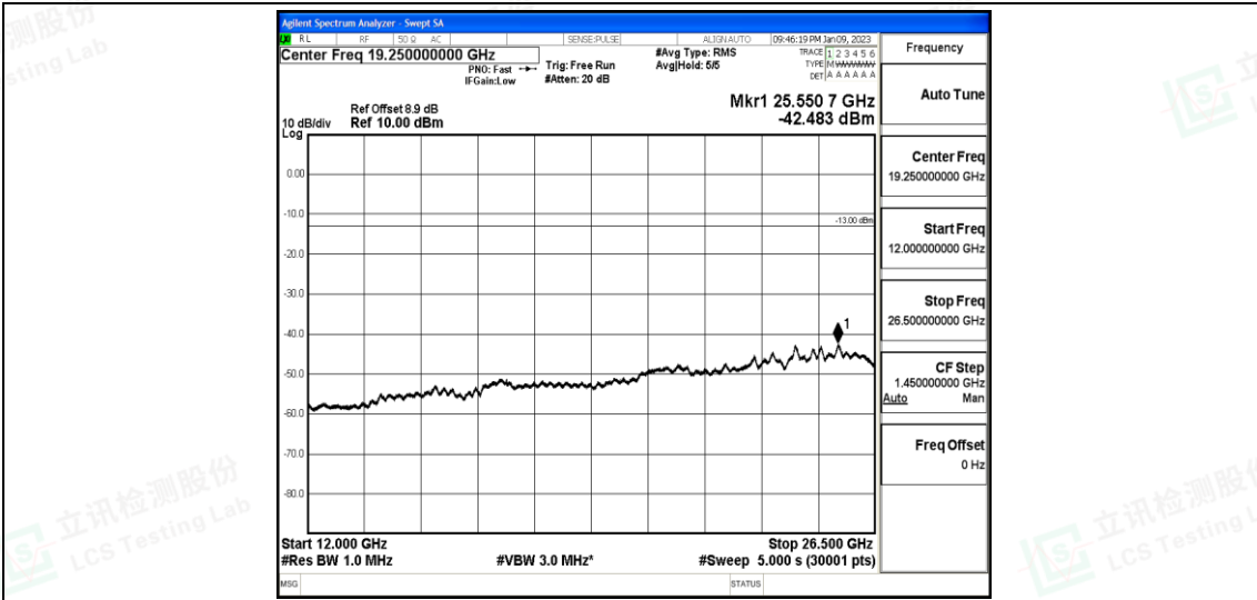
Band25-1.4MHz-QPSK-26683-1-0-High-12000-26500--42.48-PASS
