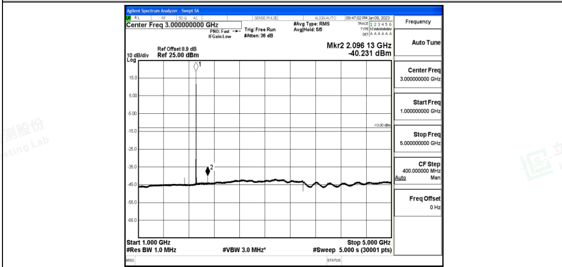
Band25-1.4MHz-16QAM-26683-1-0-High-1000-5000--40.23-PASS
