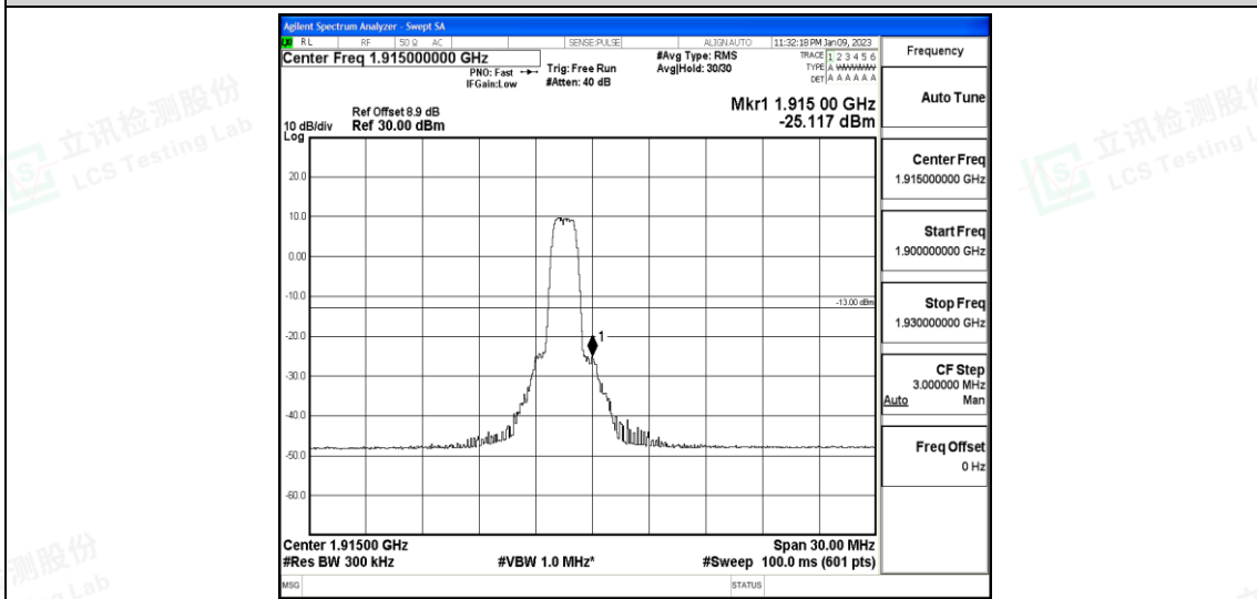
Band25-15MHz-16QAM-26615-6-0-High--25.12-PASS
