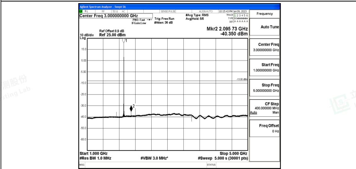
Band25-3MHz-16QAM-26675-1-0-High-1000-5000--40.35-PASS
