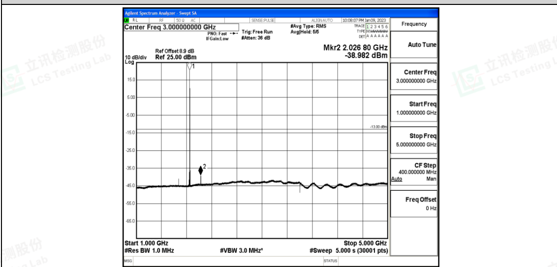
Band25-3MHz-16QAM-26055-1-0-Low-1000-5000--38.98-PASS
