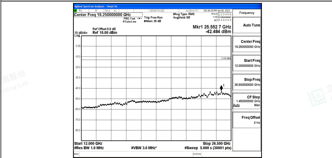
Band25-1.4MHz-QPSK-26047-1-0-Low-12000-26500--42.48-PASS
