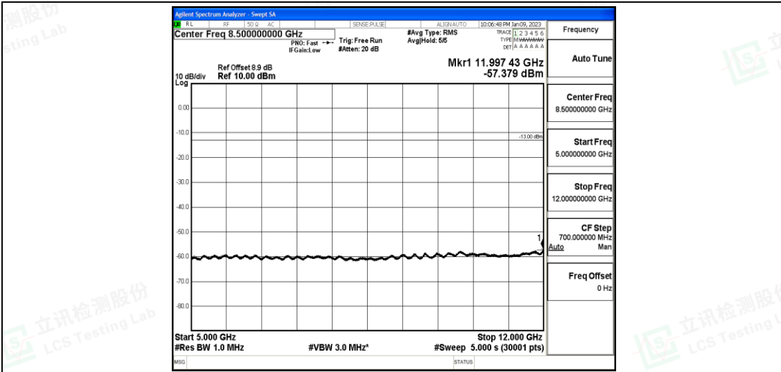
Band25-3MHz-QPSK-26055-1-0-Low-5000-12000--57.38-PASS
