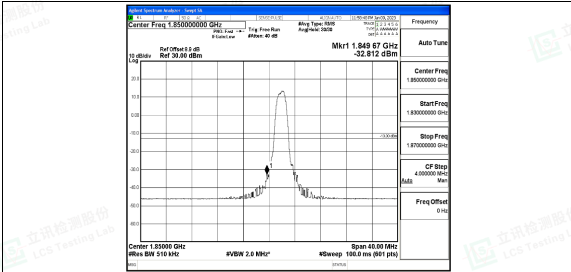
Band25-20MHz-QPSK-26140-6-0-Low--32.81-PASS
