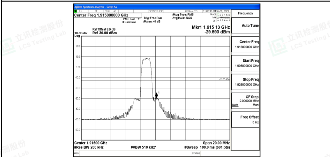
Band25-10MHz-QPSK-26640-6-0-High--29.59-PASS
