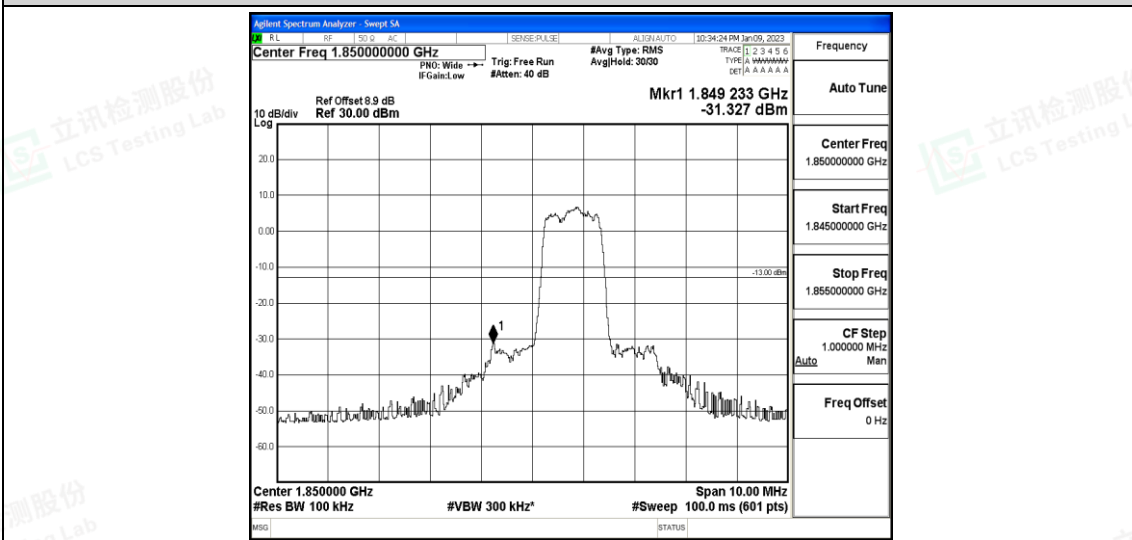
Band25-5MHz-16QAM-26065-6-0-Low--31.33-PASS
