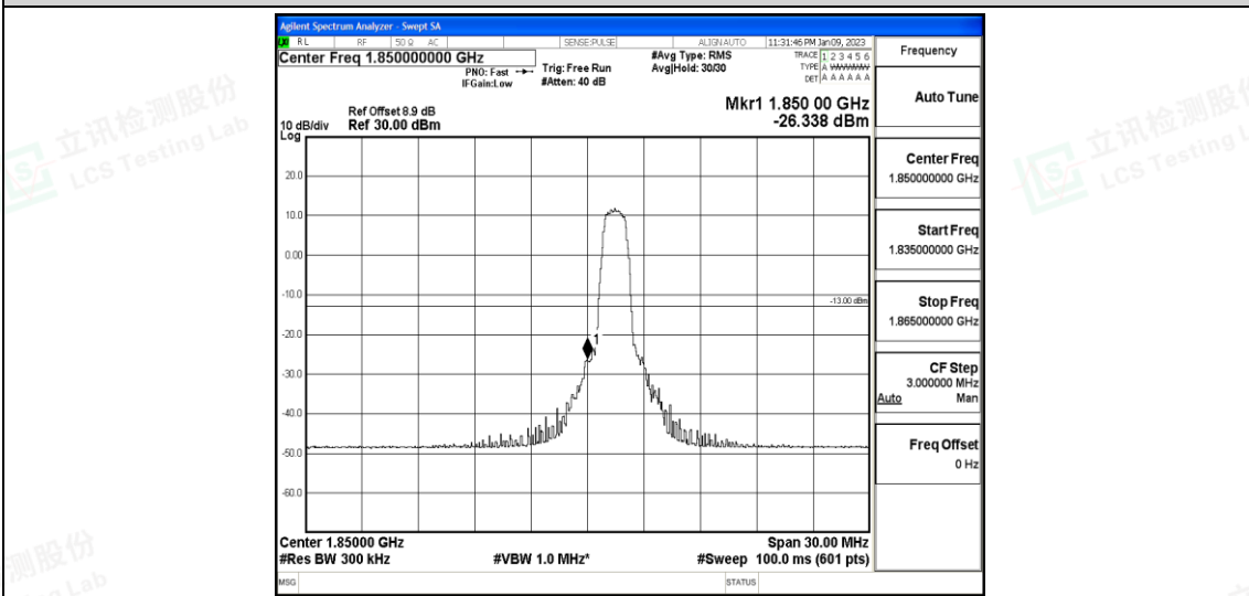
Band25-15MHz-QPSK-26115-6-0-Low--26.34-PASS
