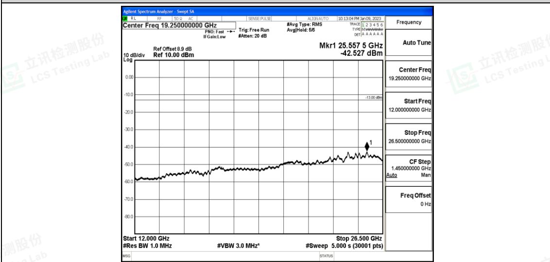
Band25-3MHz-16QAM-26365-1-0-Low-12000-26500--42.53-PASS
