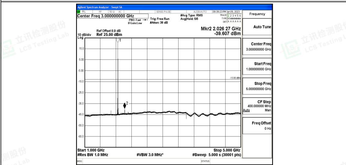
Band25-1.4MHz-16QAM-26047-1-0-Low-1000-5000--39.61-PASS
