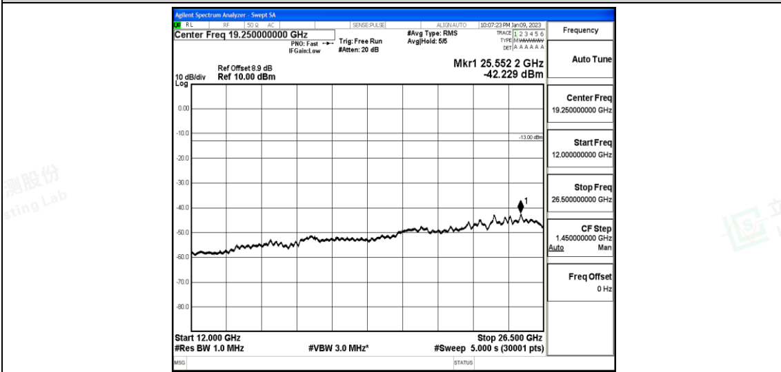
Band25-3MHz-QPSK-26055-1-0-Low-12000-26500--42.23-PASS
