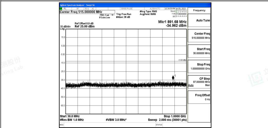
Band25-5MHz-QPSK-26065-1-0-Low-30-1000--34.96-PASS
