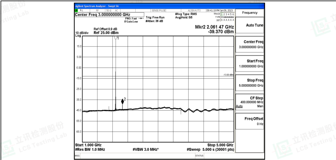
Band25-1.4MHz-QPSK-26365-1-0-Low-1000-5000--39.37-PASS
