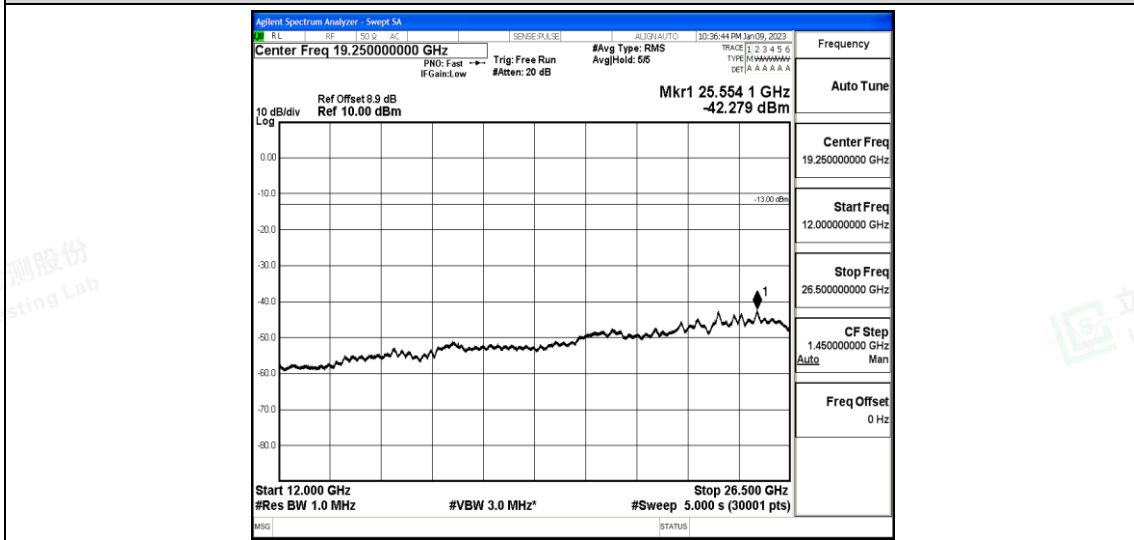
Band25-5MHz-QPSK-26065-1-0-Low-12000-26500--42.28-PASS
