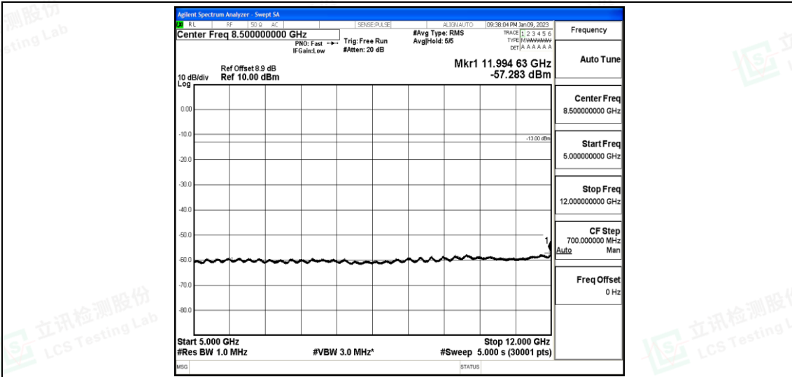
Band25-1.4MHz-QPSK-26047-1-0-Low-5000-12000--57.28-PASS
