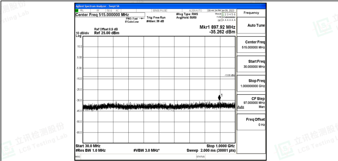
Band25-1.4MHz-QPSK-26683-1-0-High-30-1000--35.26-PASS
