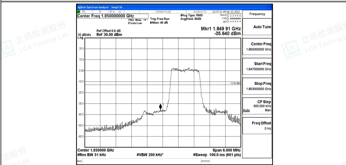
Band25-3MHz-QPSK-26055-6-0-Low--35.64-PASS
