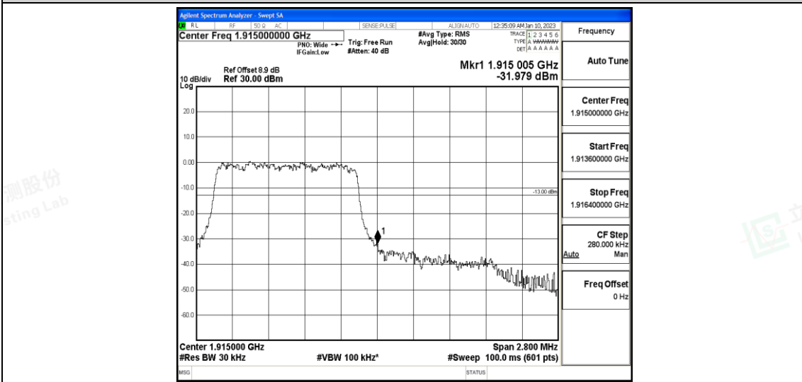
Band25-1.4MHz-16QAM-26683-6-0-High--31.98-PASS
