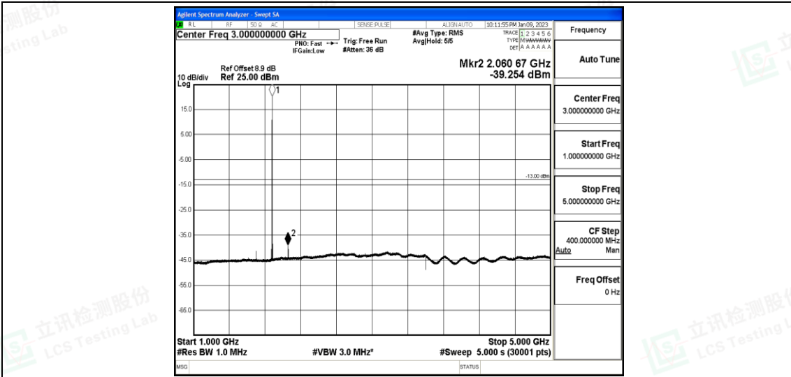
Band25-3MHz-16QAM-26365-1-0-Low-1000-5000--39.25-PASS
