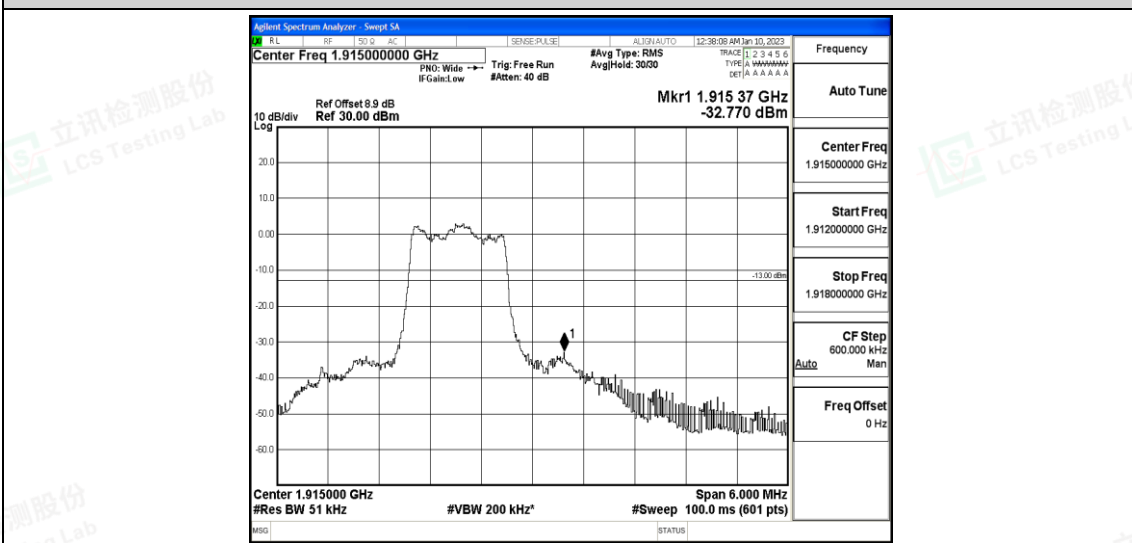
Band25-3MHz-16QAM-26675-6-0-High--32.77-PASS
