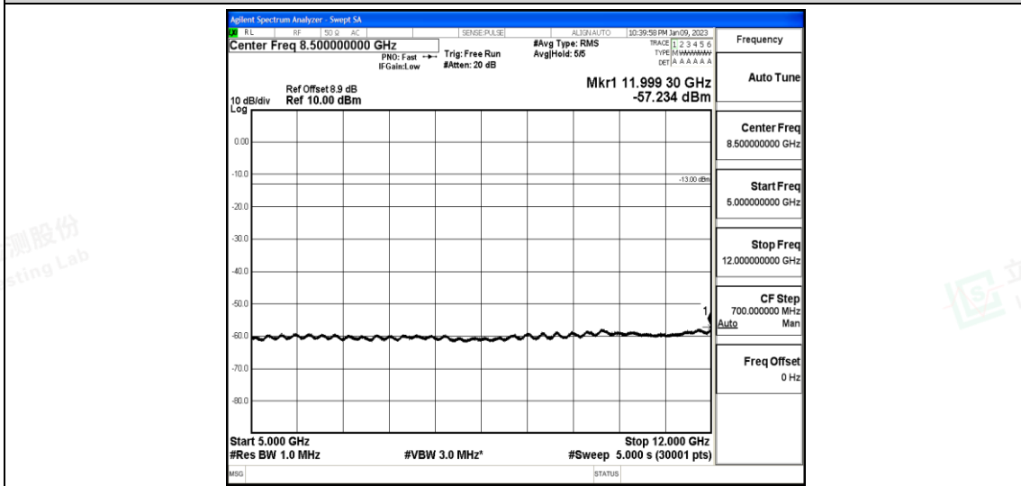
Band25-5MHz-QPSK-26365-1-0-Low-5000-12000--57.23-PASS
