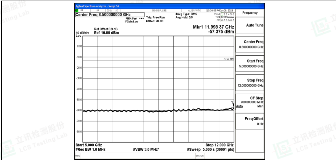
Band25-5MHz-QPSK-26065-1-0-Low-5000-12000--57.38-PASS
