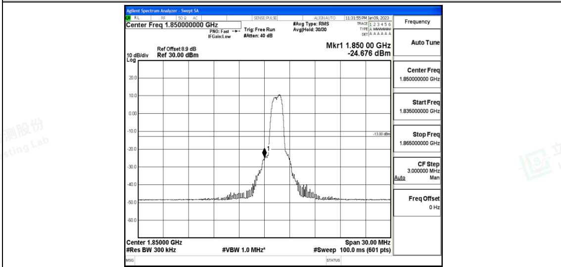
Band25-15MHz-16QAM-26115-6-0-Low--24.68-PASS
