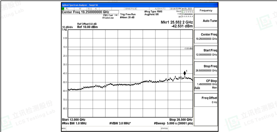
Band25-3MHz-16QAM-26675-1-0-High-12000-26500--42.53-PASS
