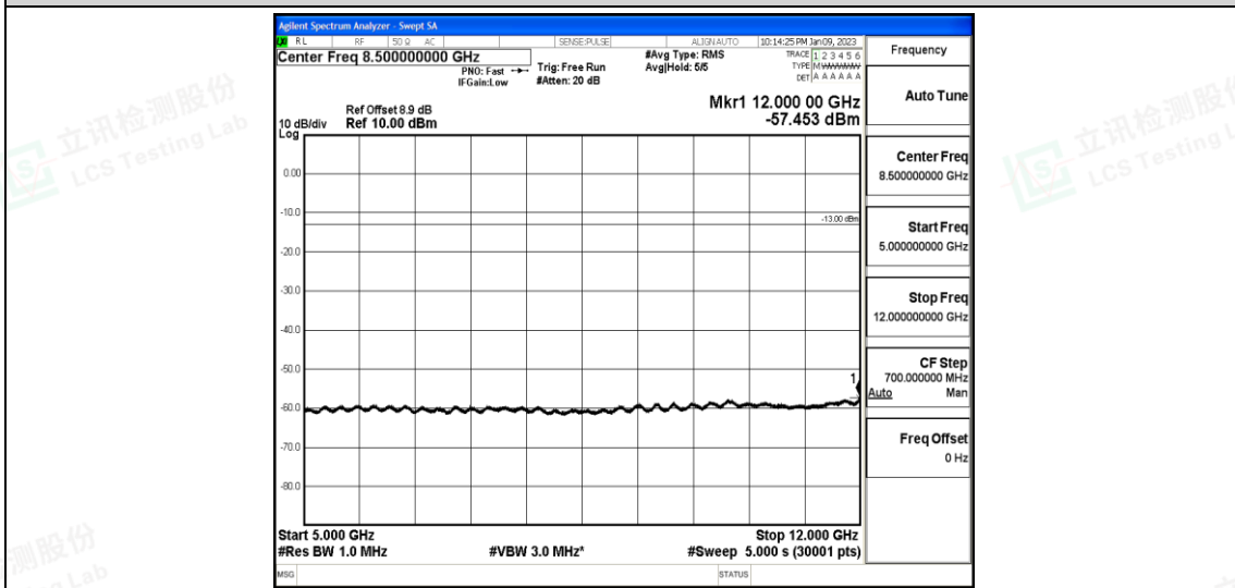
Band25-3MHz-QPSK-26675-1-0-High-5000-12000--57.45-PASS
