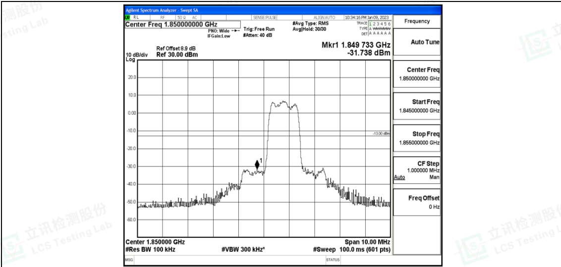
Band25-5MHz-QPSK-26065-6-0-Low--31.74-PASS
