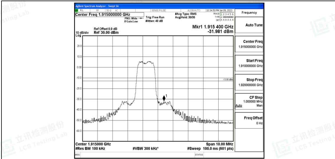
Band25-5MHz-16QAM-26665-6-0-High--31.98-PASS
