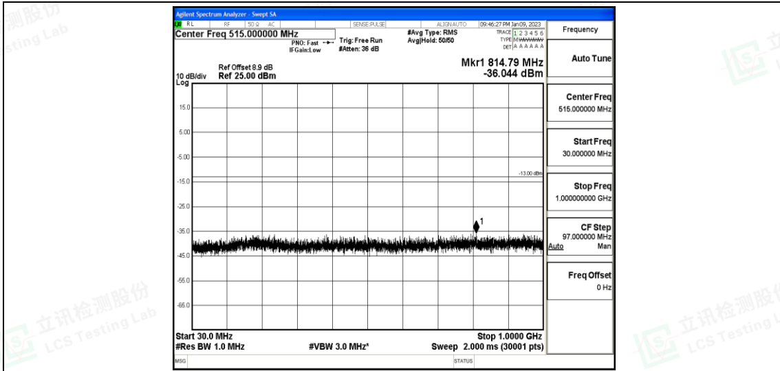
Band25-1.4MHz-16QAM-26683-1-0-High-30-1000--36.04-PASS
