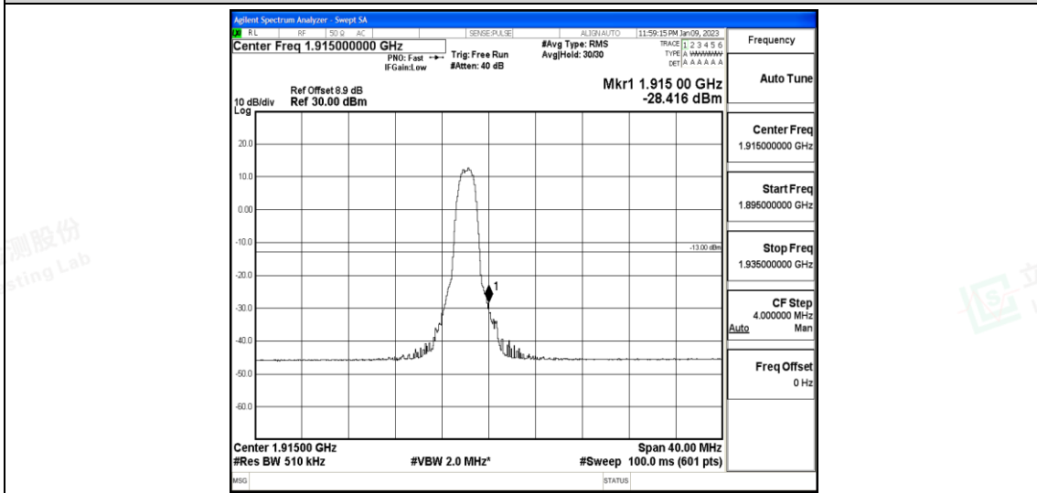
Band25-20MHz-QPSK-26590-6-0-High--28.42-PASS
