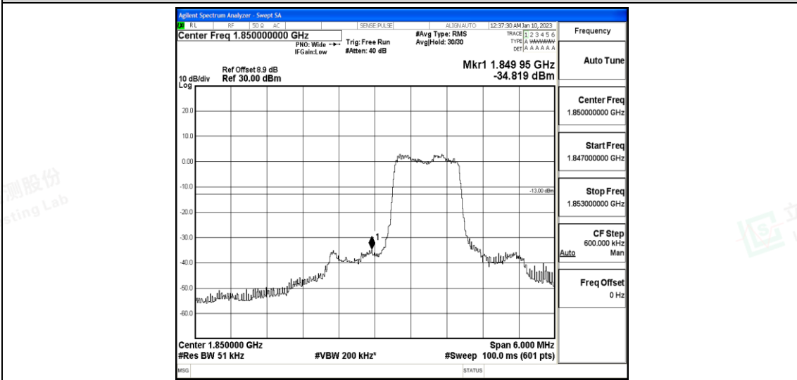
Band25-3MHz-16QAM-26055-6-0-Low--34.82-PASS
