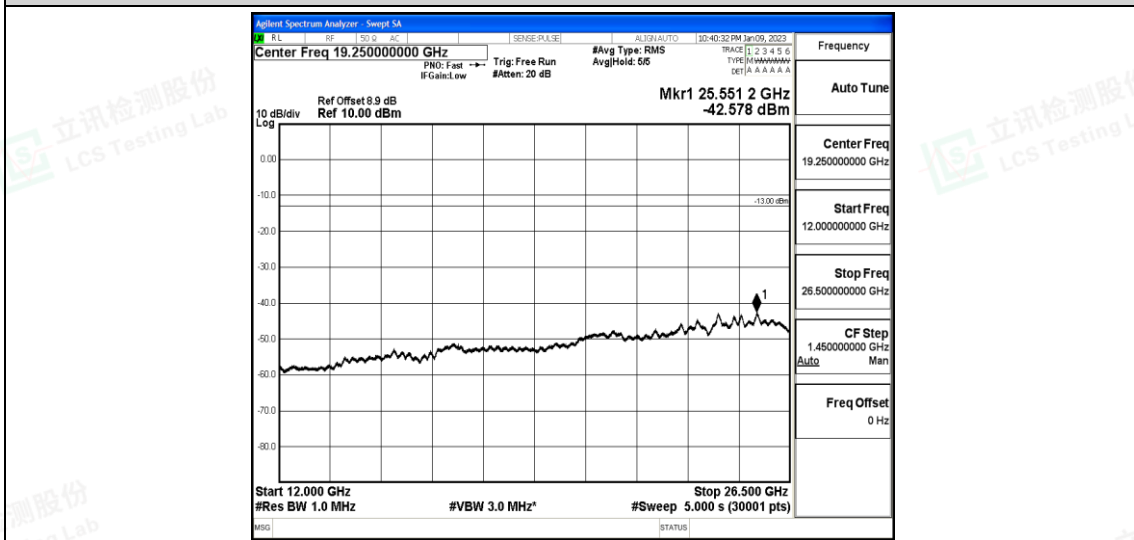
Band25-5MHz-QPSK-26365-1-0-Low-12000-26500--42.58-PASS
