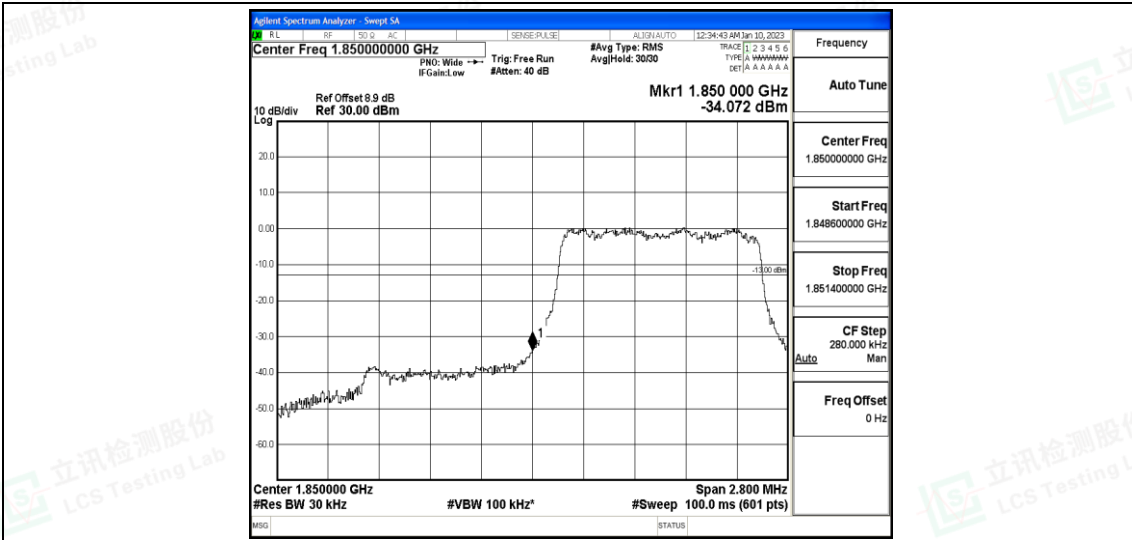
Band25-1.4MHz-16QAM-26047-6-0-Low--34.07-PASS
