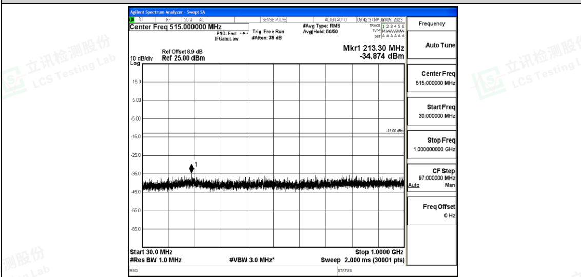
Band25-1.4MHz-16QAM-26365-1-0-Low-30-1000--34.87-PASS
