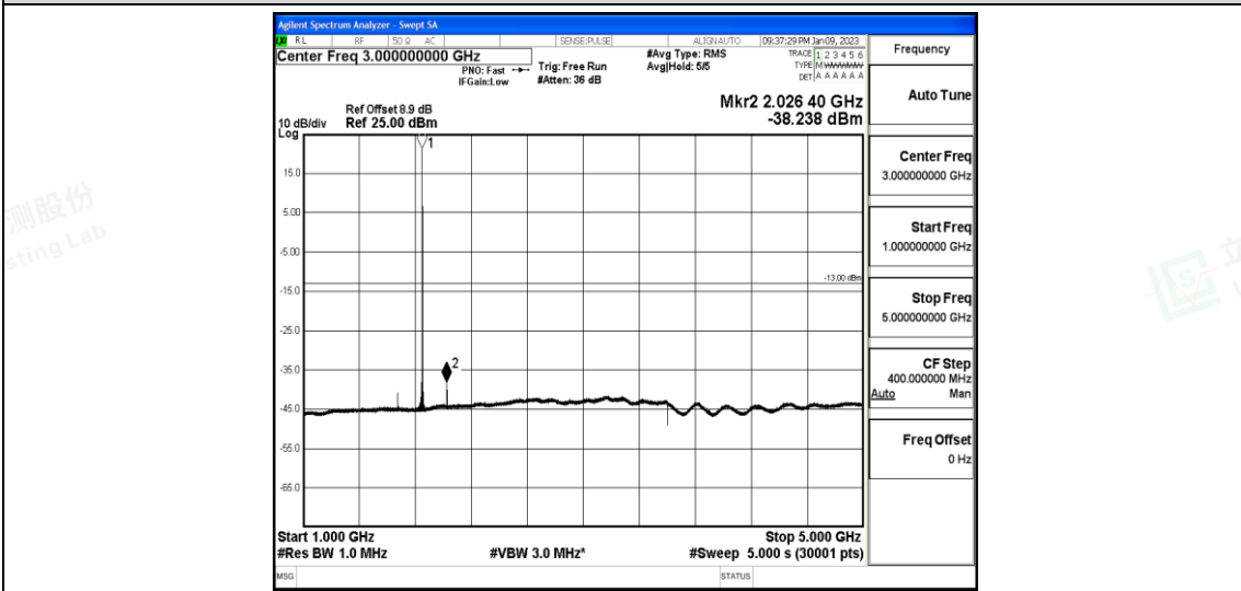
Band25-1.4MHz-QPSK-26047-1-0-Low-1000-5000--38.24-PASS
