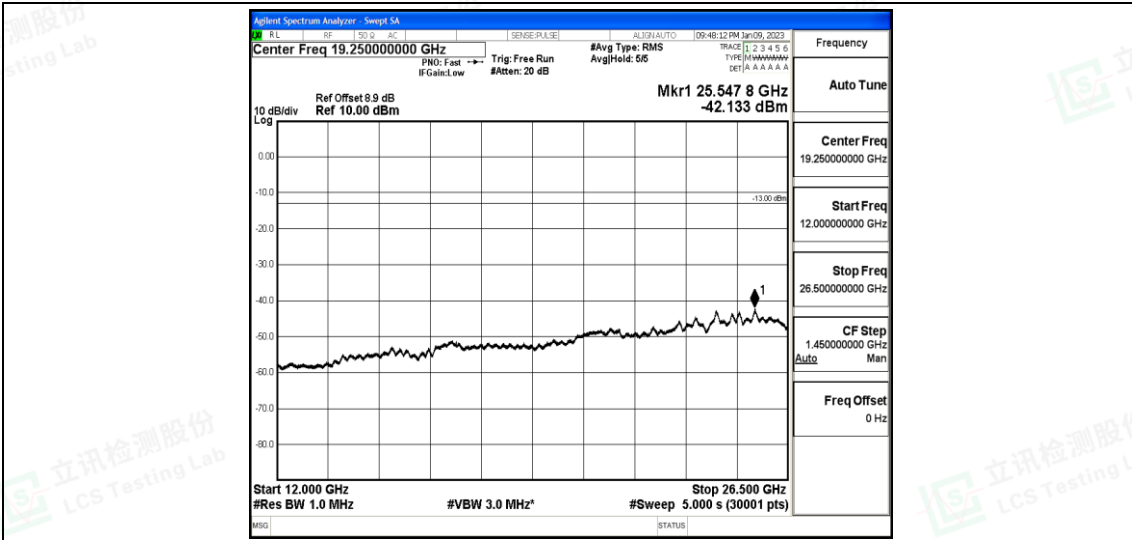
Band25-1.4MHz-16QAM-26683-1-0-High-12000-26500--42.13-PASS
