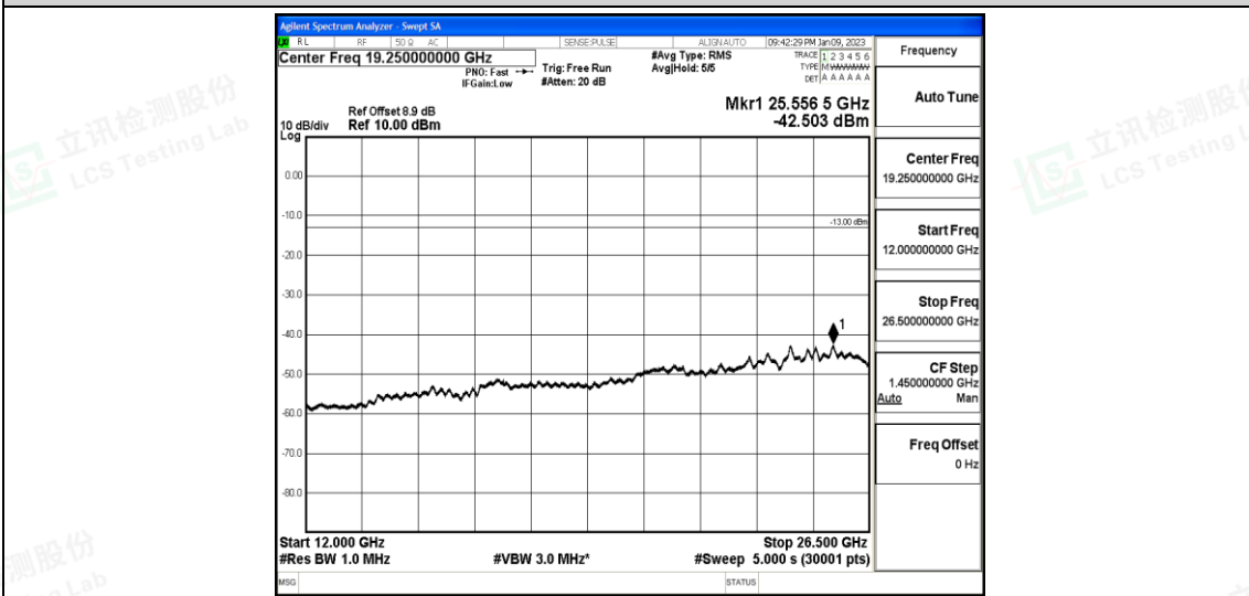
Band25-1.4MHz-QPSK-26365-1-0-Low-12000-26500--42.5-PASS
