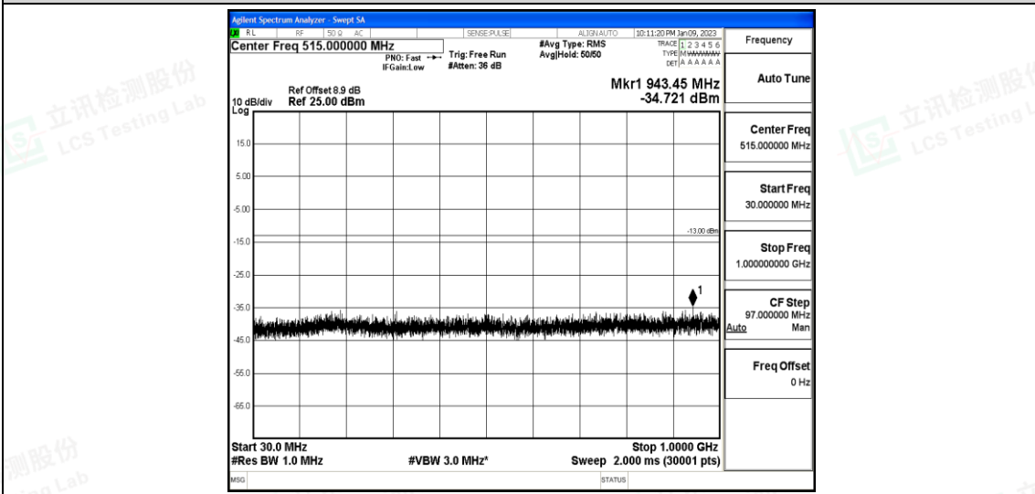
Band25-3MHz-16QAM-26365-1-0-Low-30-1000--34.72-PASS
