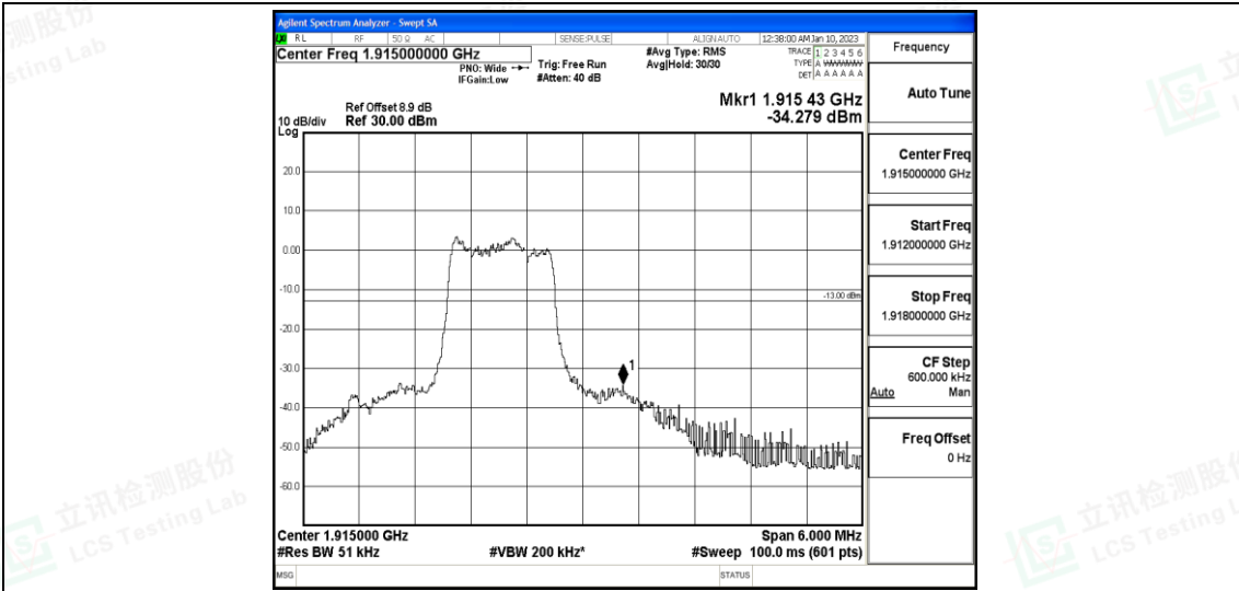
Band25-3MHz-QPSK-26675-6-0-High--34.28-PASS
