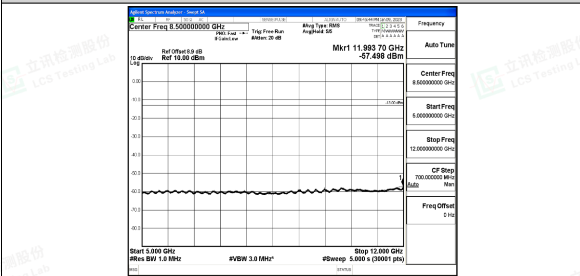
Band25-1.4MHz-QPSK-26683-1-0-High-5000-12000--57.5-PASS
