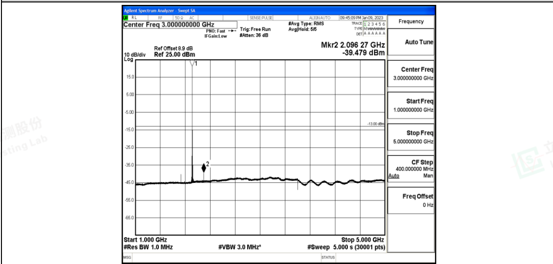
Band25-1.4MHz-QPSK-26683-1-0-High-1000-5000--39.48-PASS
