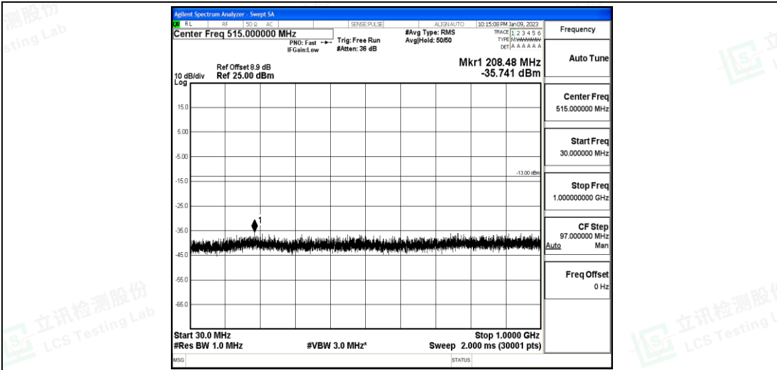
Band25-3MHz-16QAM-26675-1-0-High-30-1000--35.74-PASS
