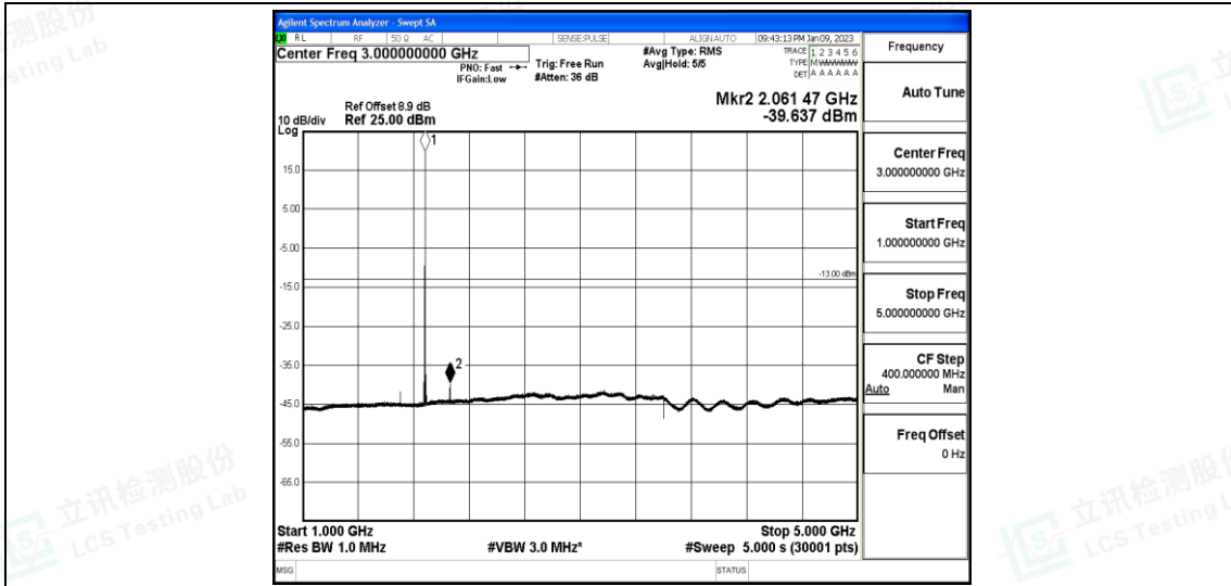
Band25-1.4MHz-16QAM-26365-1-0-Low-1000-5000--39.64-PASS
