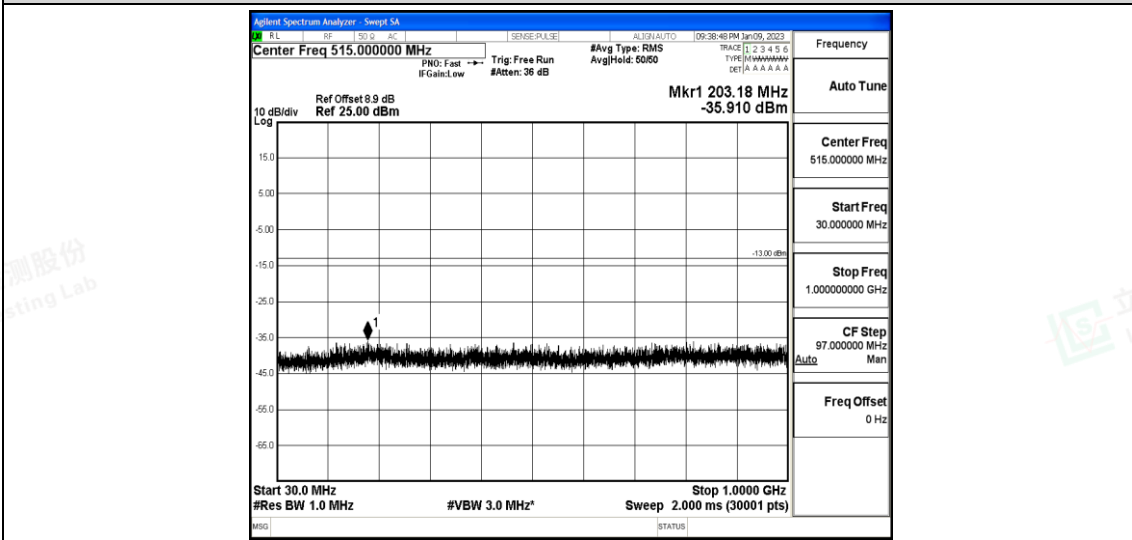
Band25-1.4MHz-16QAM-26047-1-0-Low-30-1000--35.91-PASS
