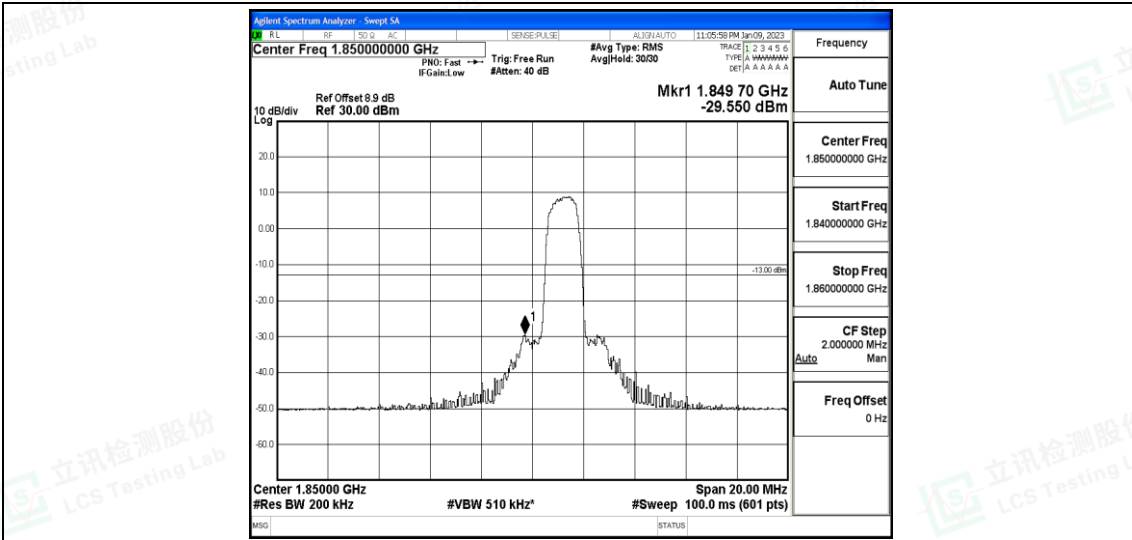
Band25-10MHz-16QAM-26090-6-0-Low--29.55-PASS
