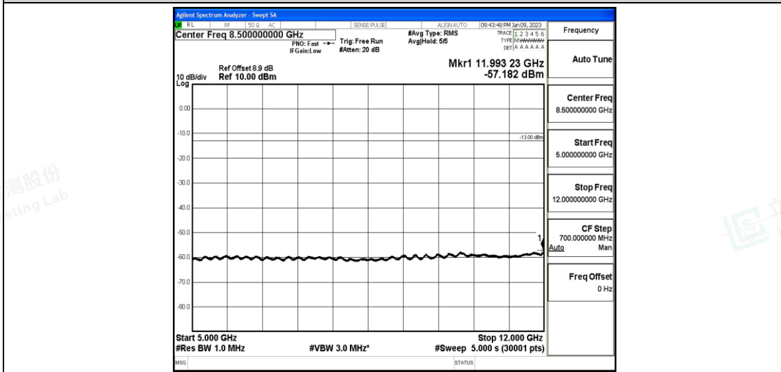
Band25-1.4MHz-16QAM-26365-1-0-Low-5000-12000--57.18-PASS
