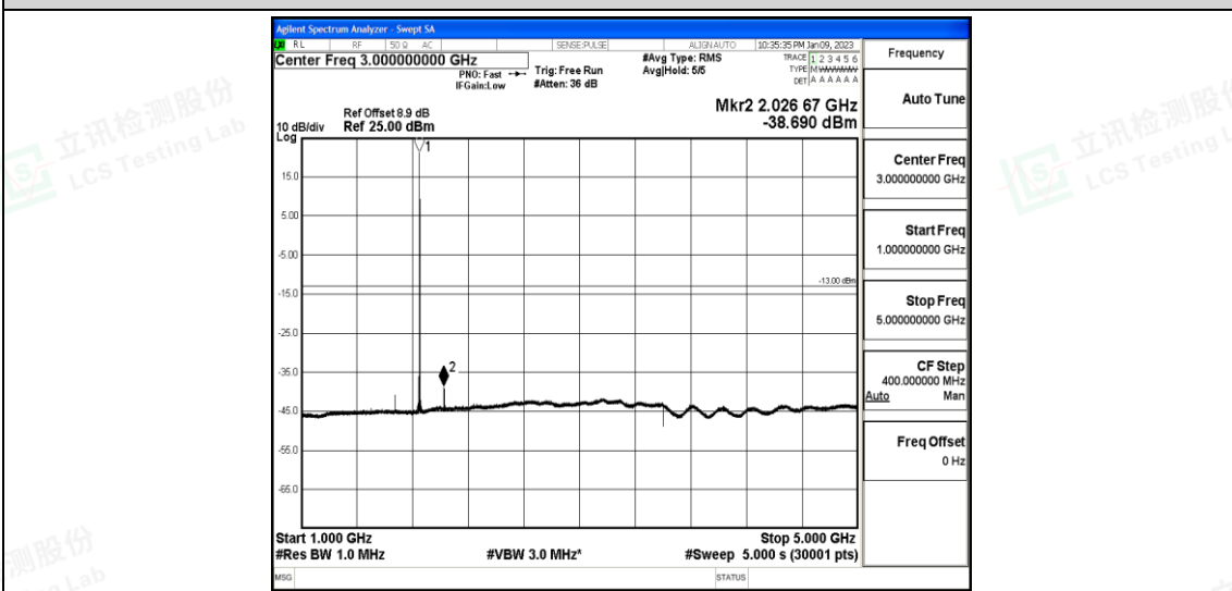
Band25-5MHz-QPSK-26065-1-0-Low-1000-5000--38.69-PASS
