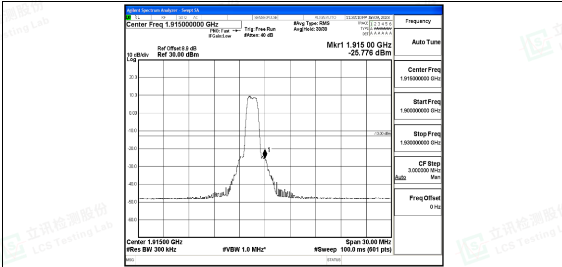
Band25-15MHz-QPSK-26615-6-0-High--25.78-PASS
